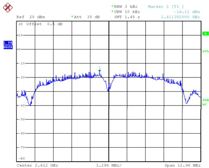
Power Spectral Density, 802.11b Low Channel
