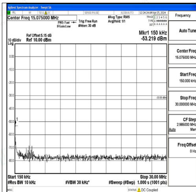
Band4_10MHz_QPSK_20000_1RB#0_0.15~30_0.15~30
