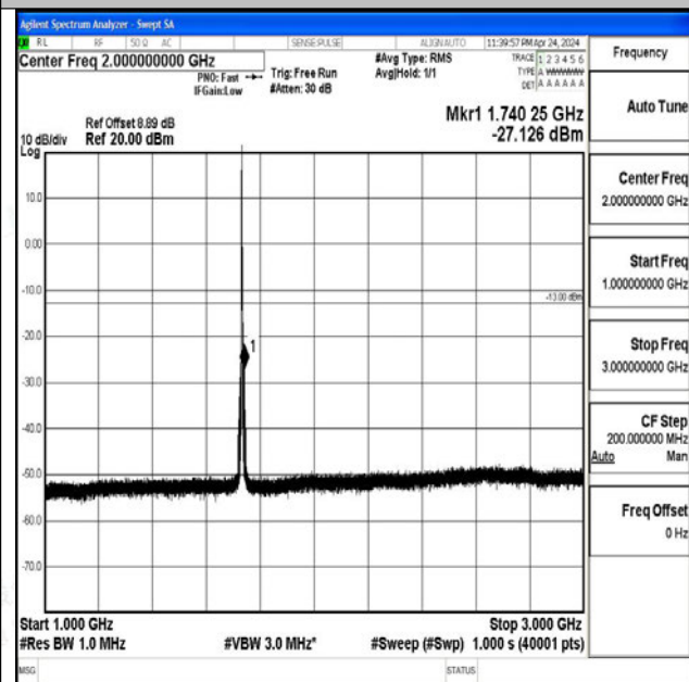
Band4_3MHz_QPSK_20175_1RB#0_1000~3000_1000~3000
