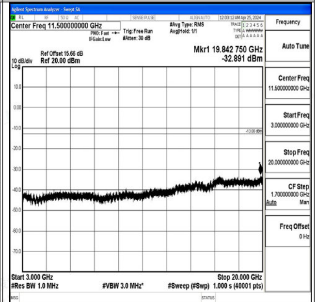
Band4_5MHz_QPSK_20175_1RB#0_3000~20000_3000~20000
