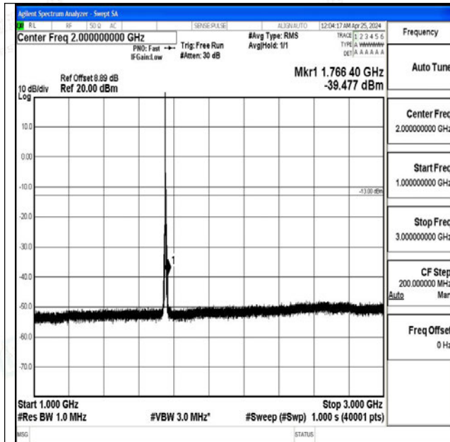
Band4_5MHz_QPSK_20375_1RB#0_1000~3000_1000~3000
