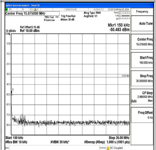
Band4_5MHz_16QAM_19975_1RB#0_0.15~30_0.15~30
