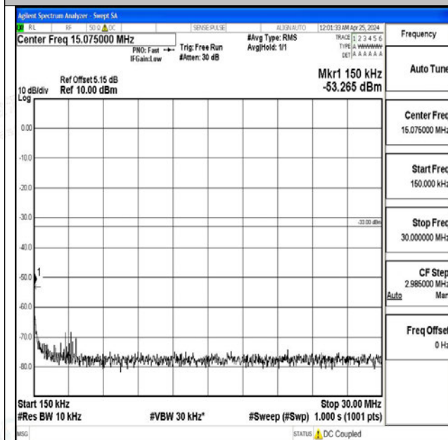
Band4_5MHz_QPSK_19975_1RB#0_0.15~30_0.15~30
