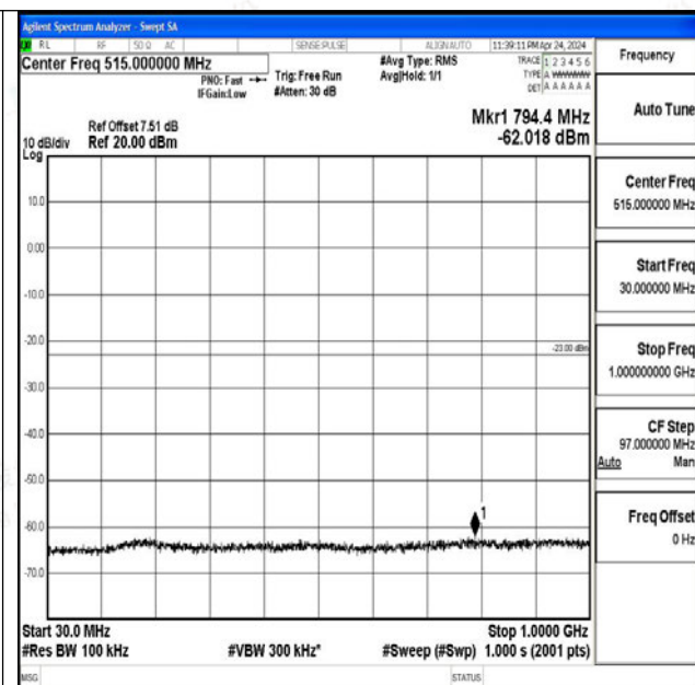
Band4_3MHz_16QAM_19965_1RB#0_30~1000_30~1000
