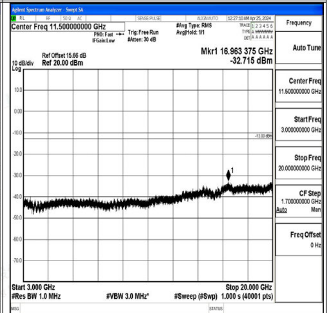
Band4_10MHz_QPSK_20350_1RB#0_3000~20000_3000 0~20000
