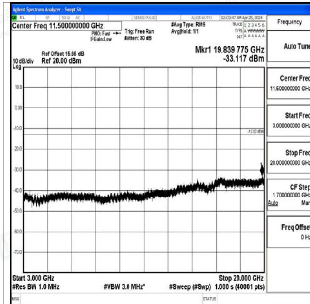
Band4_5MHz_16QAM_20175_1RB#0_3000~20000_300 0~20000
