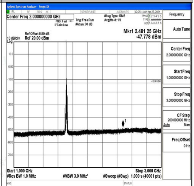
Band4_10MHz_16QAM_20000_1RB#0_1000~3000_100 0~3000
