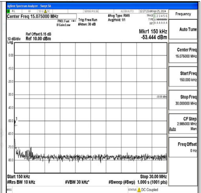
Band4_10MHz_16QAM_20350_1RB#0_0.15~30_0.15~3 0
