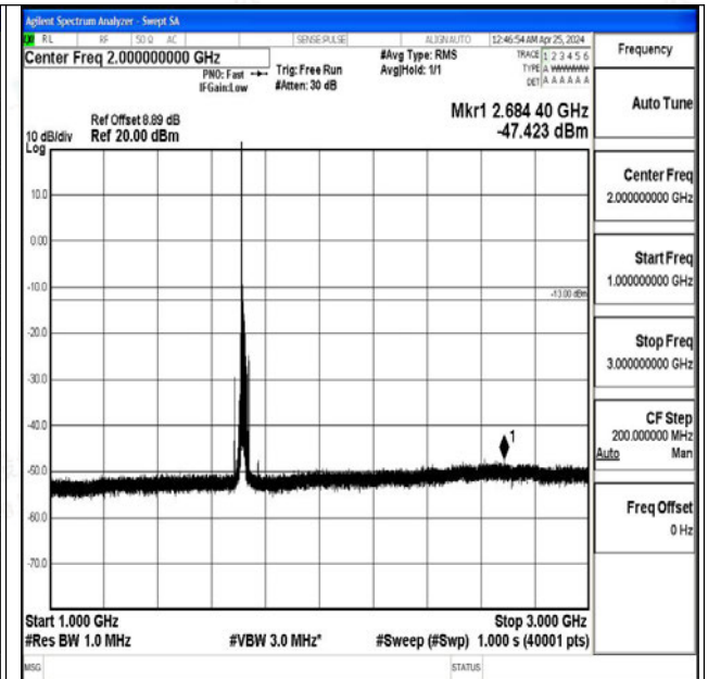
Band4_15MHz_16QAM_20025_1RB#0_1000~3000_1000~3000
