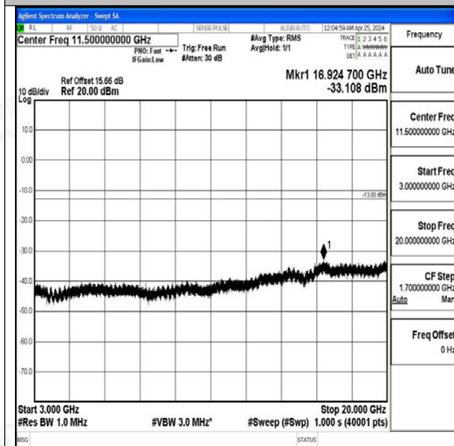
Band4_5MHz_16QAM_20375_1RB#0_3000~20000_300 0~20000
