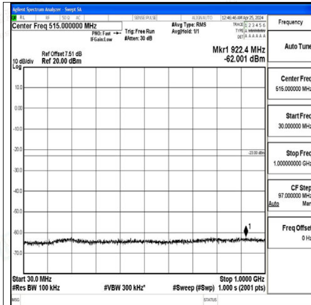
Band4_15MHz_16QAM_20025_1RB#0_30~1000_30~1000
