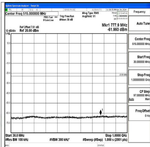
Band4_3MHz_QPSK_19965_1RB#0_30~1000_30~1000
