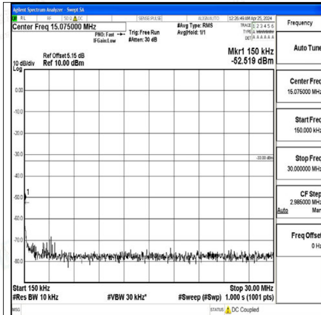
Band4_10MHz_QPSK_20350_1RB#0_0.15~30_0.15~30
