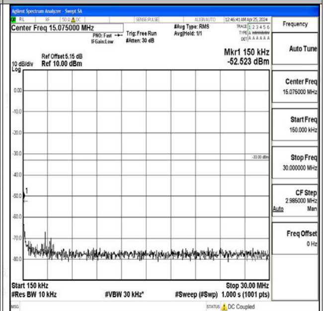
Band4_15MHz_16QAM_20025_1RB#0_0.15~30_0.15~3 0
