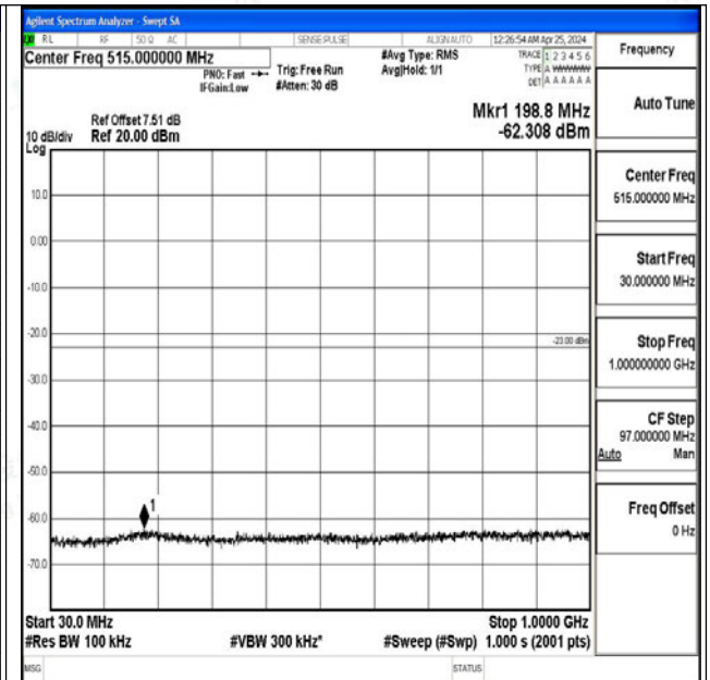
Band4_10MHz_QPSK_20350_1RB#0_30~1000_30~1000 0
