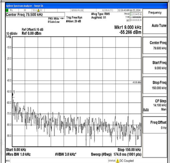
Band4_10MHz_QPSK_20350_1RB#0_0.009~0.15_0.009~0.15
