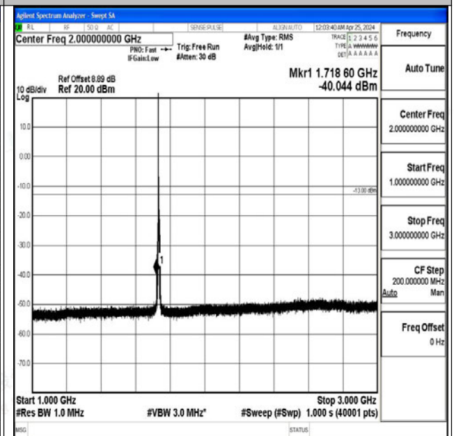
Band4_5MHz_16QAM_20175_1RB#0_1000~3000_1000 ~3000
