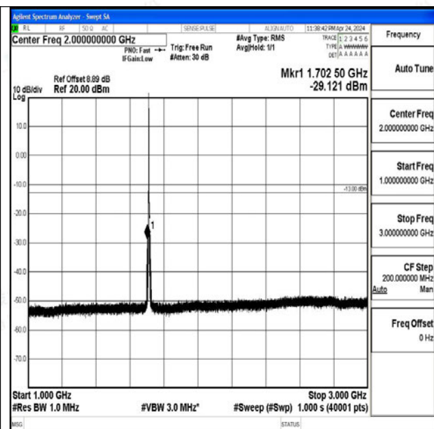
Band4_3MHz_QPSK_19965_1RB#0_1000~3000_1000~3000
