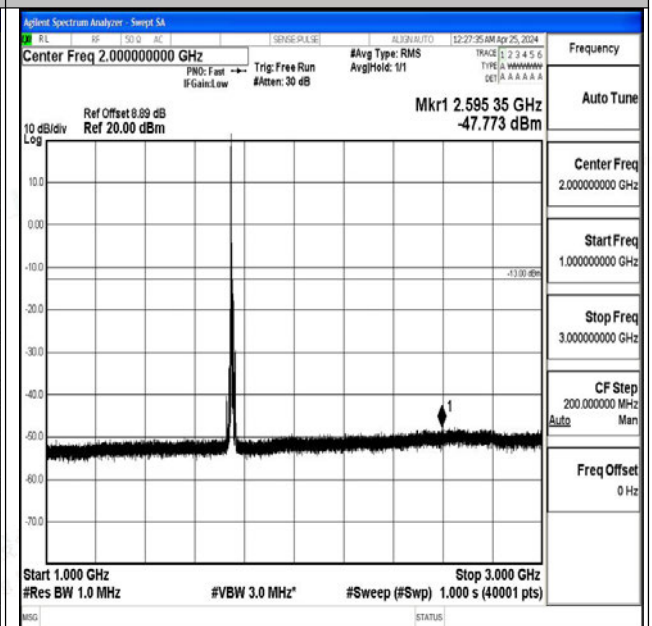
Band4_10MHz_16QAM_20350_1RB#0_1000~3000_100 0~3000
