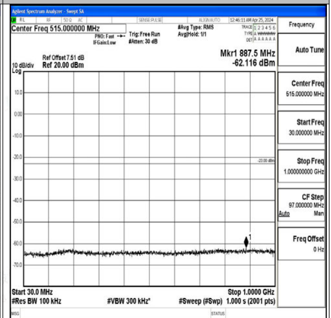
Band4_15MHz_QPSK_20025_1RB#0_30~1000_30~1000
