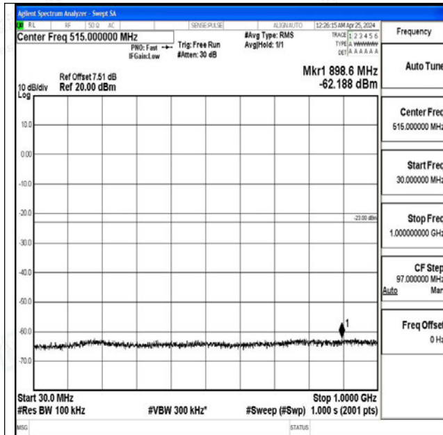
Band4_10MHz_16QAM_20175_1RB#0_30~1000_30~1000
