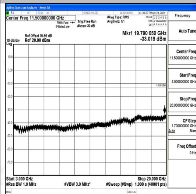
Band4_3MHz_16QAM_19965_1RB#0_3000~20000_3000~20000
