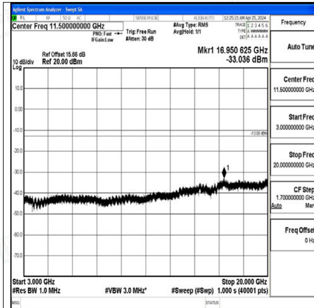
Band4_10MHz_16QAM_20000_1RB#0_3000~20000_3000~20000
