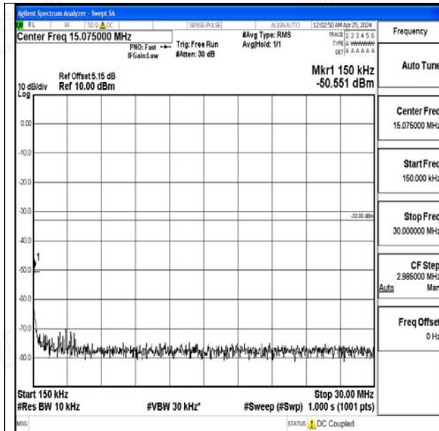
Band4_5MHz_QPSK_20175_1RB#0_0.15~30_0.15~30
