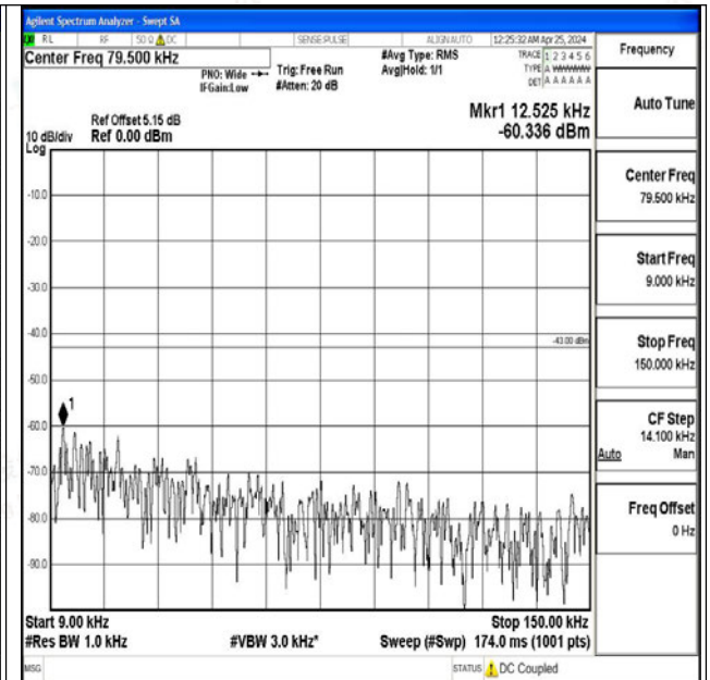
Band4_10MHz_QPSK_20175_1RB#0_0.009~0.15_0.009~0.15
