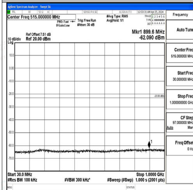
Band4_5MHz_16QAM_20175_1RB#0_30~1000_30~100 0
