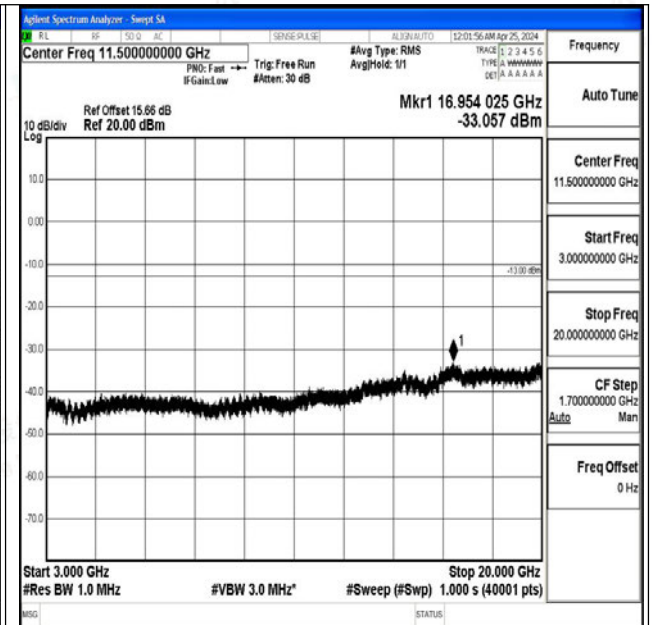
Band4_5MHz_QPSK_19975_1RB#0_3000~20000_3000~20000
