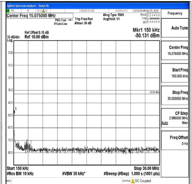
Band4_5MHz_16QAM_20175_1RB#0_0.15~30_0.15~30
