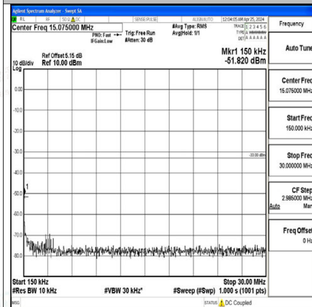
Band4_5MHz_QPSK_20375_1RB#0_0.15~30_0.15~30
