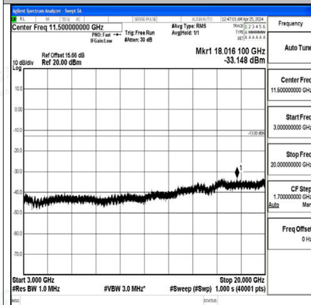
Band4_15MHz_16QAM_20025_1RB#0_3000~20000_3000~20000
