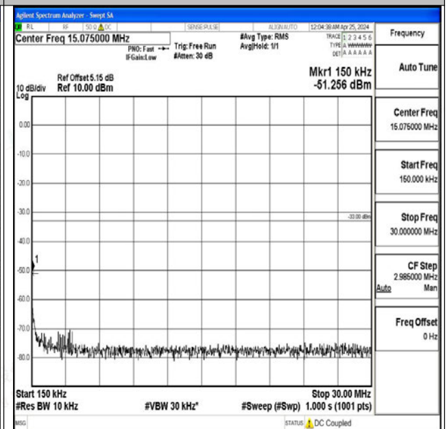
Band4_5MHz_16QAM_20375_1RB#0_0.15~30_0.15~30
