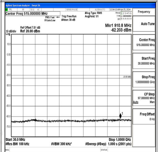
Band4_5MHz_QPSK_20375_1RB#0_30~1000_30~1000
