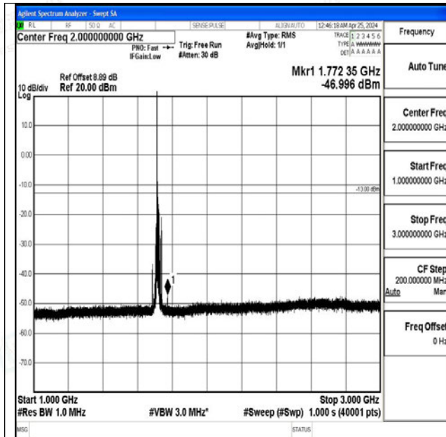
Band4_15MHz_QPSK_20025_1RB#0_1000~3000_1000 ~3000
