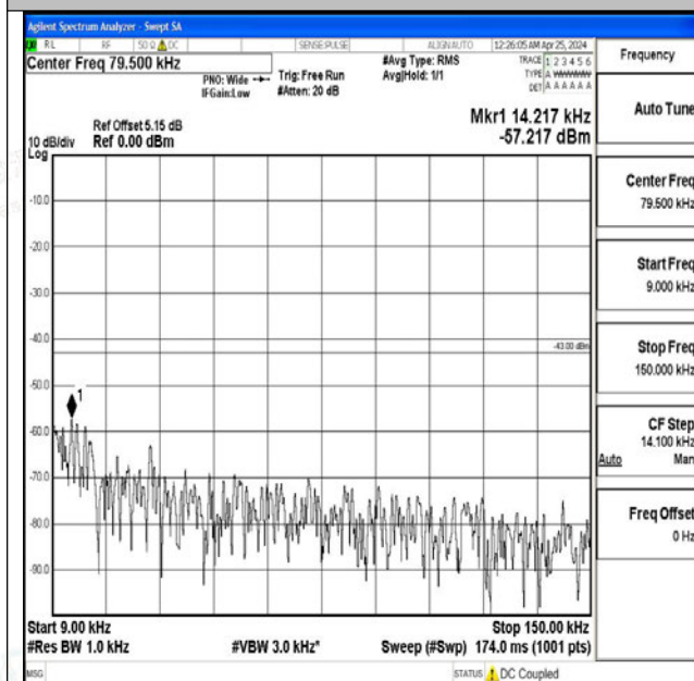
Band4_10MHz_16QAM_20175_1RB#0_0.009~0.15_0.0 09~0.15
