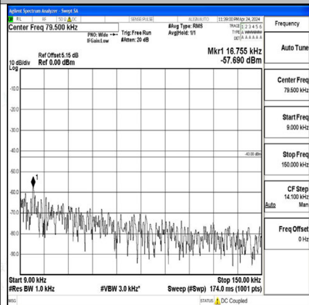
Band4_3MHz_16QAM_19965_1RB#0_0.009~0.15_0.009~0.15
