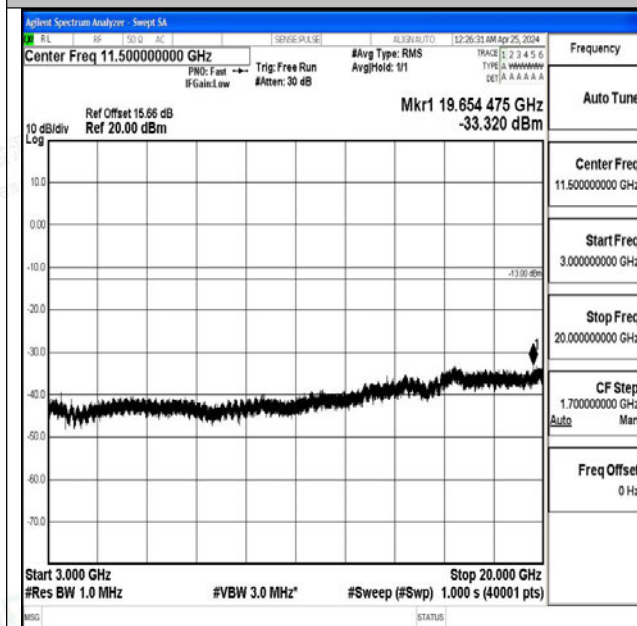
Band4_10MHz_16QAM_20175_1RB#0_3000~20000_3000~20000
