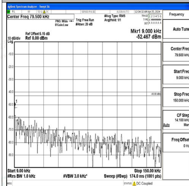
Band4_5MHz_16QAM_20375_1RB#0_0.009~0.15_0.009~0.15
