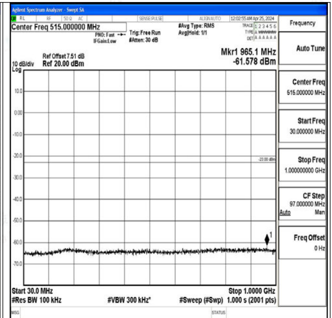
Band4_5MHz_QPSK_20175_1RB#0_30~1000_30~1000
