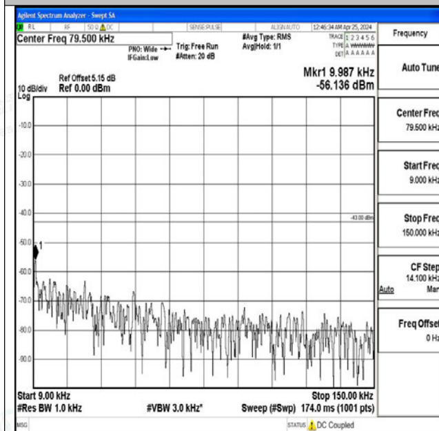
Band4_15MHz_16QAM_20025_1RB#0_0.009~0.15_0.0 09~0.15
