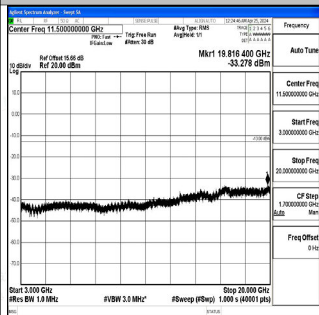
Band4_10MHz_QPSK_20000_1RB#0_3000~20000_3000 0~20000
