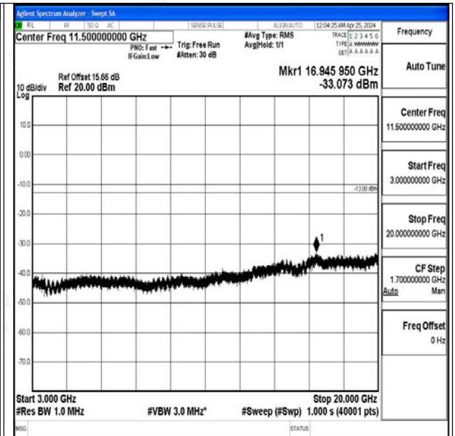
Band4_5MHz_QPSK_20375_1RB#0_3000~20000_3000~20000
