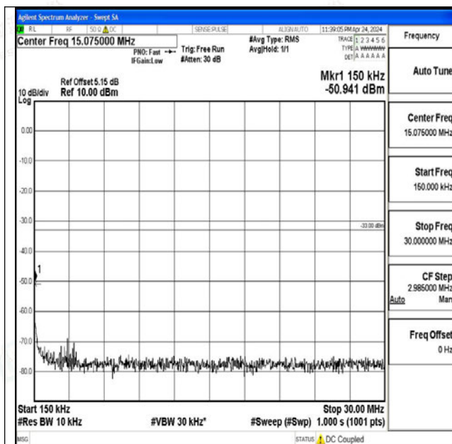
Band4_3MHz_16QAM_19965_1RB#0_0.15~30_0.15~30
