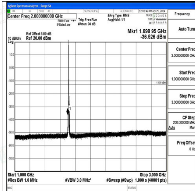
Band4_5MHz_QPSK_19975_1RB#0_1000~3000_1000~3000
