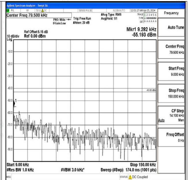
Band4_5MHz_QPSK_19975_1RB#0_0.009~0.15_0.009~ 0.15
