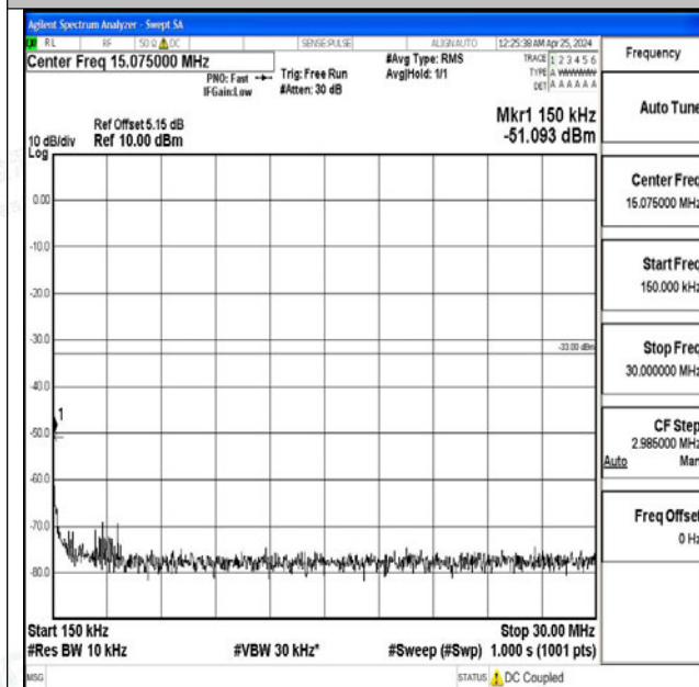
Band4_10MHz_16QAM_20000_1RB#0_3000~20000_3000~20000
