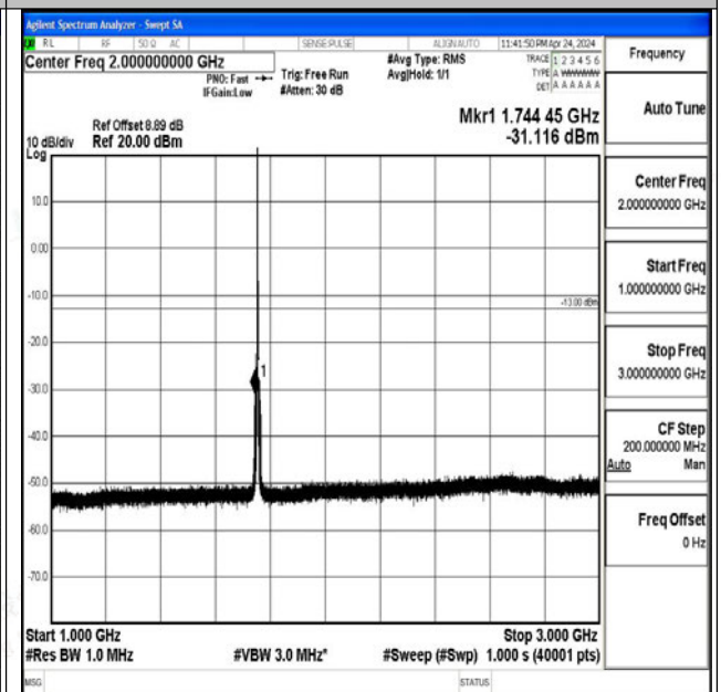
Band4_3MHz_16QAM_20385_1RB#0_1000~3000_1000 ~3000
