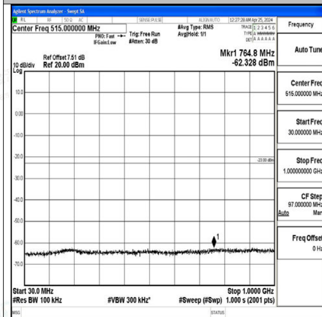
Band4_10MHz_16QAM_20350_1RB#0_30~1000_30~10 00
