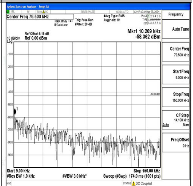
Band4_15MHz_QPSK_20175_1RB#0_0.009~0.15_0.009~0.15
