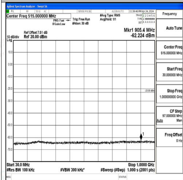
Band4_3MHz_QPSK_20175_1RB#0_30~1000_30~1000
