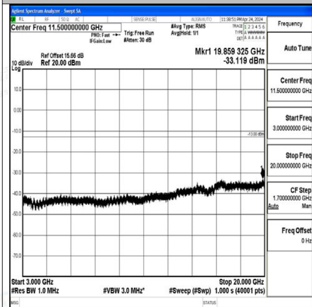
Band4_3MHz_QPSK_19965_1RB#0_3000~20000_3000~20000
