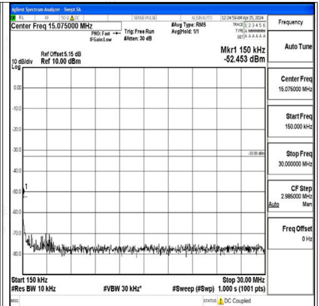
Band4_10MHz_16QAM_20000_1RB#0_0.15~30_0.15~3 0
