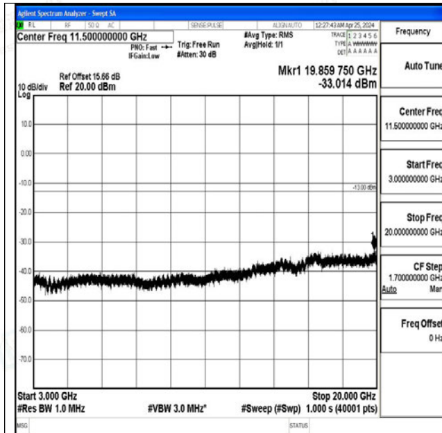
Band4_10MHz_16QAM_20350_1RB#0_3000~20000_3000~20000
