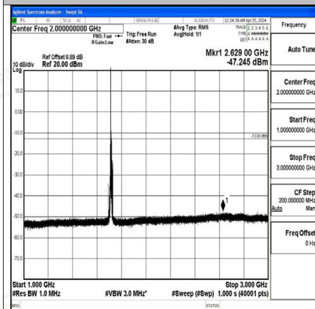
Band4_10MHz_QPSK_20000_1RB#0_1000~3000_1000 ~3000
