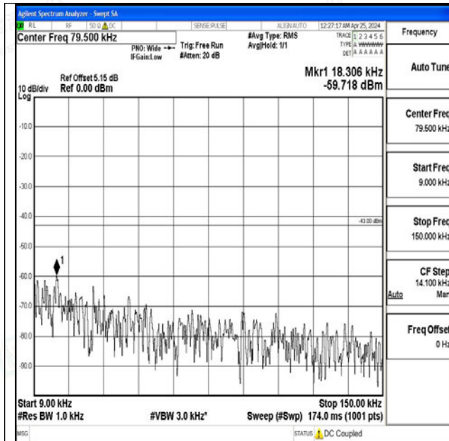
Band4_10MHz_16QAM_20350_1RB#0_0.009~0.15_0.0 09~0.15
