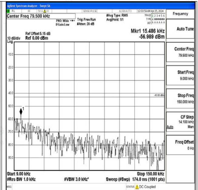
Band4_5MHz_QPSK_20375_1RB#0_0.009~0.15_0.009~ 0.15
