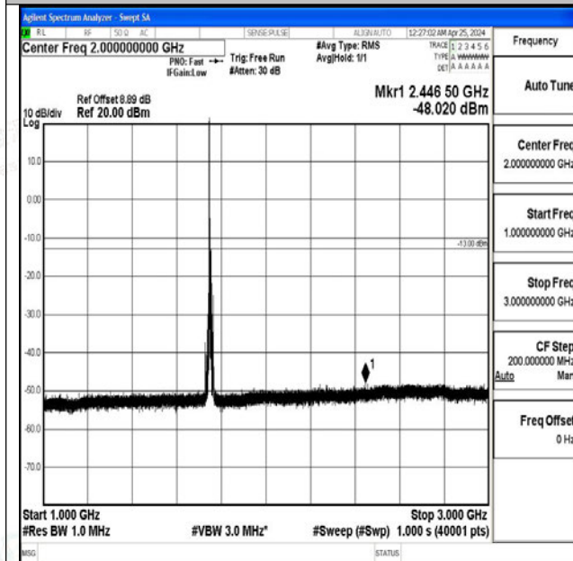
Band4_10MHz_QPSK_20350_1RB#0_1000~3000_1000 ~3000
