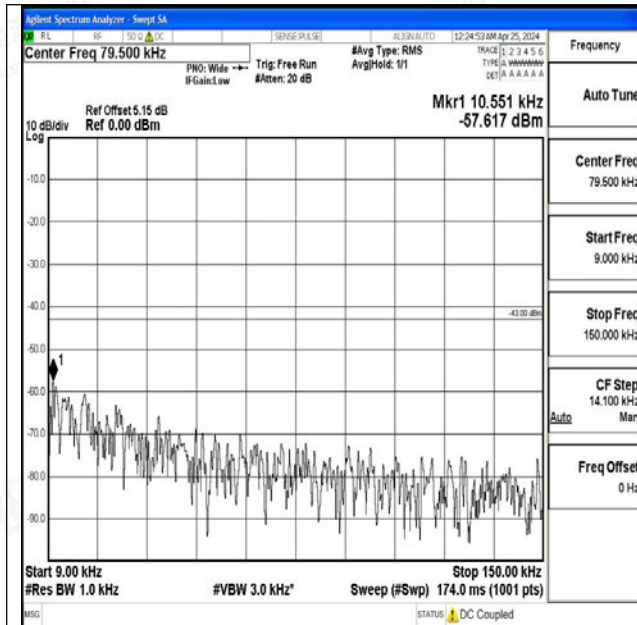
Band4_10MHz_16QAM_20000_1RB#0_0.009~0.15_0.0 09~0.15
