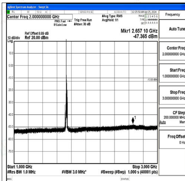
Band4_10MHz_QPSK_20175_1RB#0_1000~3000_1000 ~3000
