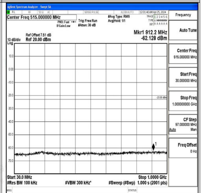
Band4_5MHz_QPSK_19975_1RB#0_30~1000_30~1000
