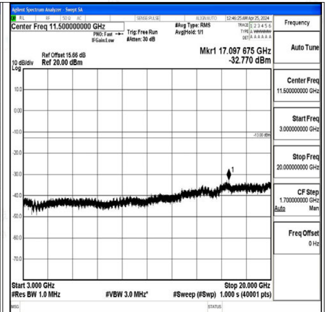
Band4_15MHz_QPSK_20025_1RB#0_3000~20000_300 0~20000
