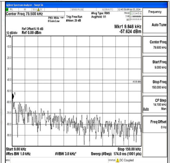
Band4_15MHz_QPSK_20025_1RB#0_0.009~0.15_0.009~0.15
