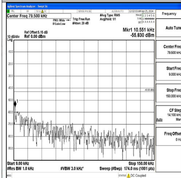
Band4_5MHz_16QAM_19975_1RB#0_0.009~0.15_0.009~0.15
