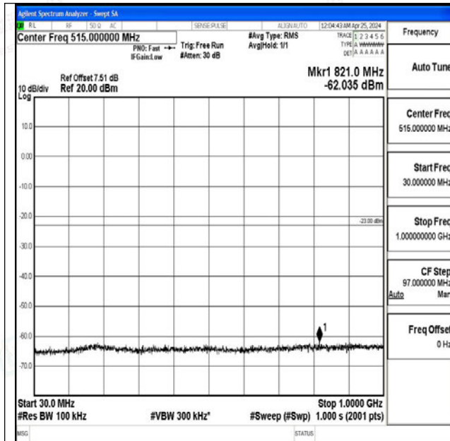
Band4_5MHz_16QAM_20375_1RB#0_30~1000_30~100 0
