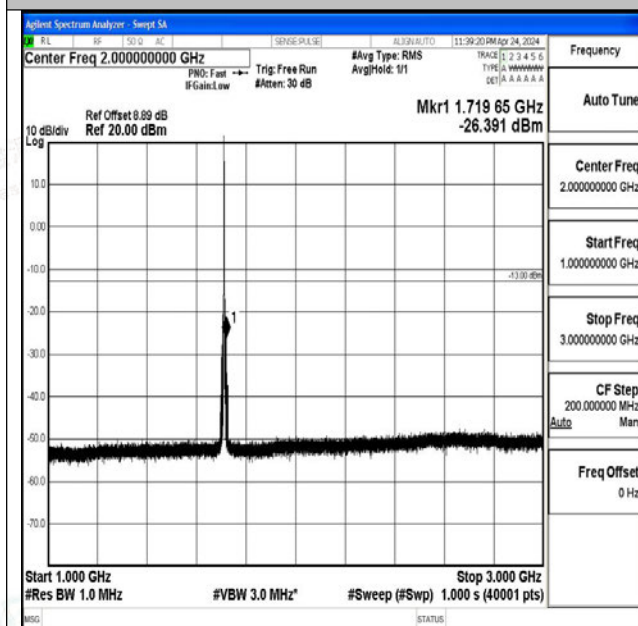
Band4_3MHz_16QAM_19965_1RB#0_1000~3000_1000~3000
