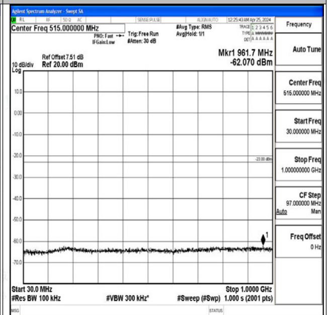
Band4_10MHz_QPSK_20175_1RB#0_30~1000_30~1000
