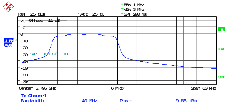
MAXIMUM CONDUCTED POWER ANT1_11ax40CH159_106RU4 Date: 4.AUG.2023 19:15:34
