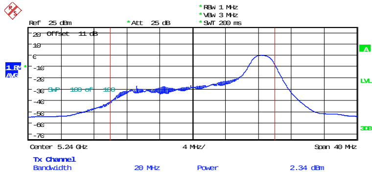
MAXIMUM CONDUCTED POWER ANT1_11ax20CH48_26RU1 Date: 4.AUG.2023 18:24:12
