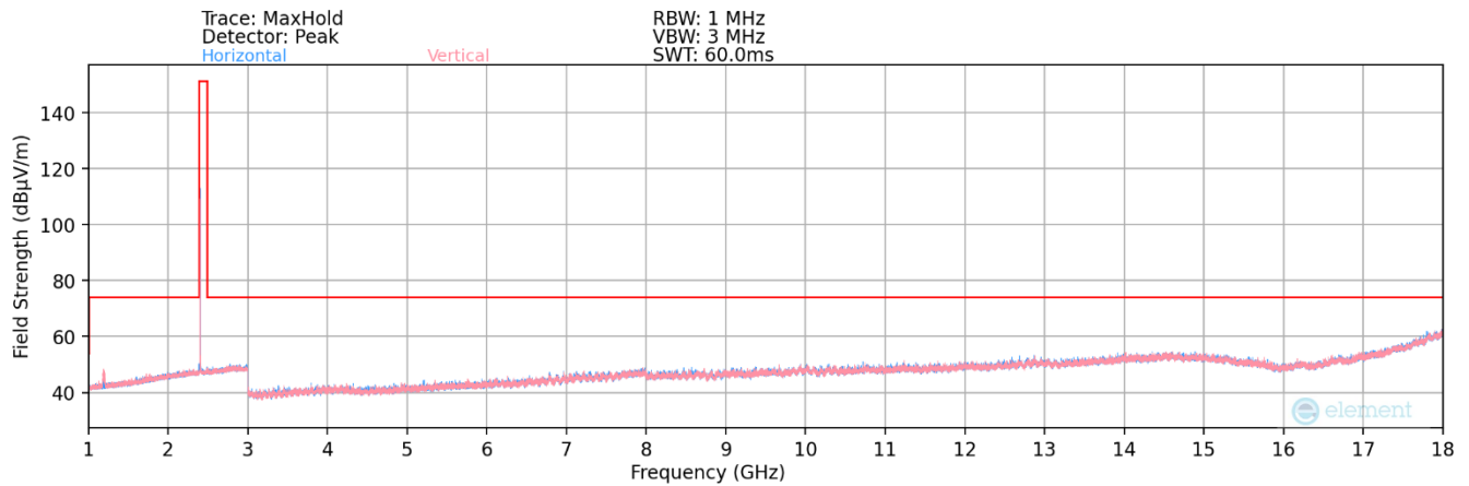
Plot 7-84. Radiated Spurious Plot above 1GHz (BT– Ch. 0) – Ant1
