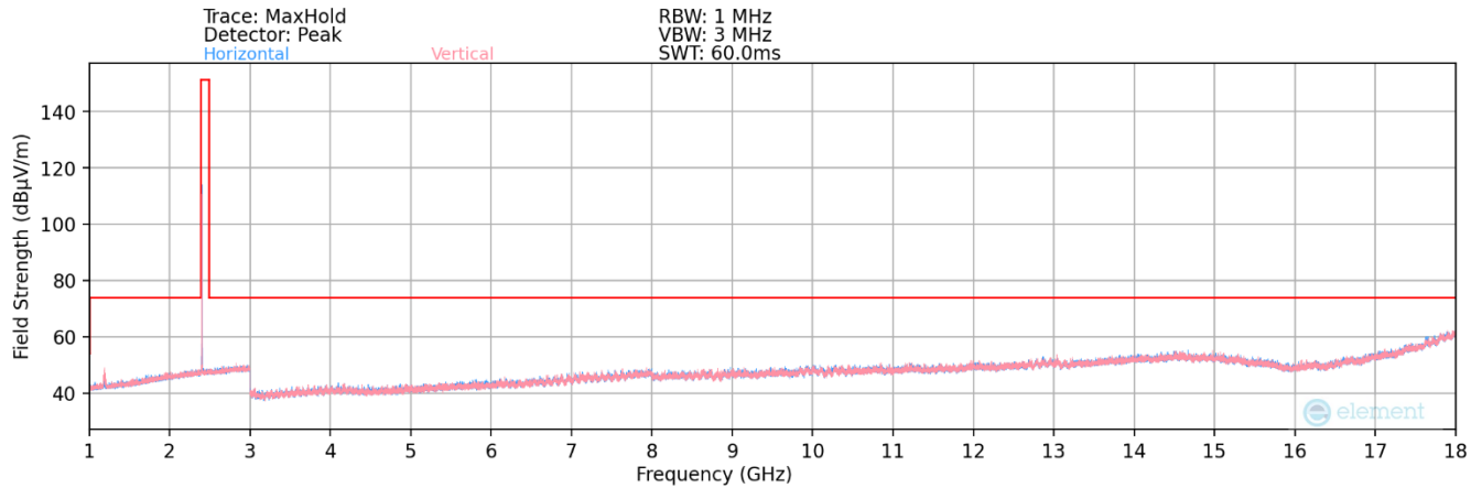
Plot 7-88. Radiated Spurious Plot above 1GHz (BT– Ch. 0) – Ant2
