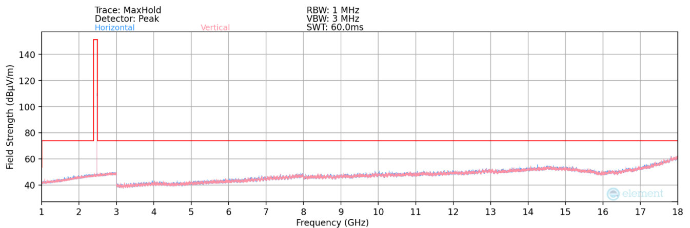
Plot 7-86. Radiated Spurious Plot above 1GHz (BT– Ch. 78) – Ant1
