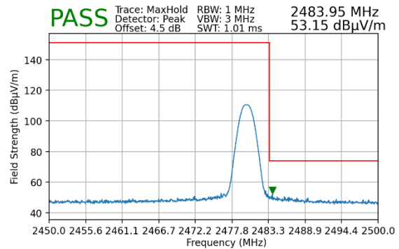
Plot 7-93. Radiated Restricted Upper Band Edge Measurement (Peak) – Ant1
