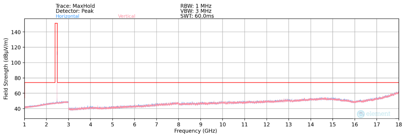
Plot 7-90. Radiated Spurious Plot above 1GHz (BT– Ch. 78) – Ant2
