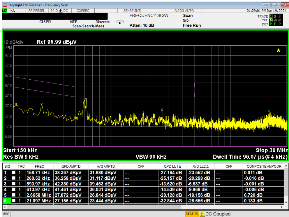
Plot 7-98. Line-Conducted Test Plot (L1)
