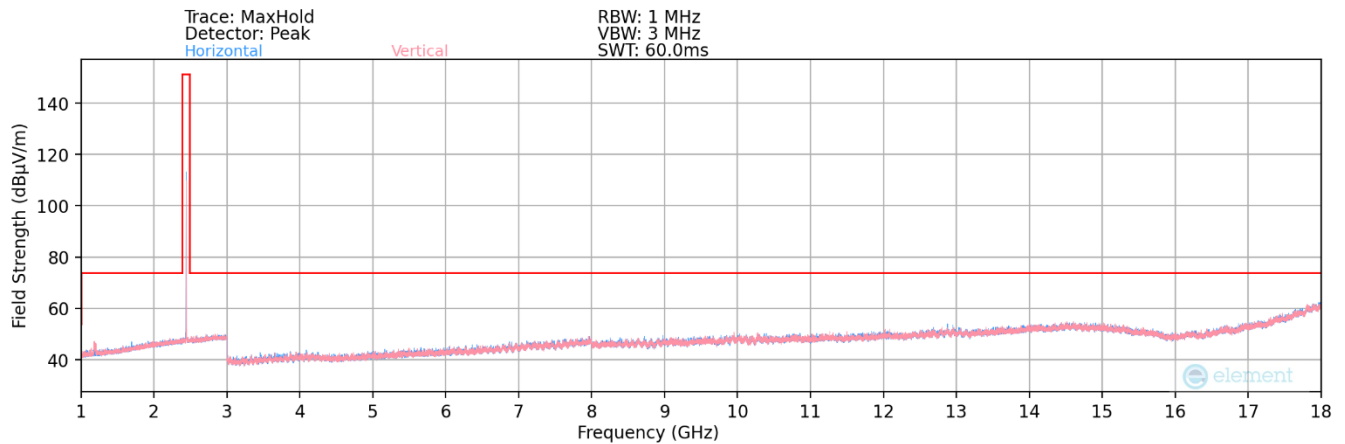
Plot 7-89. Radiated Spurious Plot above 1GHz (BT– Ch. 39) – Ant2
