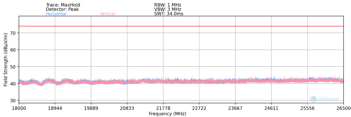
Plot 7-91. Radiated Spurious Plot above 18GHz – Ant2
