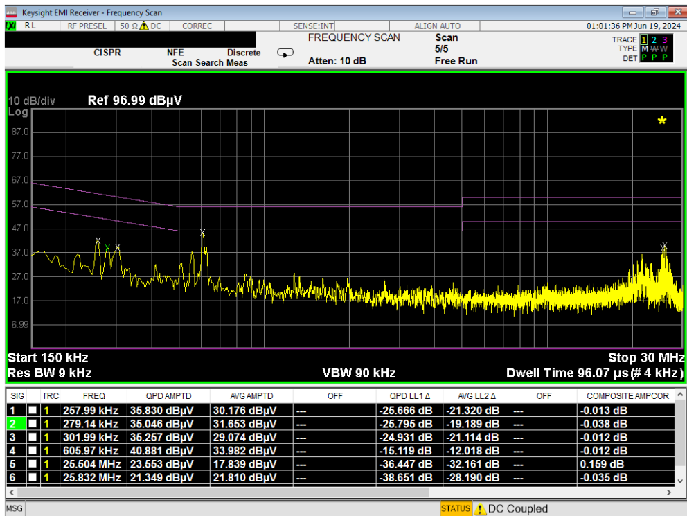
Plot 7-99. Line-Conducted Test Plot (N)
