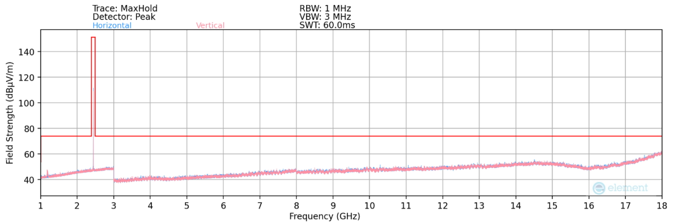
Plot 7-85. Radiated Spurious Plot above 1GHz (BT– Ch. 39) – Ant1
