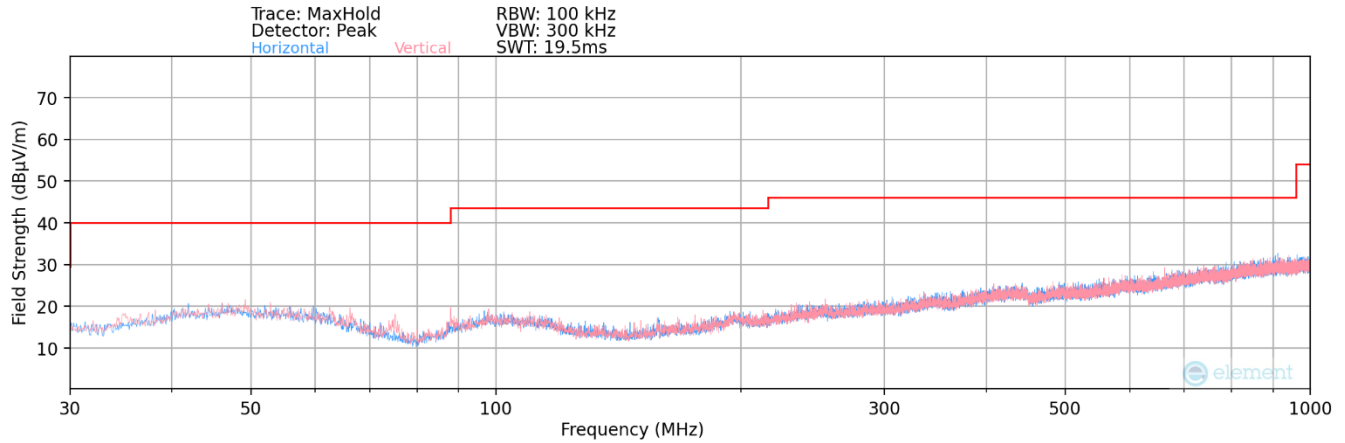
Plot 7-96. Radiated Spurious Plot below 1GHz – Ant1
