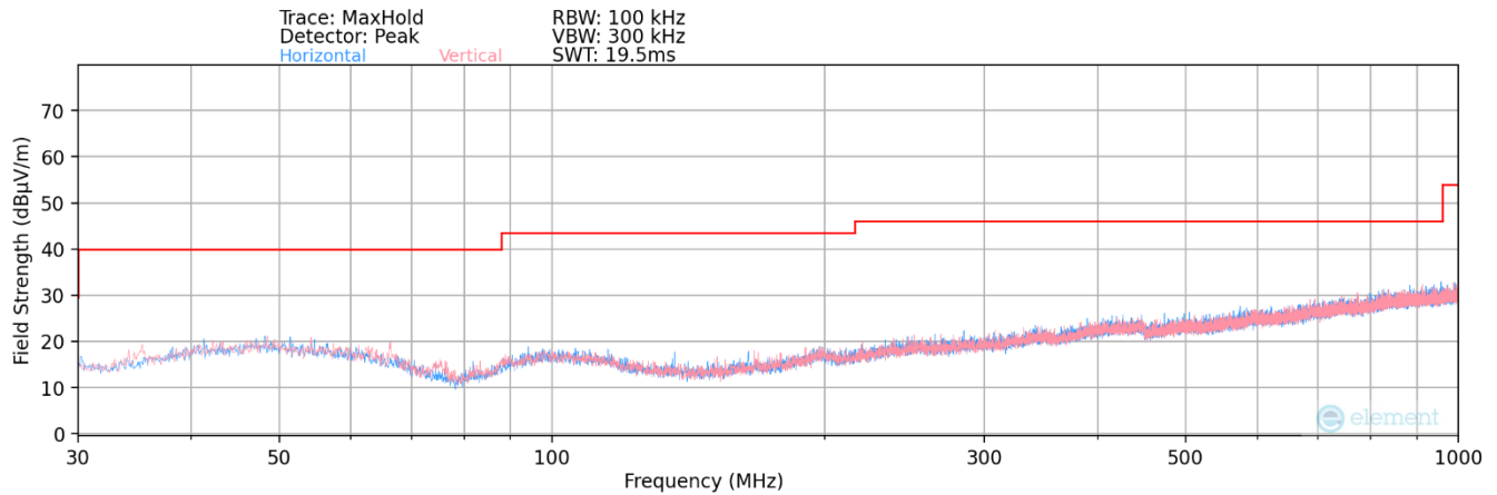
Plot 7-97. Radiated Spurious Plot below 1GHz – Ant2
