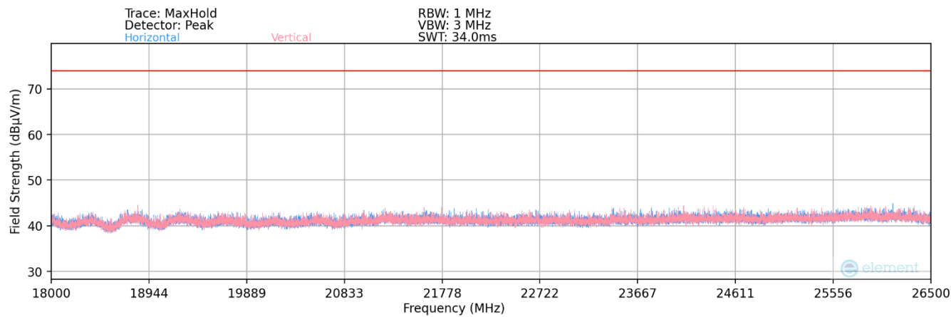
Plot 7-87. Radiated Spurious Plot above 18GHz – Ant1
