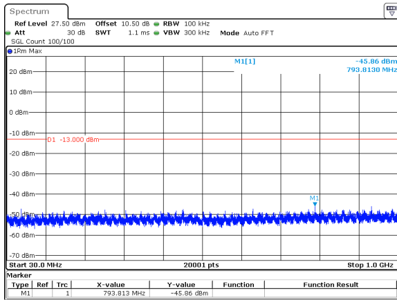
25MHz_30kHz_3712.5MHz_DFT-s-OFDM QPSK_RB1@64&amp;-45.86 dBm
