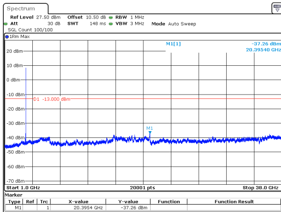
50MHz_30kHz_3775MHz_DFT-s-OFDM QPSK_RB1@132&amp;-37.26 dBm
