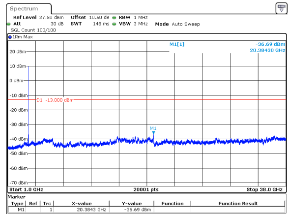
50MHz_30kHz_3725MHz_DFT-s-OFDM QPSK_RB1@132&amp;-36.69 dBm
