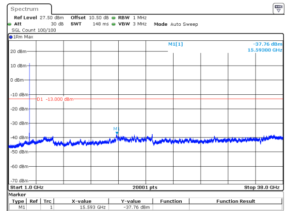
25MHz_15kHz_3787.5MHz_DFT-s-OFDM QPSK_RB1@132&amp;-37.76 dBm
