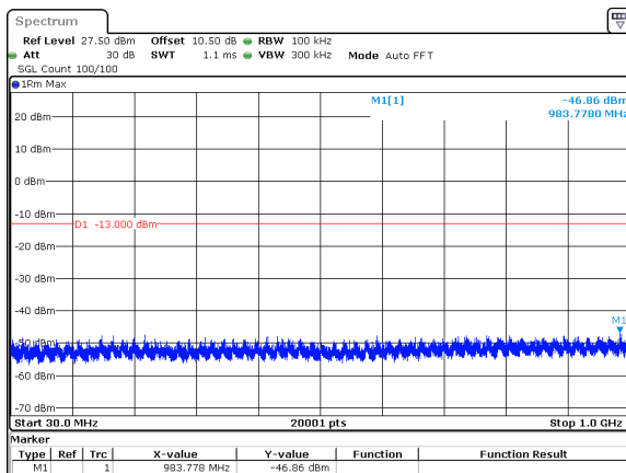
60MHz_30kHz_3730MHz_DFT-s-OFDM QPSK_RB162@0&amp;-46.86 dBm
