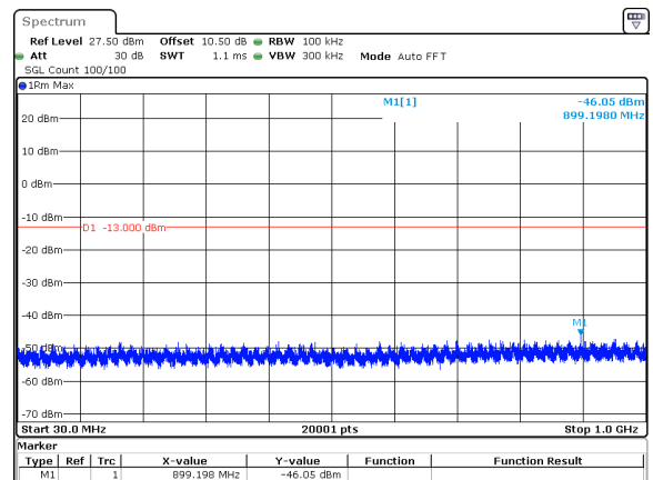
50MHz_30kHz_3725MHz_DFT-s-OFDM QPSK_RB128@0&amp;-46.05 dBm
