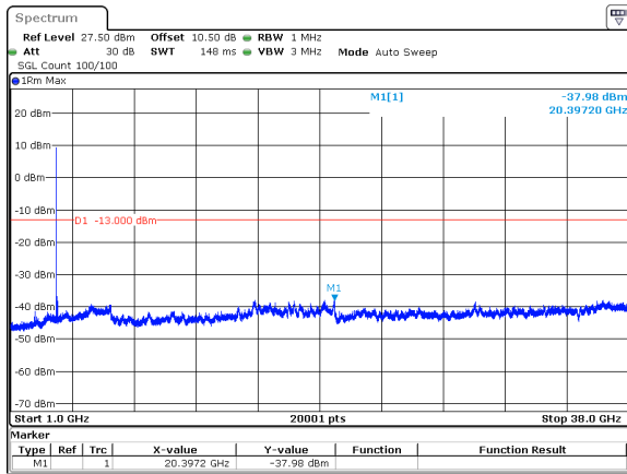
30MHz_15kHz_3750MHz_DFT-s-OFDM QPSK_RB1@0&amp;-37.98 dBm
