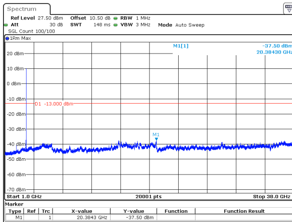
30MHz_30kHz_3715MHz_DFT-s-OFDM QPSK_RB1@77&amp;-37.50 dBm
