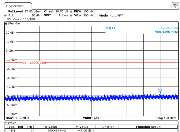
30MHz_15kHz_3715MHz_DFT-s-OFDM QPSK_RB160@0&amp;-47.06 dBm
