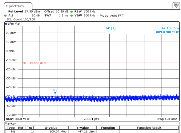
25MHz_15kHz_3750MHz_DFT-s-OFDM QPSK_RB128@0&amp;-47.18 dBm
