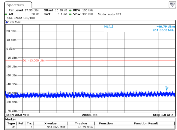
30MHz_15kHz_3750MHz_DFT-s-OFDM QPSK_RB1@0&amp;-46.79 dBm
