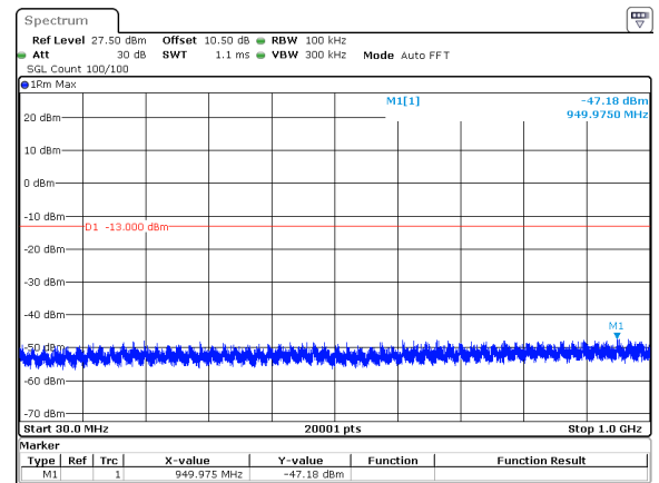
25MHz_30kHz_3787.5MHz_DFT-s-OFDM QPSK_RB1@64&amp;-47.18 dBm
