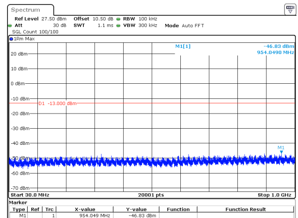
50MHz_15kHz_3775MHz_DFT-s-OFDM QPSK_RB270@0&amp;-46.83 dBm
