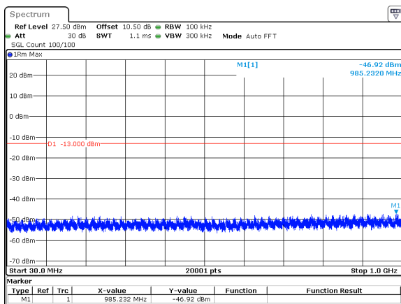
25MHz_15kHz_3787.5MHz_DFT-s-OFDM QPSK_RB128@0&amp;-46.92 dBm
