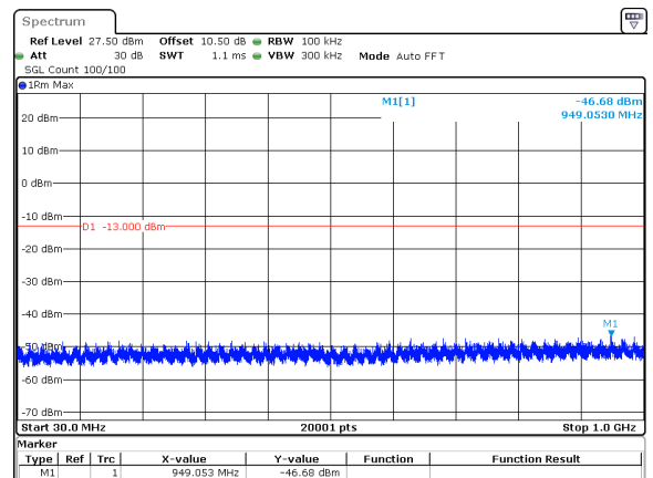
40MHz_30kHz_3750MHz_DFT-s-OFDM QPSK_RB100@0&amp;-46.68 dBm
