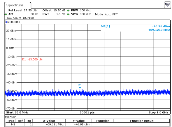
50MHz_15kHz_3750MHz_DFT-s-OFDM QPSK_RB1@269&amp;-46.95 dBm
