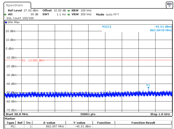
50MHz_30kHz_3775MHz_DFT-s-OFDM QPSK_RB1@132&amp;-45.51 dBm
