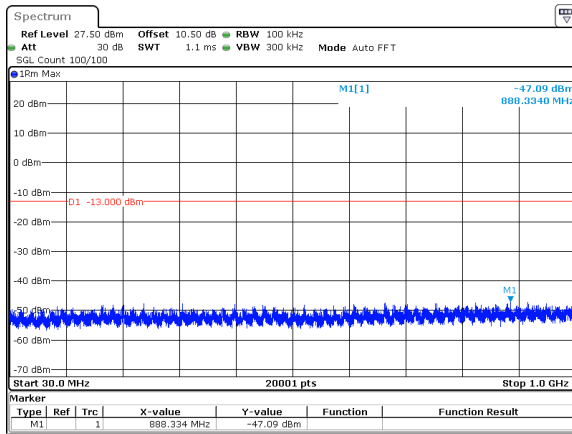
30MHz_15kHz_3715MHz_DFT-s-OFDM QPSK_RB1@0&amp;-47.09 dBm
