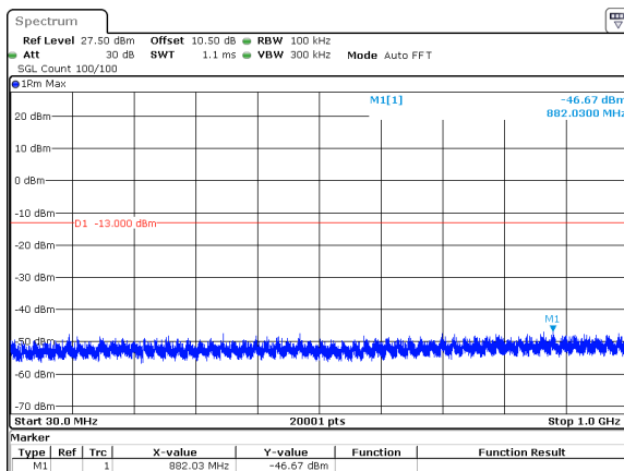
15MHz_30kHz_3750MHz_DFT-s-OFDM QPSK_RB36@0&amp;-46.67 dBm
