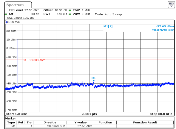
30MHz_30kHz_3715MHz_DFT-s-OFDM QPSK_RB1@0&amp;-37.63 dBm
