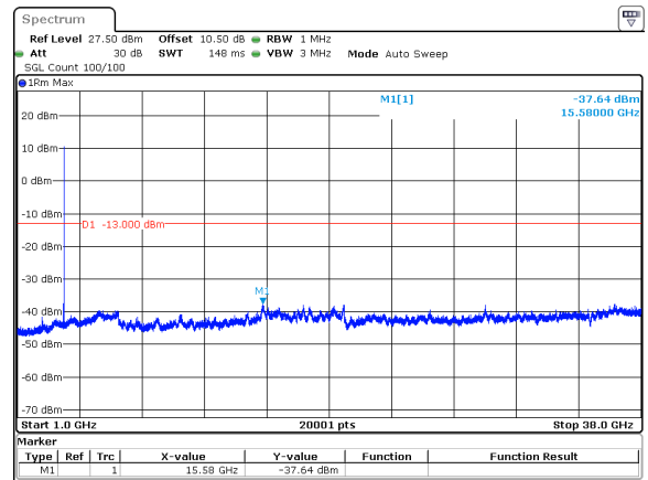
25MHz_15kHz_3750MHz_DFT-s-OFDM QPSK_RB1@132&amp;-37.64 dBm
