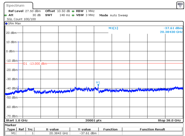
60MHz_30kHz_3750MHz_DFT-s-OFDM QPSK_RB1@161&amp;-37.61 dBm
