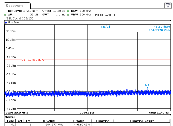
30MHz_15kHz_3785MHz_DFT-s-OFDM QPSK_RB160@0&amp;-46.62 dBm
