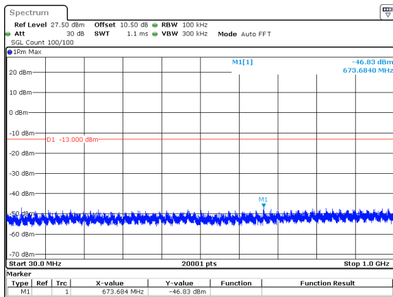
25MHz_15kHz_3787.5MHz_DFT-s-OFDM QPSK_RB1@132&amp;-46.83 dBm
