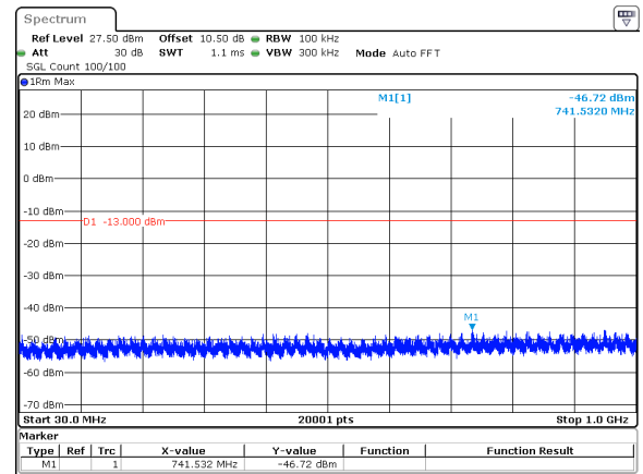
15MHz_15kHz_3750MHz_DFT-s-OFDM QPSK_RB1@78&amp;-46.72 dBm
