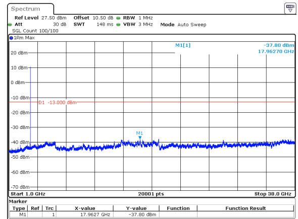
15MHz_30kHz_3750MHz_DFT-s-OFDM QPSK_RB1@37&amp;-37.80 dBm
