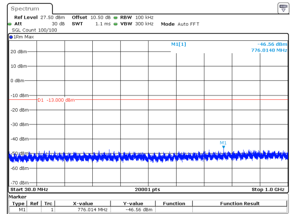
50MHz_15kHz_3775MHz_DFT-s-OFDM QPSK_RB1@269&amp;-46.56 dBm
