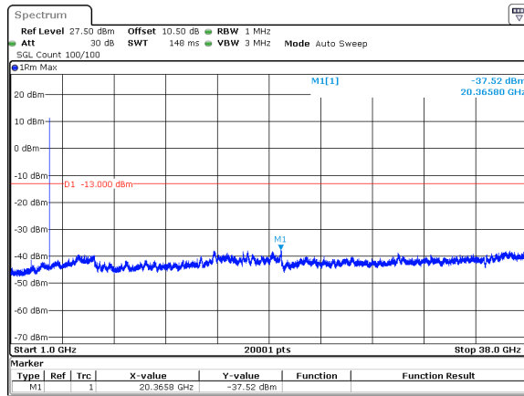
15MHz_15kHz_3750MHz_DFT-s-OFDM QPSK_RB1@0&amp;-37.52 dBm
