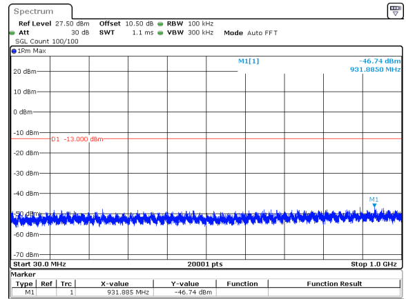
50MHz_30kHz_3775MHz_DFT-s-OFDM QPSK_RB1@0&amp;-46.74 dBm
