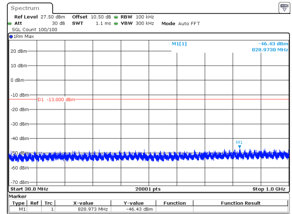
50MHz_15kHz_3750MHz_DFT-s-OFDM QPSK_RB1@0&amp;-46.43 dBm
