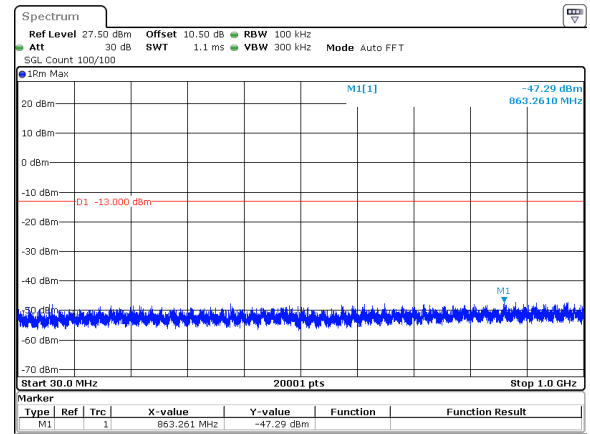
15MHz_15kHz_3750MHz_DFT-s-OFDM QPSK_RB1@0&amp;-47.29 dBm
