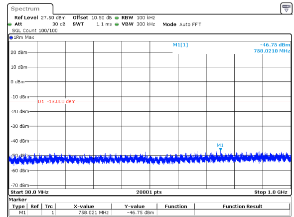
70MHz_30kHz_3735MHz_DFT-s-OFDM QPSK_RB1@188&amp;-46.75 dBm
