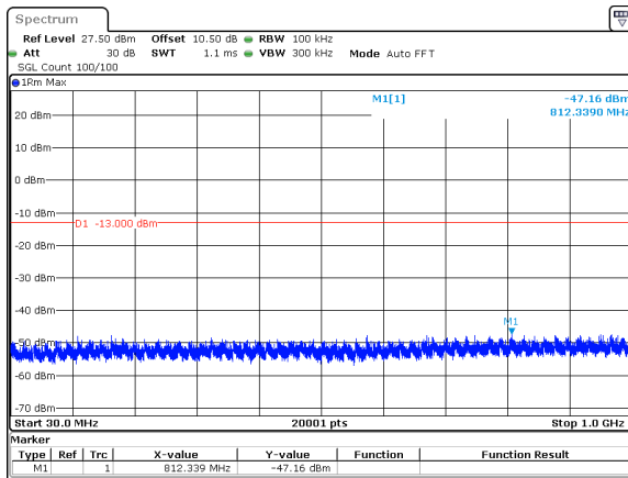
60MHz_30kHz_3730MHz_DFT-s-OFDM QPSK_RB1@161&amp;-47.16 dBm
