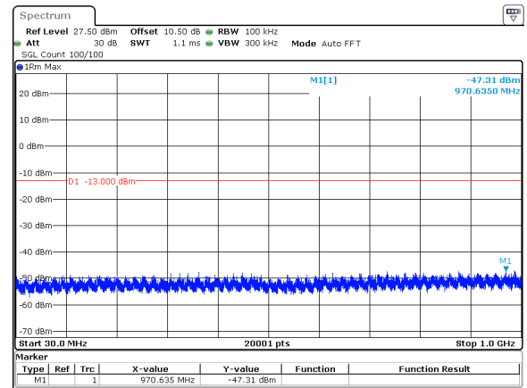
25MHz_30kHz_3750MHz_DFT-s-OFDM QPSK_RB1@64&amp;-47.31 dBm
