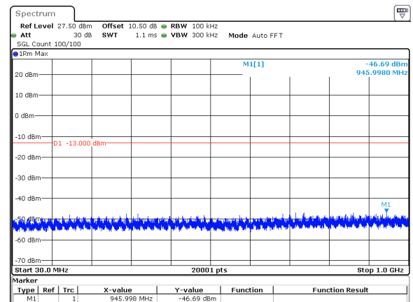
40MHz_15kHz_3720MHz_DFT-s-OFDM QPSK_RB216@0&amp;-46.69 dBm
