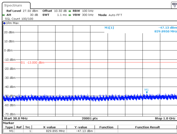
15MHz_15kHz_3792.5MHz_DFT-s-OFDM QPSK_RB1@0&amp;-47.13 dBm
