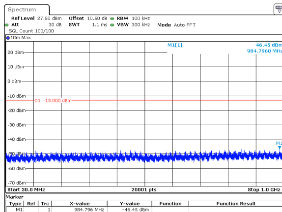
15MHz_15kHz_3750MHz_DFT-s-OFDM QPSK_RB75@0&amp;-46.45 dBm
