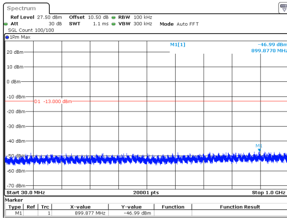
40MHz_15kHz_3720MHz_DFT-s-OFDM QPSK_RB1@0&amp;-46.99 dBm
