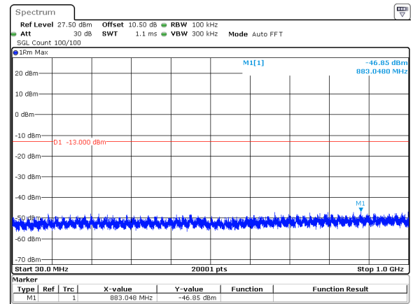
50MHz_15kHz_3725MHz_DFT-s-OFDM QPSK_RB1@269&amp;-46.85 dBm
