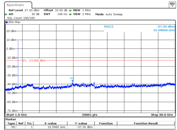
15MHz_30kHz_3750MHz_DFT-s-OFDM QPSK_RB1@0&amp;-37.35 dBm
