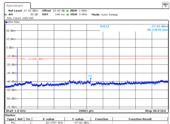
30MHz_15kHz_3750MHz_DFT-s-OFDM QPSK_RB160@0&amp;-37.62 dBm
