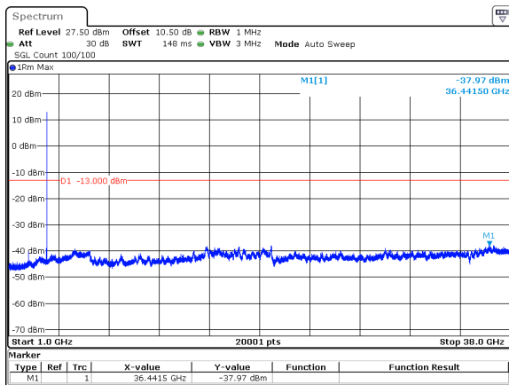
15MHz_15kHz_3792.5MHz_DFT-s-OFDM QPSK_RB1@78&amp;-37.97 dBm
