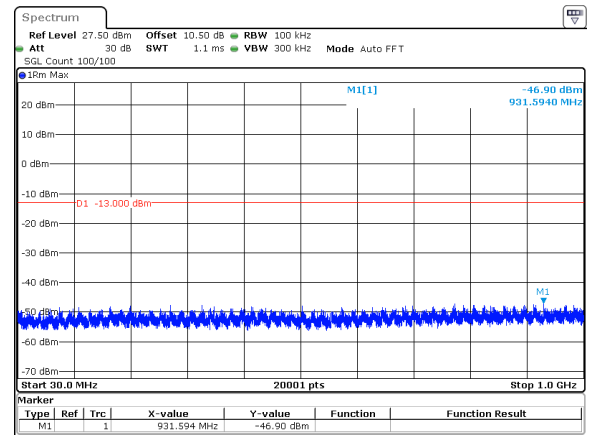
30MHz_30kHz_3715MHz_DFT-s-OFDM QPSK_RB1@77&amp;-46.90 dBm
