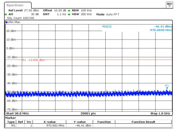
25MHz_30kHz_3712.5MHz_DFT-s-OFDM QPSK_RB1@0&amp;-46.41 dBm
