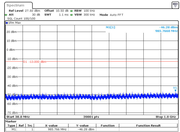
70MHz_30kHz_3750MHz_DFT-s-OFDM QPSK_RB1@188&amp;-46.28 dBm
