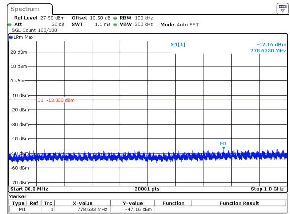
15MHz_30kHz_3792.5MHz_DFT-s-OFDM QPSK_RB1@37&amp;-47.16 dBm
