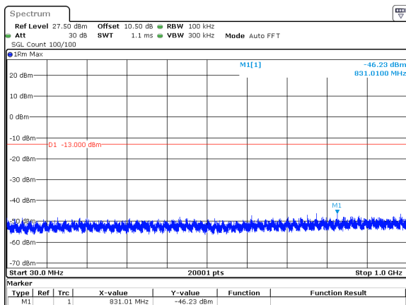
30MHz_15kHz_3750MHz_DFT-s-OFDM QPSK_RB160@0&amp;-46.23 dBm
