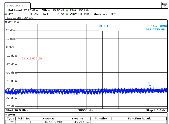
25MHz_15kHz_3712.5MHz_DFT-s-OFDM QPSK_RB128@0&amp;-46.73 dBm
