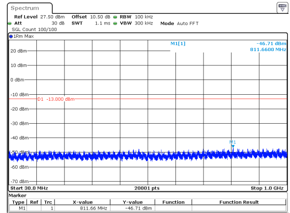
50MHz_15kHz_3725MHz_DFT-s-OFDM QPSK_RB1@0&amp;-46.71 dBm
