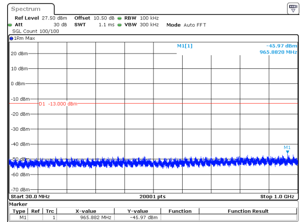
30MHz_15kHz_3750MHz_DFT-s-OFDM QPSK_RB1@159&amp;-45.97 dBm
