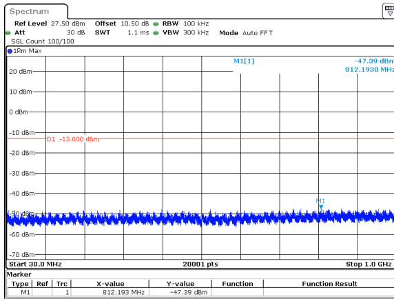
15MHz_30kHz_3750MHz_DFT-s-OFDM QPSK_RB1@0&amp;-47.39 dBm
