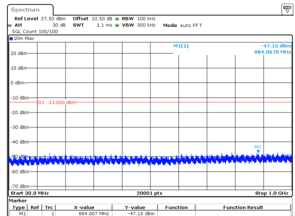
25MHz_30kHz_3750MHz_DFT-s-OFDM QPSK_RB64@0&amp;-47.15 dBm
