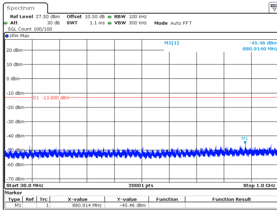
25MHz_30kHz_3750MHz_DFT-s-OFDM QPSK_RB1@0&amp;-45.46 dBm
