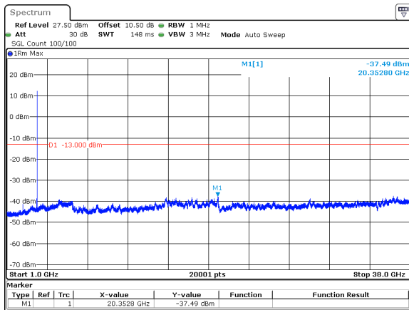
30MHz_15kHz_3750MHz_DFT-s-OFDM QPSK_RB1@159&amp;-37.49 dBm
