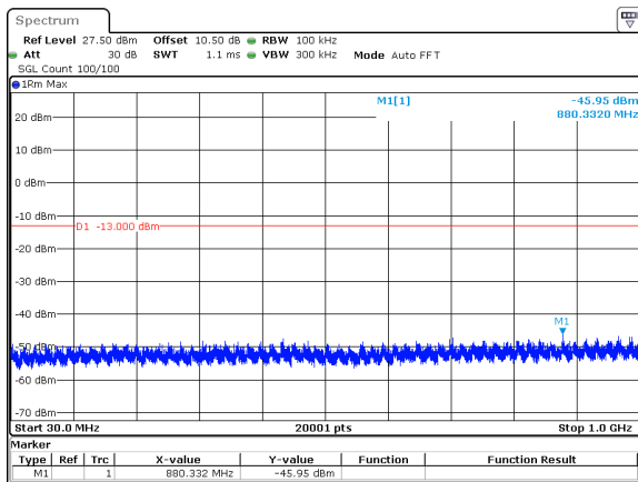
15MHz_30kHz_3707.5MHz_DFT-s-OFDM QPSK_RB1@37&amp;-45.95 dBm
