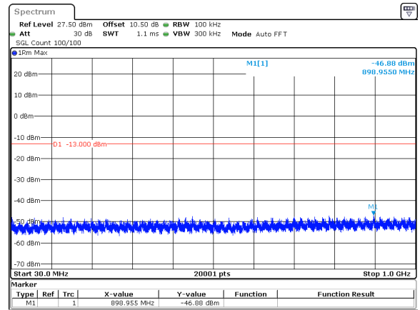
50MHz_30kHz_3725MHz_DFT-s-OFDM QPSK_RB1@0&amp;-46.88 dBm
