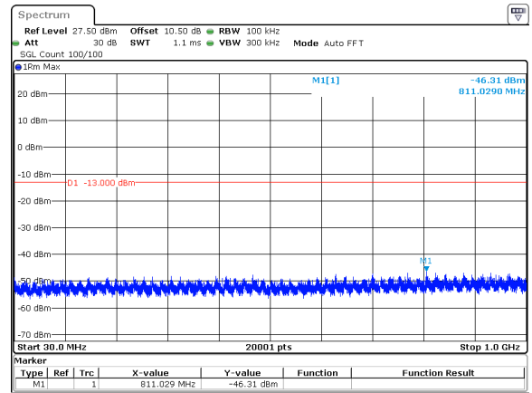
25MHz_15kHz_3750MHz_DFT-s-OFDM QPSK_RB1@0&amp;-46.31 dBm
