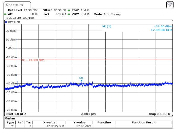
40MHz_30kHz_3750MHz_DFT-s-OFDM QPSK_RB1@0&amp;-37.60 dBm
