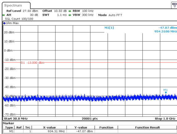
30MHz_15kHz_3785MHz_DFT-s-OFDM QPSK_RB1@159&amp;-47.07 dBm
