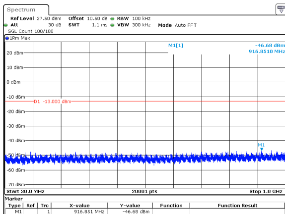
40MHz_15kHz_3750MHz_DFT-s-OFDM QPSK_RB216@0&amp;-46.68 dBm
