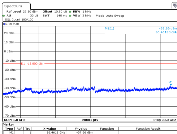
30MHz_15kHz_3715MHz_DFT-s-OFDM QPSK_RB160@0&amp;-37.66 dBm
