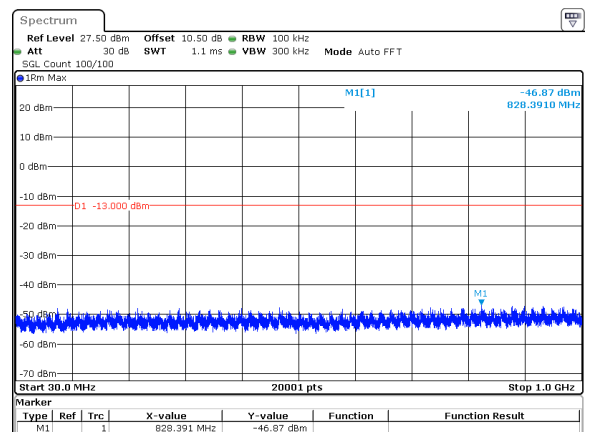
15MHz_15kHz_3792.5MHz_DFT-s-OFDM QPSK_RB75@0&amp;-46.87 dBm
