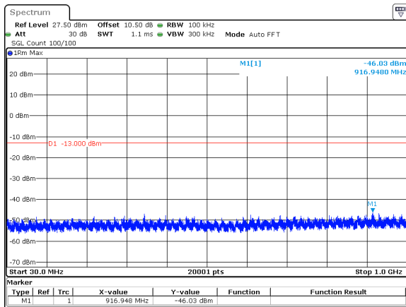
40MHz_15kHz_3750MHz_DFT-s-OFDM QPSK_RB1@215&amp;-46.03 dBm
