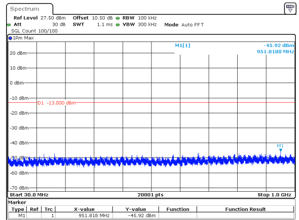
40MHz_30kHz_3750MHz_DFT-s-OFDM QPSK_RB1@105&amp;-45.92 dBm
