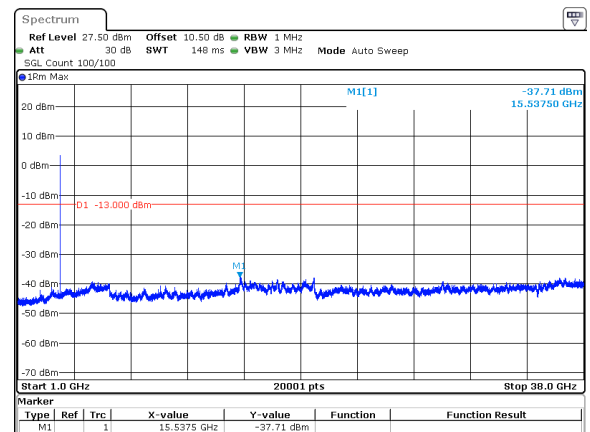
15MHz_15kHz_3750MHz_DFT-s-OFDM QPSK_RB75@0&amp;-37.71 dBm
