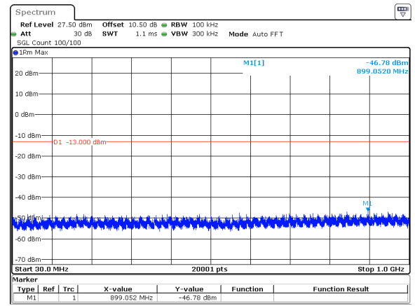
25MHz_30kHz_3787.5MHz_DFT-s-OFDM QPSK_RB1@0&amp;-46.78 dBm
