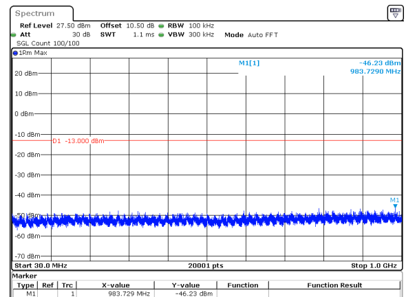
50MHz_30kHz_3750MHz_DFT-s-OFDM QPSK_RB128@0&amp;-46.23 dBm
