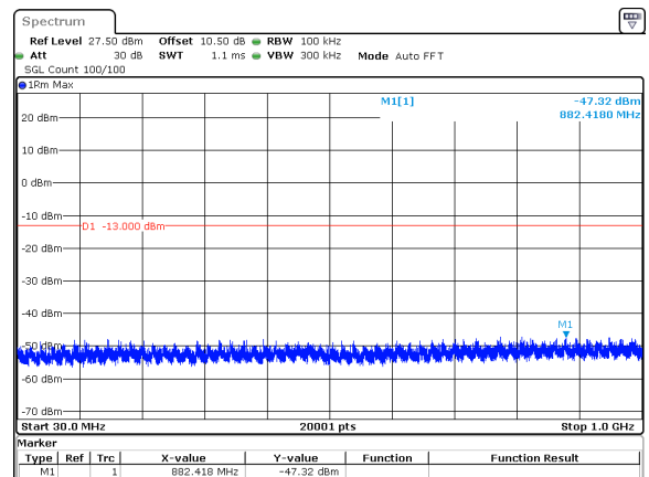
60MHz_30kHz_3750MHz_DFT-s-OFDM QPSK_RB162@0&amp;-47.32 dBm
