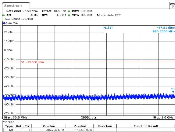
25MHz_30kHz_3712.5MHz_DFT-s-OFDM QPSK_RB64@0&amp;-47.21 dBm
