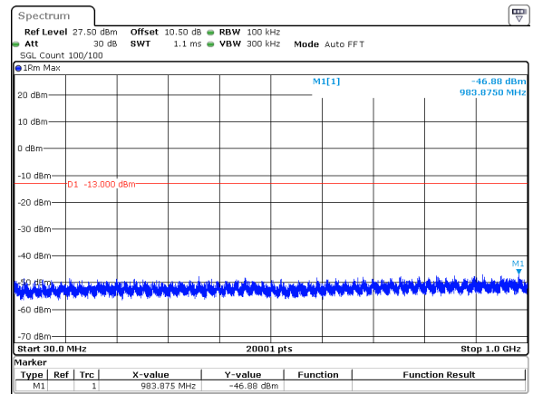
30MHz_15kHz_3715MHz_DFT-s-OFDM QPSK_RB1@159&amp;-46.88 dBm
