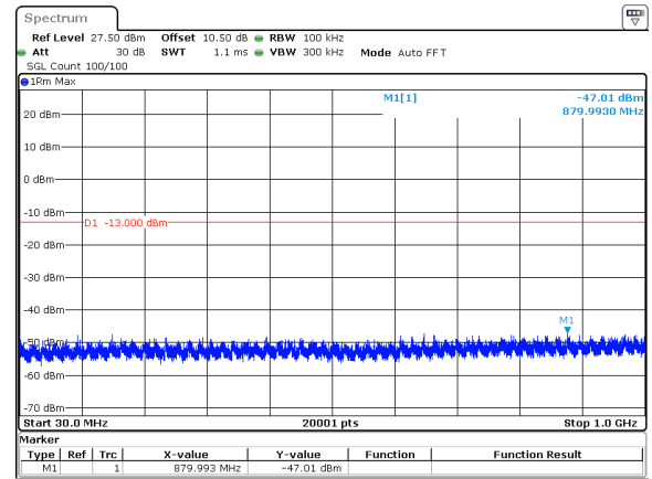
50MHz_15kHz_3775MHz_DFT-s-OFDM QPSK_RB1@0&amp;-47.01 dBm
