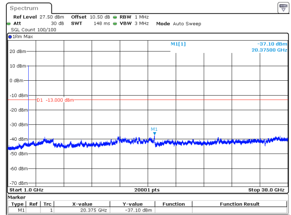
30MHz_15kHz_3715MHz_DFT-s-OFDM QPSK_RB1@0&amp;-37.10 dBm
