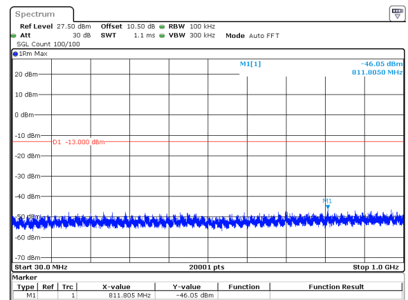
15MHz_30kHz_3707.5MHz_DFT-s-OFDM QPSK_RB36@0&amp;-46.05 dBm
