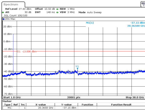
70MHz_30kHz_3735MHz_DFT-s-OFDM QPSK_RB1@188&amp;-37.15 dBm
