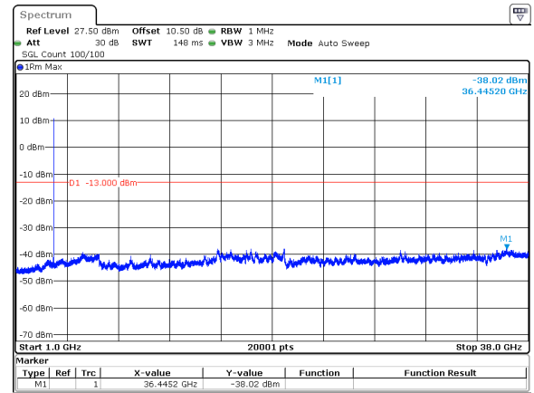
25MHz_30kHz_3712.5MHz_DFT-s-OFDM QPSK_RB1@64&amp;-38.02 dBm
