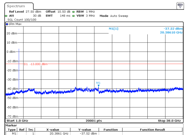
15MHz_30kHz_3750MHz_DFT-s-OFDM QPSK_RB36@0&amp;-37.52 dBm
