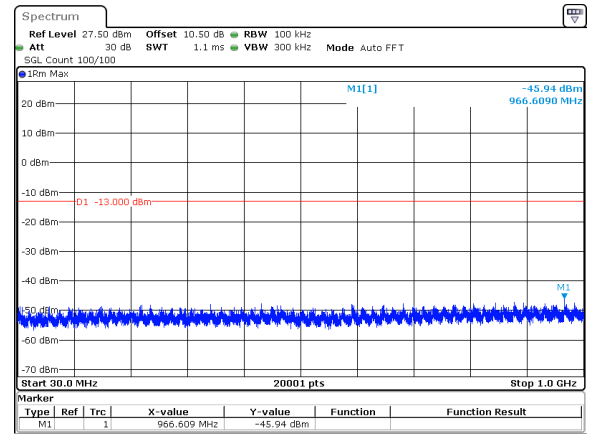
40MHz_30kHz_3780MHz_DFT-s-OFDM QPSK_RB1@0&amp;-45.94 dBm
