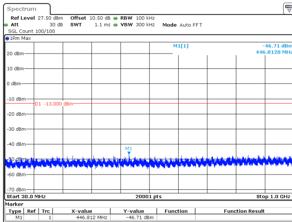
15MHz_30kHz_3750MHz_DFT-s-OFDM QPSK_RB1@37&amp;-46.71 dBm
