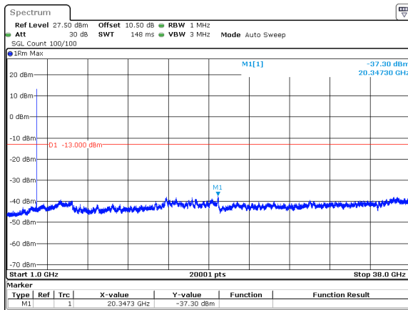
30MHz_15kHz_3715MHz_DFT-s-OFDM QPSK_RB1@159&amp;-37.30 dBm
