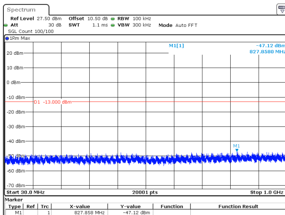
30MHz_30kHz_3715MHz_DFT-s-OFDM QPSK_RB75@0&amp;-47.12 dBm
