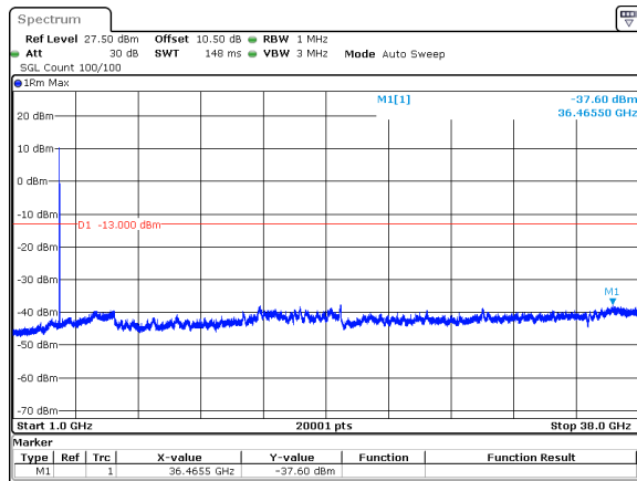
40MHz_30kHz_3720MHz_DFT-s-OFDM QPSK_RB1@105&amp;-37.60 dBm
