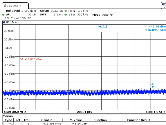
50MHz_15kHz_3725MHz_DFT-s-OFDM QPSK_RB270@0&amp;-46.54 dBm
