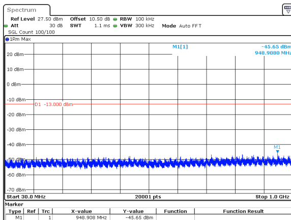
70MHz_30kHz_3735MHz_DFT-s-OFDM QPSK_RB180@0&amp;-45.65 dBm
