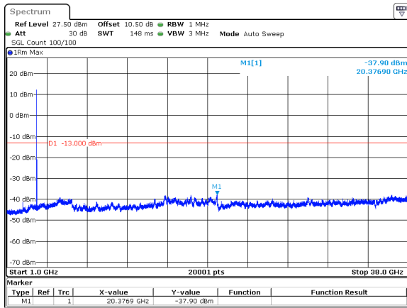
25MHz_15kHz_3750MHz_DFT-s-OFDM QPSK_RB1@0&amp;-37.90 dBm
