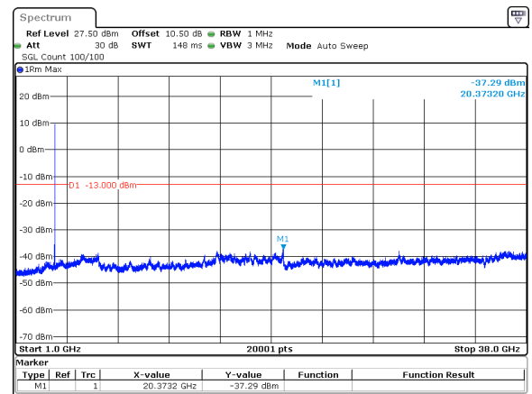
40MHz_30kHz_3780MHz_DFT-s-OFDM QPSK_RB1@105&amp;-37.29 dBm
