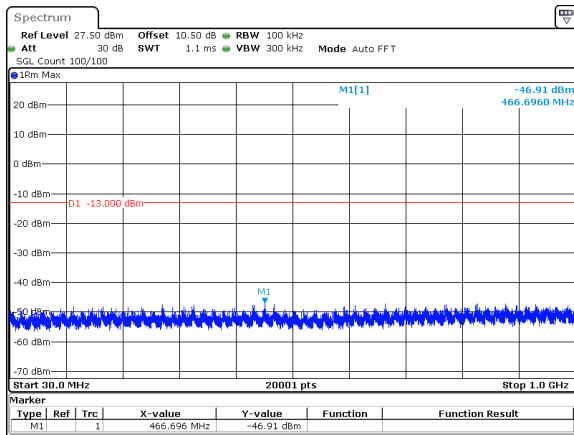
50MHz_30kHz_3725MHz_DFT-s-OFDM QPSK_RB1@132&amp;-46.91 dBm
