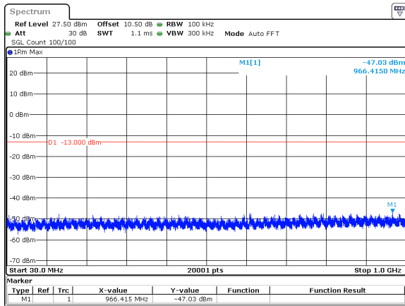
40MHz_15kHz_3750MHz_DFT-s-OFDM QPSK_RB1@0&amp;-47.03 dBm
