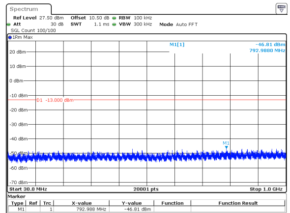
15MHz_15kHz_3792.5MHz_DFT-s-OFDM QPSK_RB1@78&amp;-46.81 dBm
