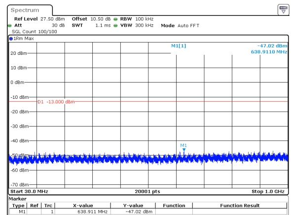
15MHz_30kHz_3792.5MHz_DFT-s-OFDM QPSK_RB36@0&amp;-47.02 dBm
