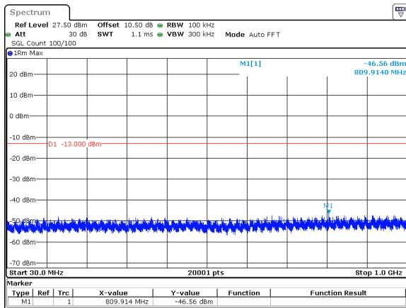
25MHz_15kHz_3750MHz_DFT-s-OFDM QPSK_RB1@132&amp;-46.56 dBm
