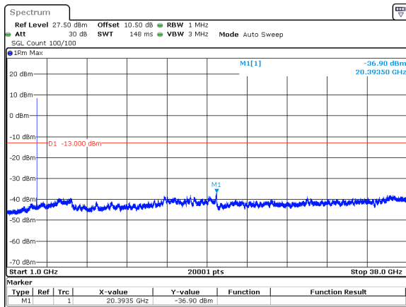
70MHz_30kHz_3750MHz_DFT-s-OFDM QPSK_RB1@188&amp;-36.90 dBm
