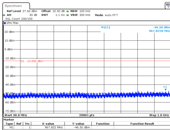
40MHz_30kHz_3780MHz_DFT-s-OFDM QPSK_RB1@105&amp;-46.50 dBm
