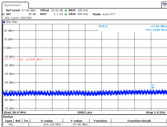
70MHz_30kHz_3765MHz_DFT-s-OFDM QPSK_RB1@188&amp;-47.06 dBm
