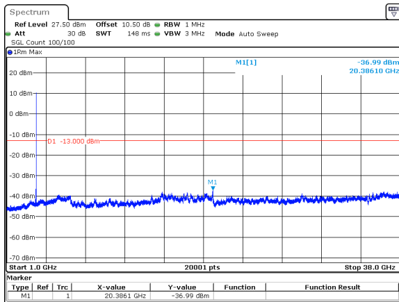
40MHz_30kHz_3750MHz_DFT-s-OFDM QPSK_RB1@105&amp;-36.99 dBm
