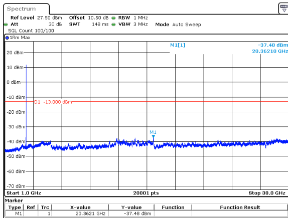
50MHz_30kHz_3750MHz_DFT-s-OFDM QPSK_RB1@132&amp;-37.48 dBm
