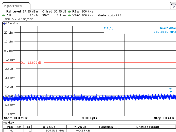
40MHz_15kHz_3780MHz_DFT-s-OFDM QPSK_RB216@0&amp;-46.57 dBm
