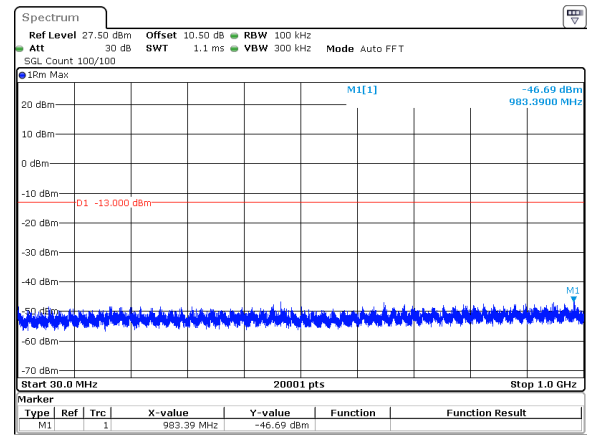
15MHz_30kHz_3707.5MHz_DFT-s-OFDM QPSK_RB1@0&amp;-46.69 dBm
