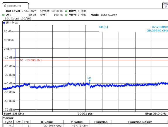
40MHz_30kHz_3750MHz_DFT-s-OFDM QPSK_RB100@0&amp;-37.73 dBm
