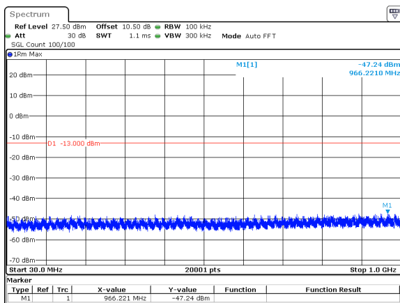
25MHz_30kHz_3787.5MHz_DFT-s-OFDM QPSK_RB64@0&amp;-47.24 dBm
