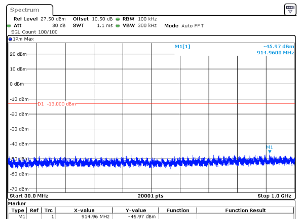
40MHz_30kHz_3720MHz_DFT-s-OFDM QPSK_RB100@0&amp;-45.97 dBm
