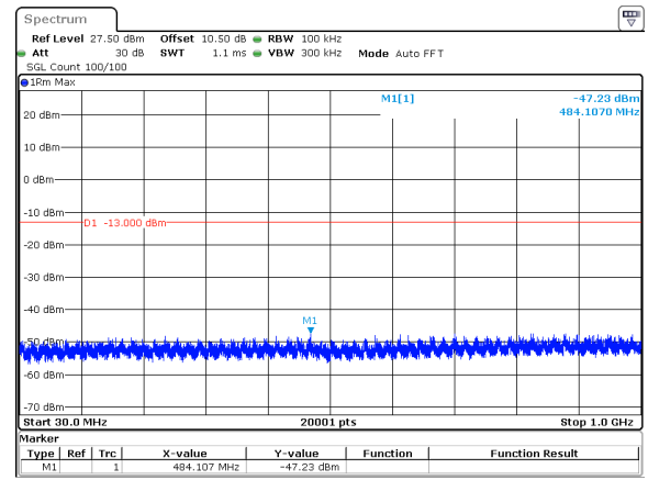
15MHz_30kHz_3792.5MHz_DFT-s-OFDM QPSK_RB1@0&amp;-47.23 dBm
