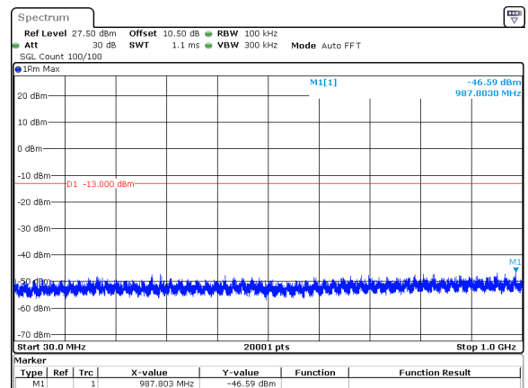
50MHz_30kHz_3775MHz_DFT-s-OFDM QPSK_RB128@0&amp;-46.59 dBm
