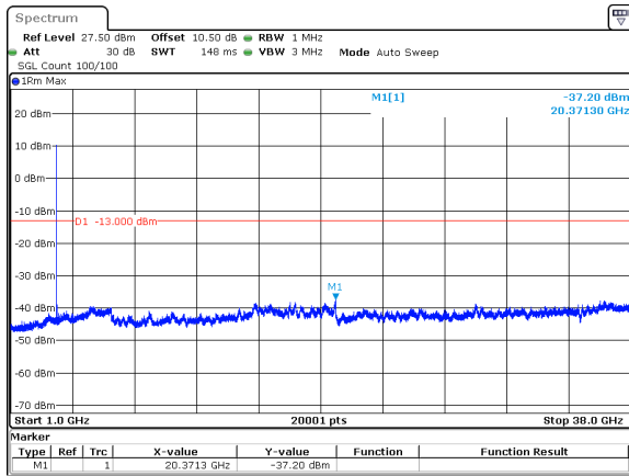
50MHz_30kHz_3725MHz_DFT-s-OFDM QPSK_RB1@0&amp;-37.20 dBm
