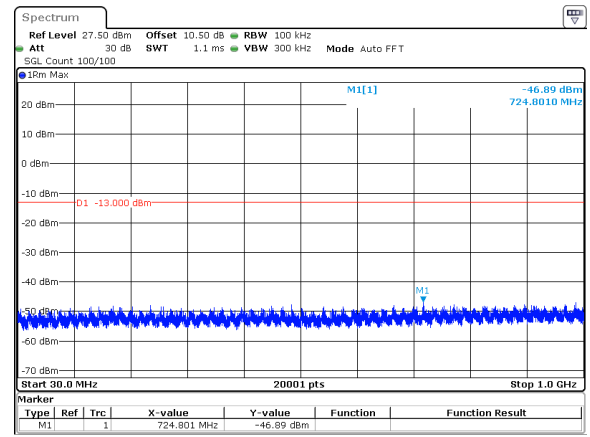
25MHz_15kHz_3787.5MHz_DFT-s-OFDM QPSK_RB1@0&amp;-46.89 dBm
