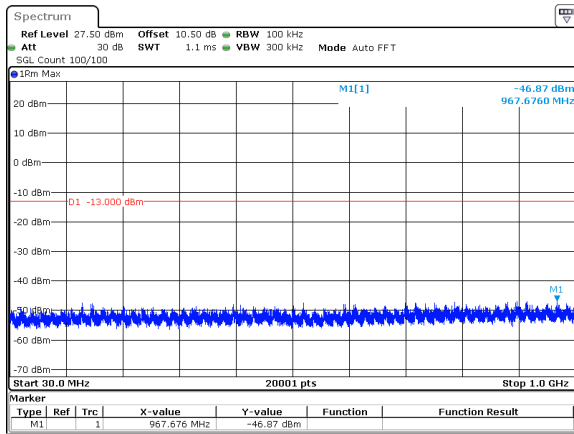
40MHz_15kHz_3780MHz_DFT-s-OFDM QPSK_RB1@0&amp;-46.87 dBm
