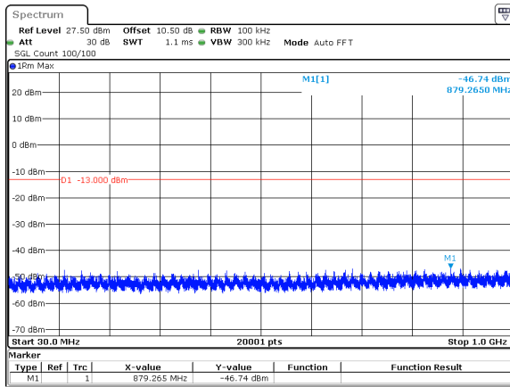
30MHz_30kHz_3715MHz_DFT-s-OFDM QPSK_RB1@0&amp;-46.74 dBm
