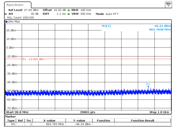
25MHz_15kHz_3712.5MHz_DFT-s-OFDM QPSK_RB1@132&amp;-46.34 dBm
