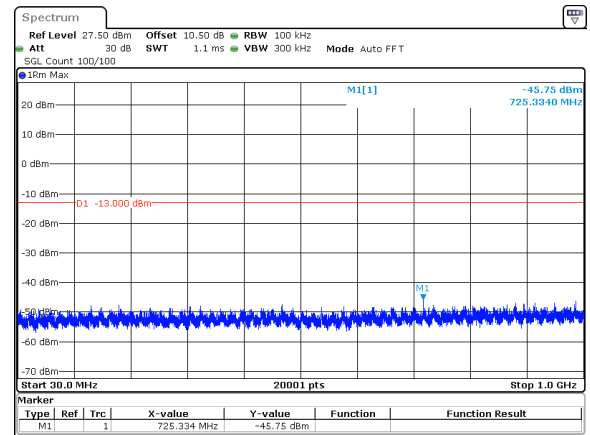
50MHz_30kHz_3750MHz_DFT-s-OFDM QPSK_RB1@132&amp;-45.75 dBm
