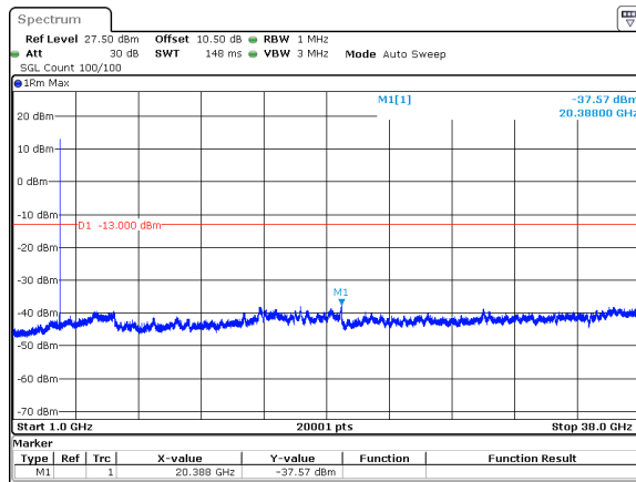
15MHz_15kHz_3750MHz_DFT-s-OFDM QPSK_RB1@78&amp;-37.57 dBm
