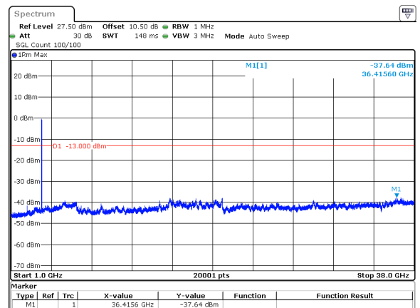
40MHz_15kHz_3780MHz_DFT-s-OFDM QPSK_RB216@0&amp;-37.64 dBm
