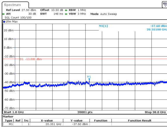
70MHz_30kHz_3735MHz_DFT-s-OFDM QPSK_RB1@0&amp;-37.60 dBm
