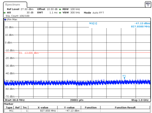
30MHz_30kHz_3785MHz_DFT-s-OFDM QPSK_RB1@77&amp;-47.13 dBm
