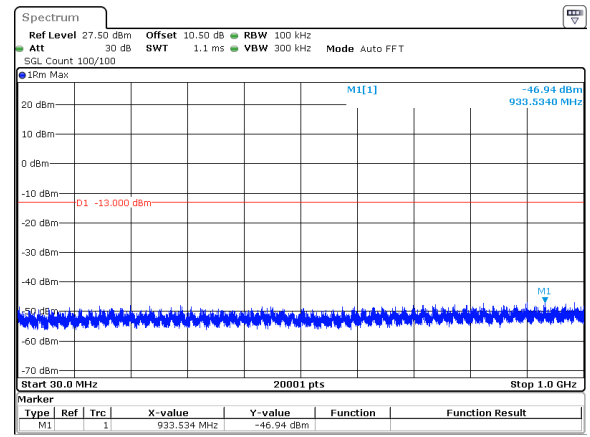
25MHz_15kHz_3712.5MHz_DFT-s-OFDM QPSK_RB1@0&amp;-46.94 dBm
