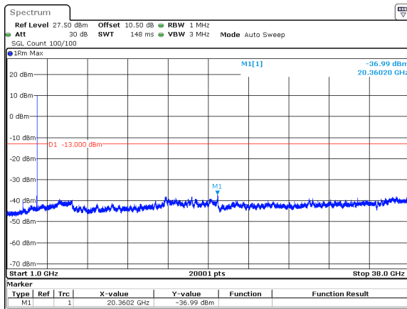
25MHz_30kHz_3750MHz_DFT-s-OFDM QPSK_RB1@64&amp;-36.99 dBm
