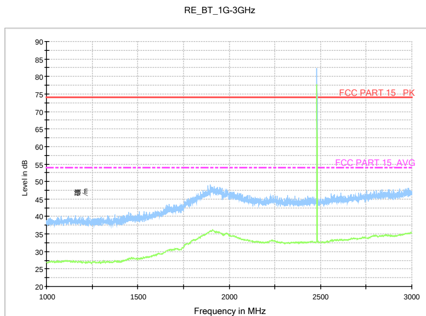
Fig.23. Radiated emission: GFSK, 2480MHz, 1 GHz - 3 GHz
