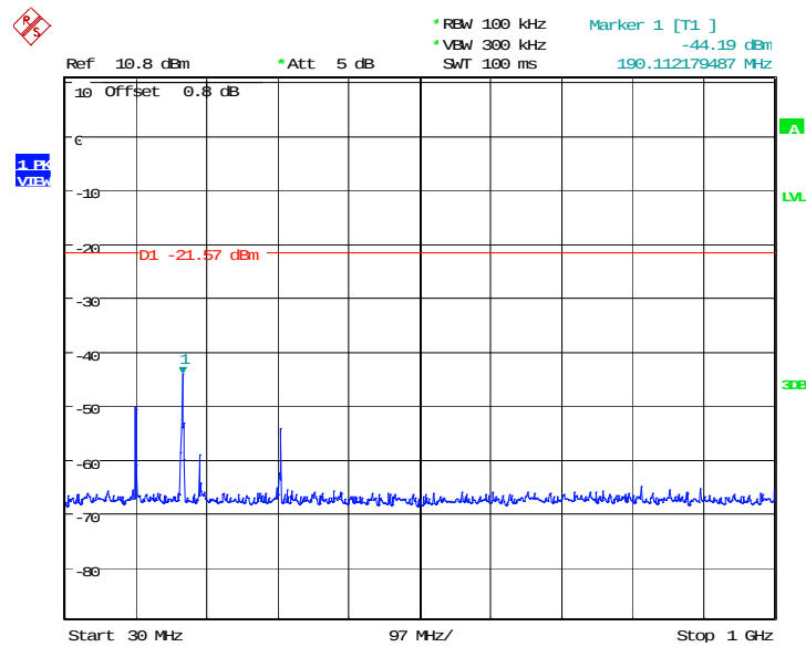
Fig.8. Conducted spurious emission: GFSK, 2440MHz
