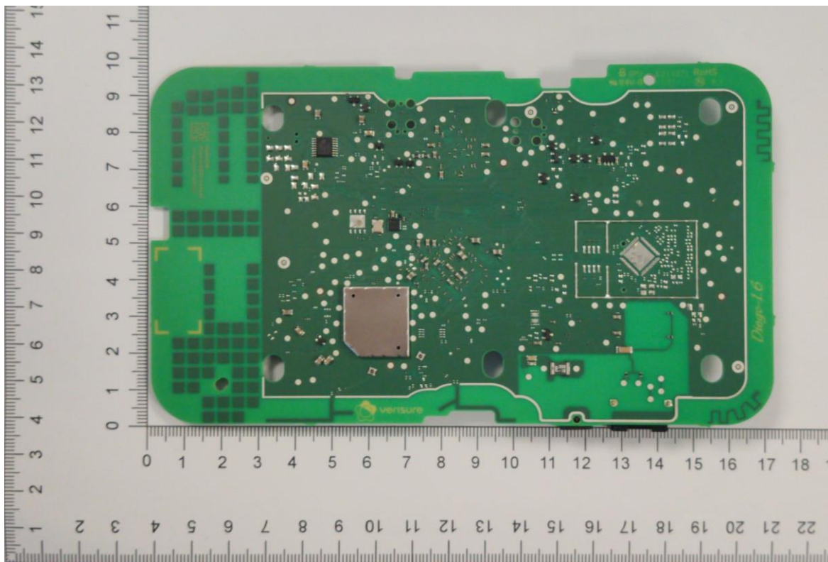
Figure 4 GWL-WXTND (489937) LATAM internal bottom view
