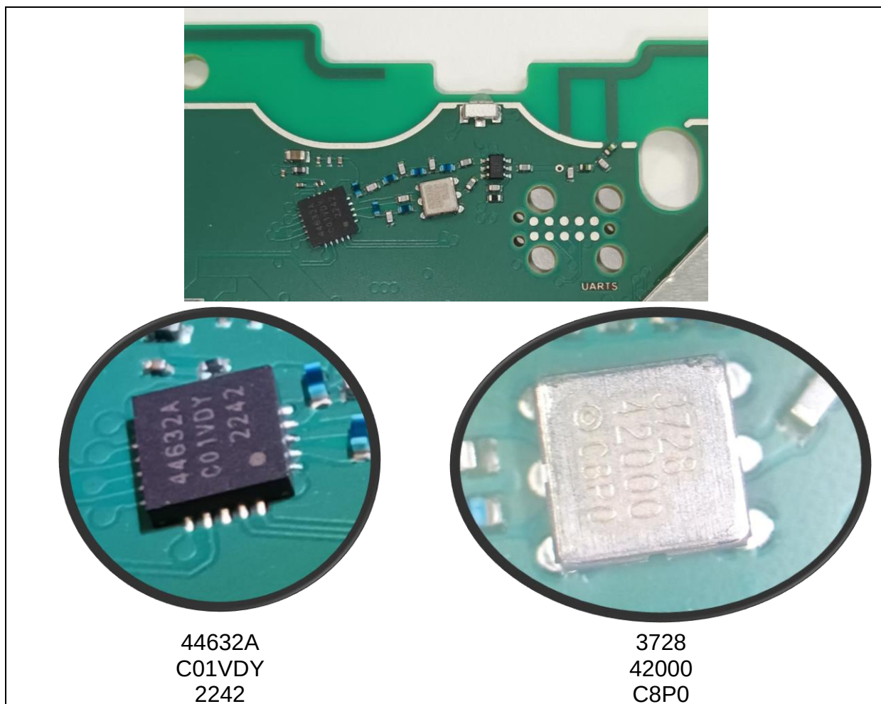
Figure 3 GWL-WXTND (489937) Zoom into ISM radio chip (left) and oscillator (Right)
