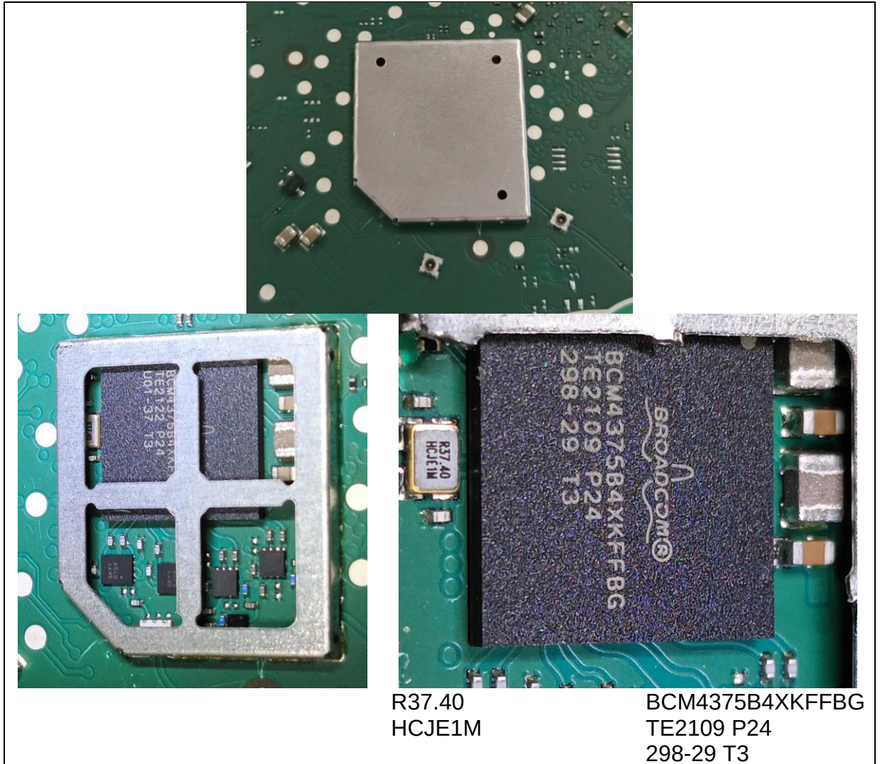
Figure 5 GWL-WXTND (489937) Zoom into Wi-Fi SoC and Xtal with metal frame (left) and removed (right)
