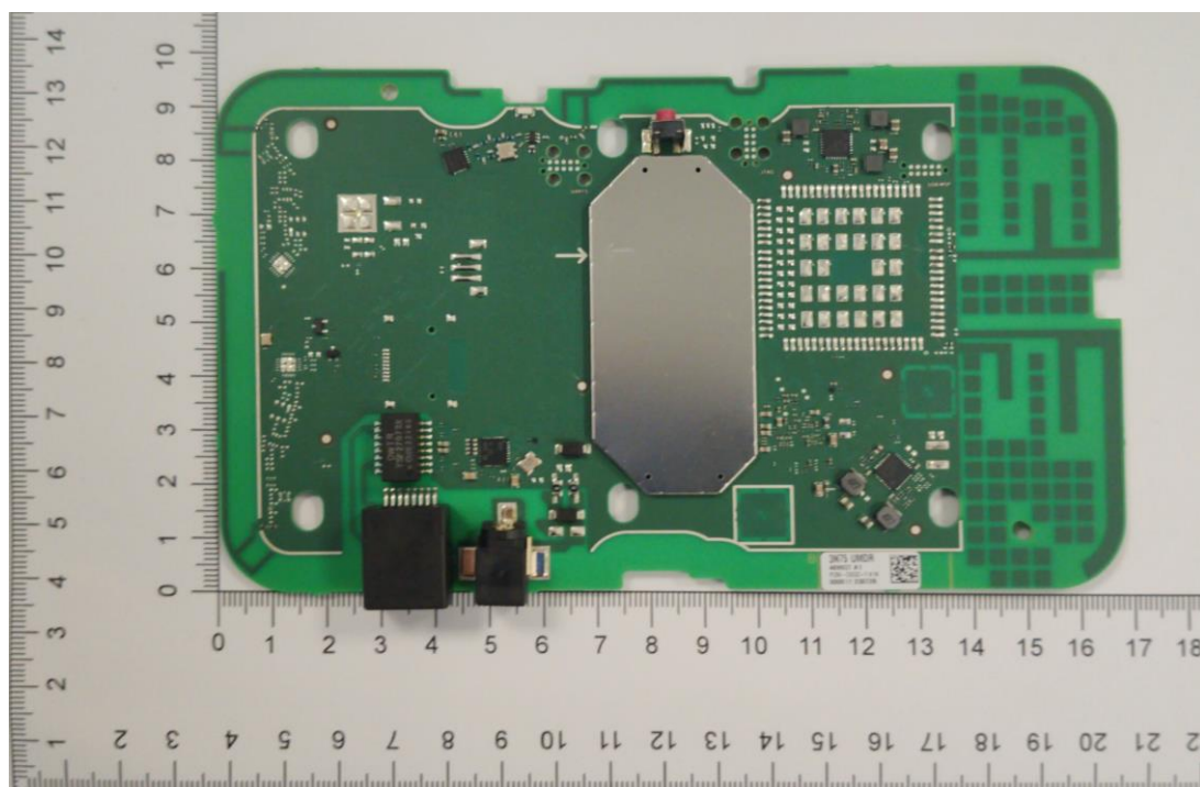
Figure 2 GWL-WXTND (489937) LATAM internal top view
