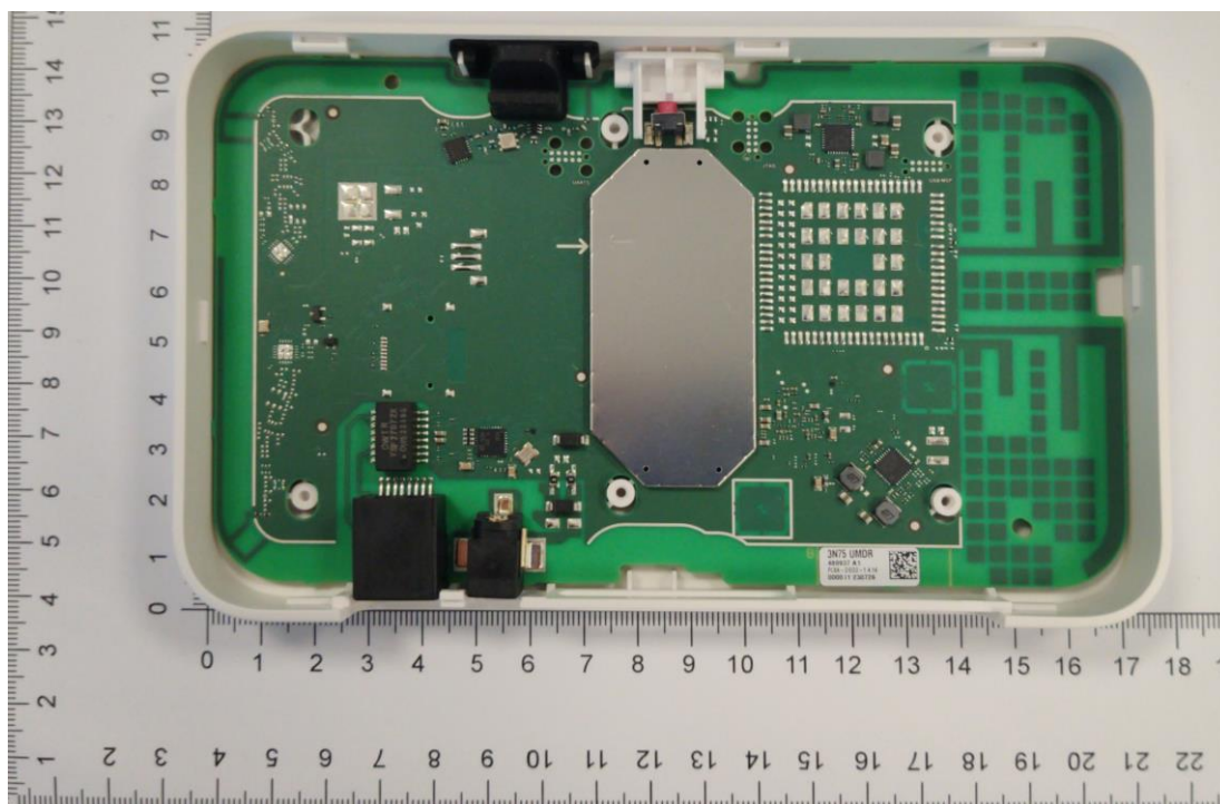
Figure 1 GWL-WXTND (489937) LATAM internal top view on housing
