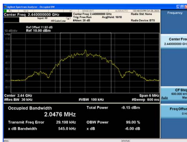
Modulation: 2Mbps 2440MHz
