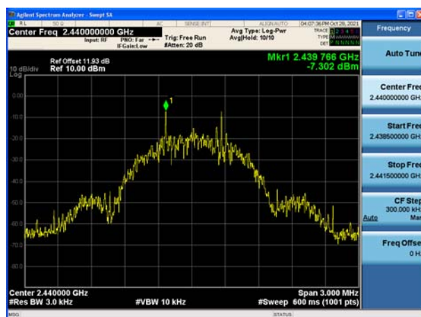
Modulation: Coded 500K 2440MHz
