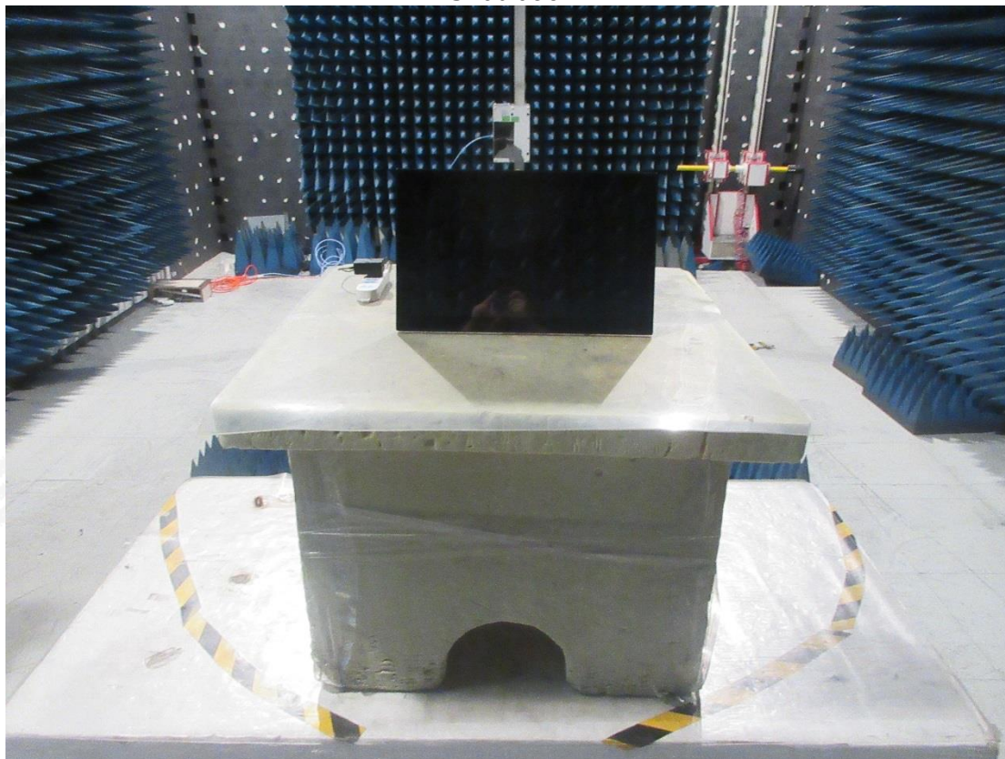
DTS radiation H
