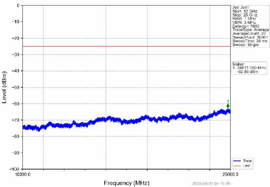
Band7_15MHz_QPSK_HCH_2562.5MHz_RB_1_0_NTNV
