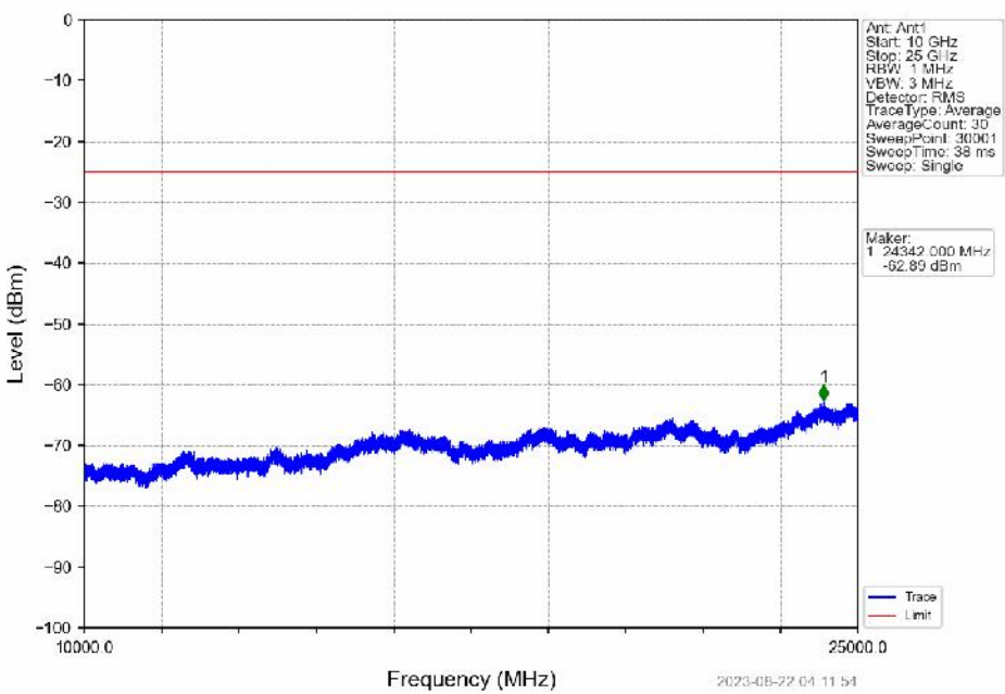
Band7_10MHz_16QAM_LCH_2505MHz_RB_1_0_NTNV
