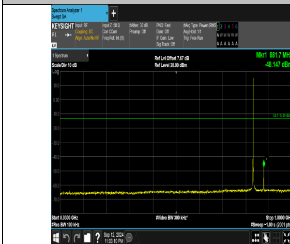
Band5_1.4MHz_QPSK_20525_1RB#5_30~1000_30~1000
