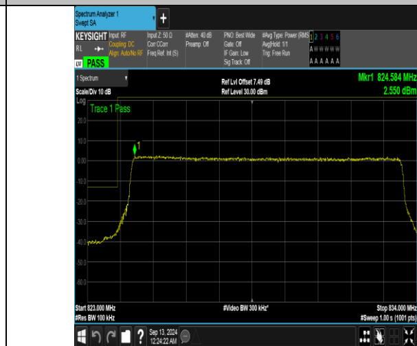
Band5_10MHz_16QAM_20450_50RB#0
