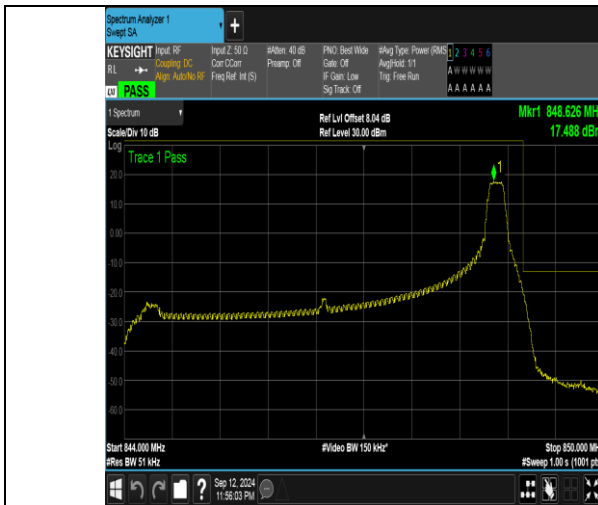
Band5_5MHz_QPSK_20625_1RB#24
