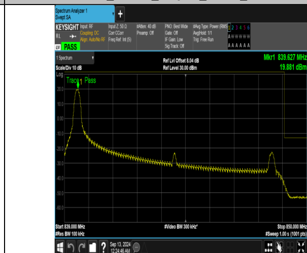
Band5_10MHz_16QAM_20600_1RB#0
