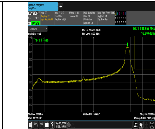
Band5_5MHz_16QAM_20625_1RB#24
