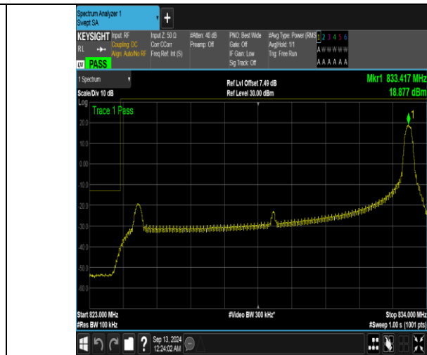
Band5_10MHz_16QAM_20450_1RB#49
