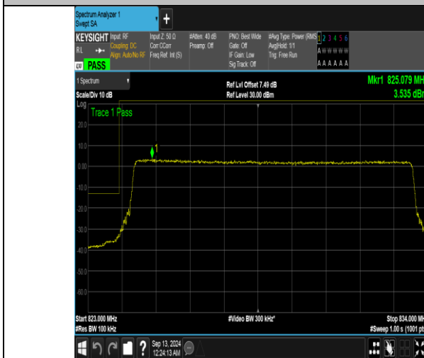
Band5_10MHz_QPSK_20450_50RB#0
