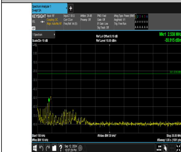
Band5_1.4MHz_16QAM_20407_1RB#0_0.15~30_0.15~30
