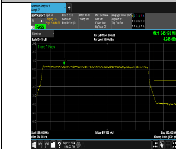
Band5_5MHz_QPSK_20625_25RB#0
