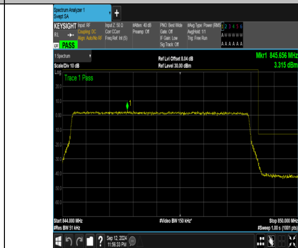
Band5_5MHz_16QAM_20625_25RB#0
