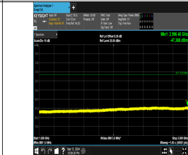
Band5_1.4MHz_QPSK_20407_1RB#5_1000~3000_1000~3000
