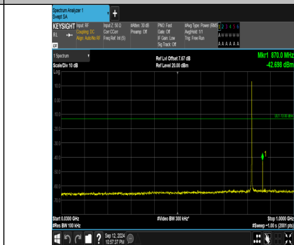
Band5_1.4MHz_16QAM_20407_1RB#0_30~1000_30~1000
