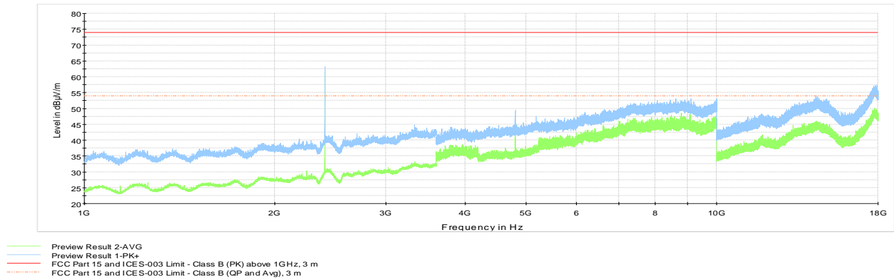
Figure 8.4-22: Radiated spurious emissions 1 to 18 GHz with antenna 4, Low channel
