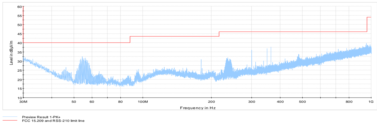
Figure 8.4-20: Radiated spurious emissions 30 MHz to 1 GHz with antenna 4, mid channel
