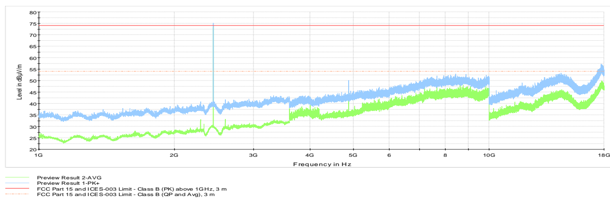
Figure 8.4-17: Radiated spurious emissions 1 to 18 GHz with antenna 3, mid channel
