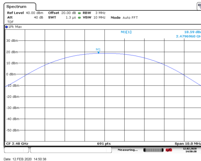
Figure 8.3-6: Conducted output power, high channel
