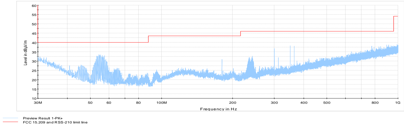
Figure 8.4-19: Radiated spurious emissions 30 MHz to 1 GHz with antenna 4, Low channel
