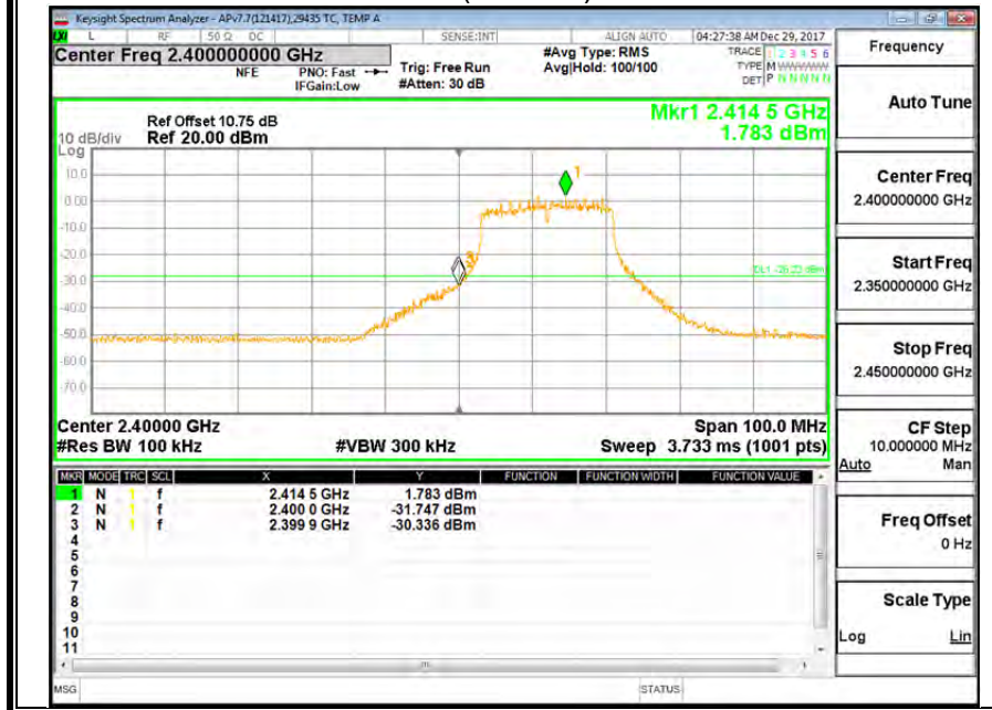
2.4GHz 2TX CDD CBE CH1 (Chain 1)
