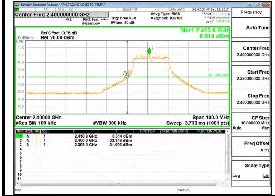
2.4GHz 2TX CDD CBE CH1 (Chain 0)
