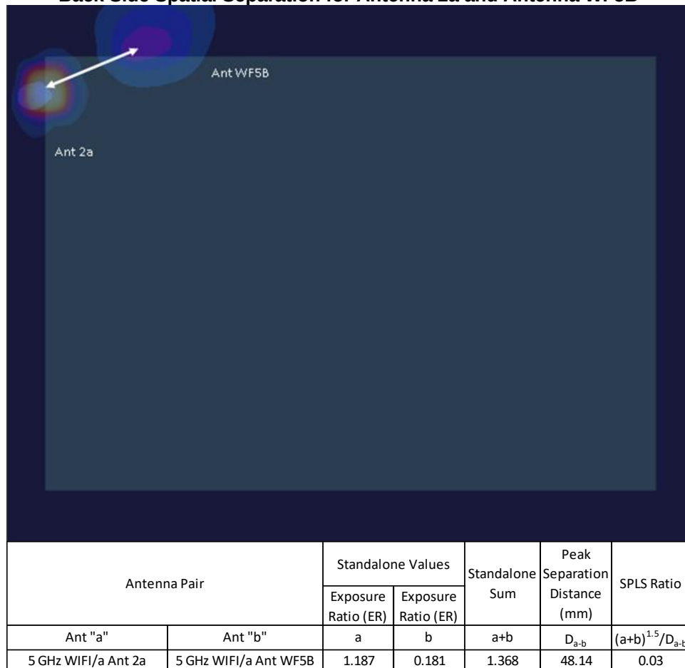
Figure 11-7 Back Side Spatial Separation for Antenna 2a and Antenna WF5B
