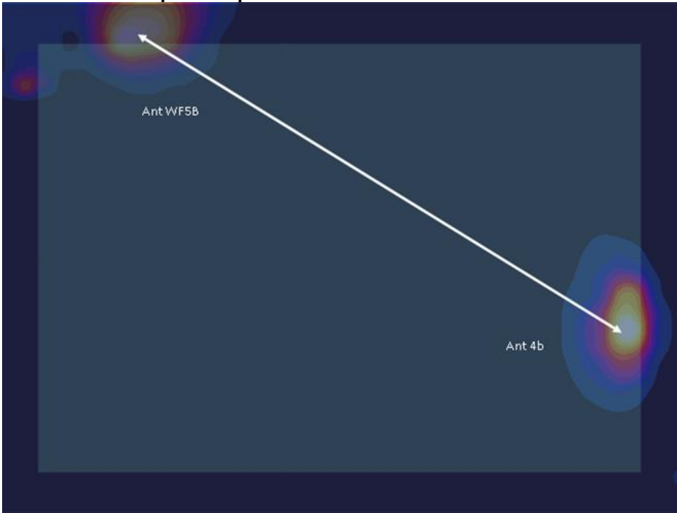
Figure 11-13 Back Side Spatial Separation for Antenna 4b and Antenna WF5B
