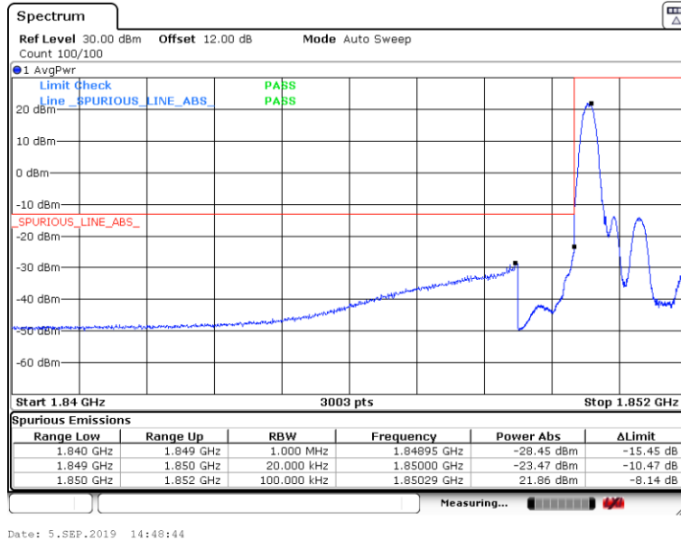
Band2-1.4MHz-QPSK-10607-6RB#0
