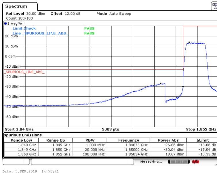
Band2-1.4MHz-QPSK-19193-1RB#0
