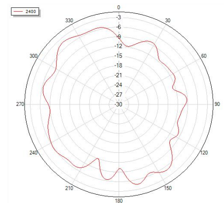
Phi=90 freq=2400MHz
