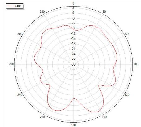
Phi=0 freq=2400MHz
