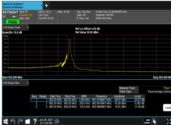
B2_N71(20M)_DFT-s- OFDM_QPSK_Edge_1RB_Left_Low_CH
