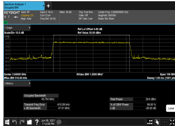
B2_N77(50M)_DFT-s- OFDM_QPSK_Outer_Full_Mid_CH
