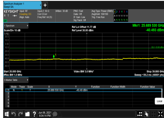
B2_N77(20M)_DFT-s- OFDM_BPSK_Edge_1RB_Left_High_CH
