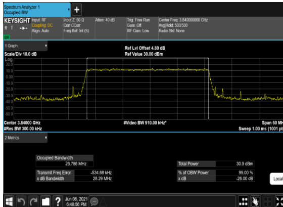
B2_N77(30M)_DFT-s-OFDM_PI_2- BPSK_Outer_Full_Mid_CH
