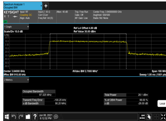
B2_N77(90M)_CP-OFDM_16 QAM_Outer_Full_Mid_CH
