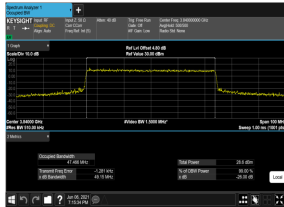
B2_N77(50M)_CP-OFDM_16 QAM_Outer_Full_Mid_CH
