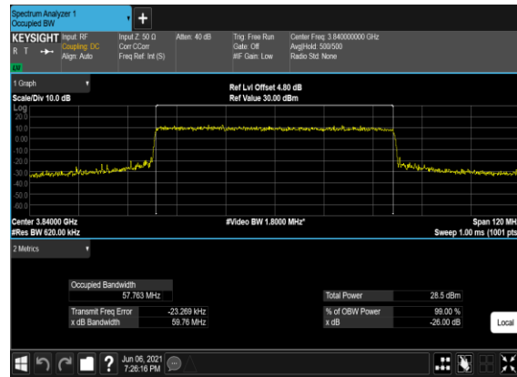
B2_N77(60M)_CP-OFDM_16 QAM_Outer_Full_Mid_CH
