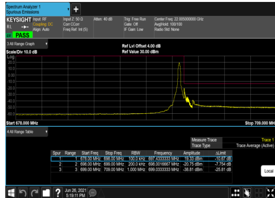
B2_N71(20M)_DFT-s- OFDM_BPSK_Edge_1RB_Right_High_CH
