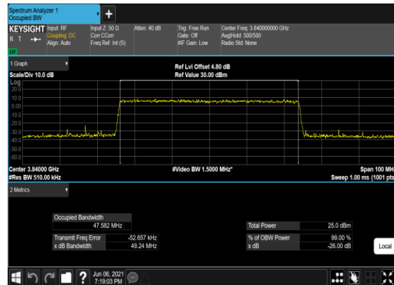
B2_N77(50M)_CP-OFDM_256 QAM_Outer_Full_Mid_CH
