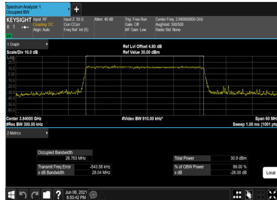
B2_N77(30M)_DFT-s- OFDM_QPSK_Outer_Full_Mid_CH
