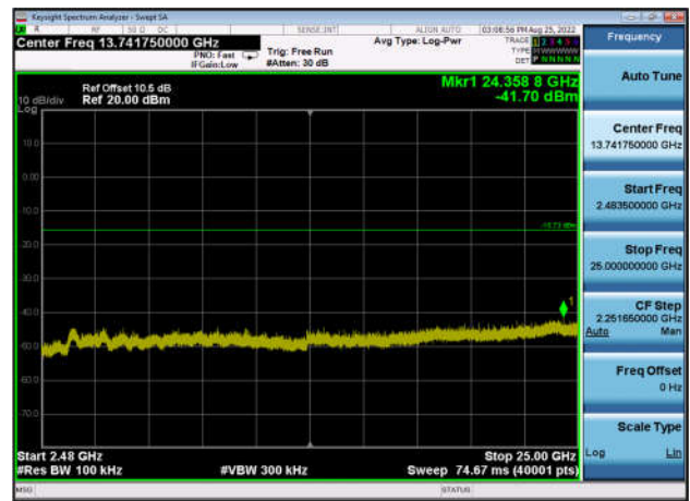
,Plot 4,2483.5MHz~25000MHz-802.11ax(H T20),2437MHz,Ant1
