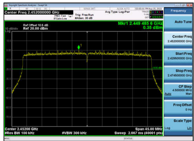
,Plot 1,Reference Level-802.11ax(HT40 ) ,2452MHz,Ant1
