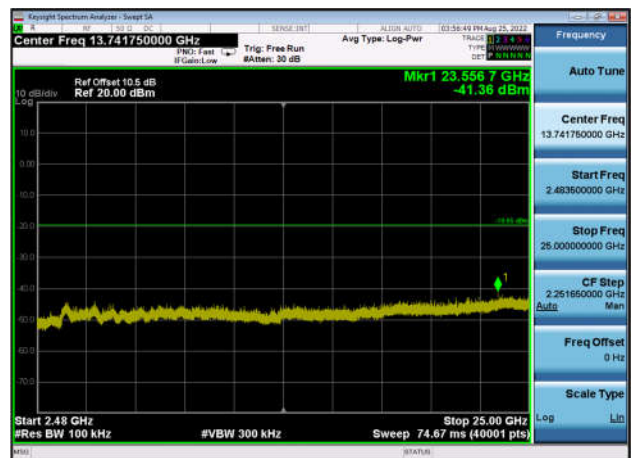
,Plot 4,2483.5MHz~25000MHz-802.11ax(H T40),2452MHz,Ant1
