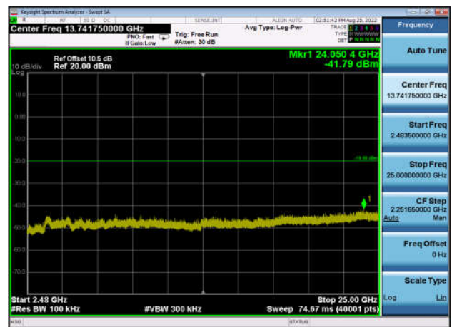
,Plot 4,2483.5MHz~25000MHz-802.11n(HT 40),2452MHz,Ant1
