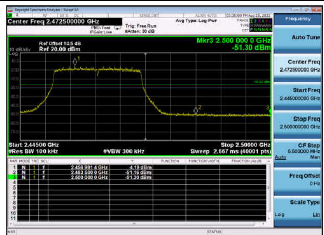
,Plot 2,Band Edge-802.11ax(HE20) ,2462MHz,Ant1
