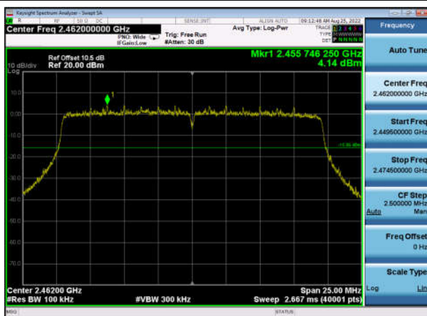
,Plot 1,Reference Level-802.11ax(HT20 ,2462MHz,Ant0
