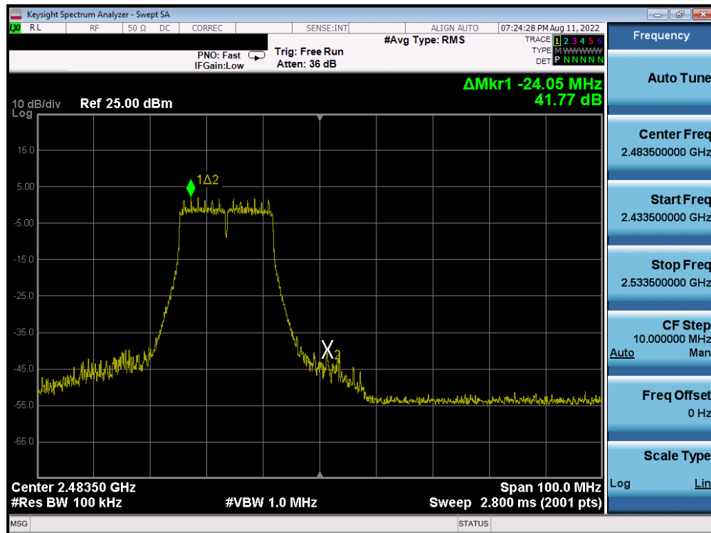
Plot 7-36. Band Edge Plot Antenna 1 (802.11g – Ch. 12)
