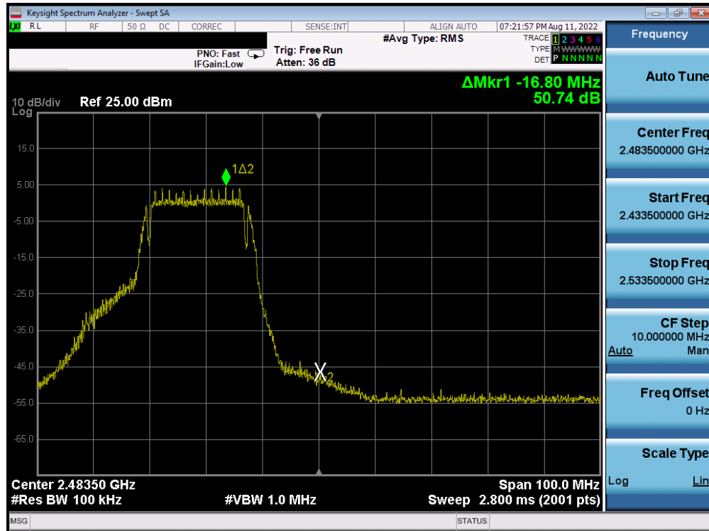
Plot 7-35. Band Edge Plot Antenna 1 (802.11g – Ch. 11)
