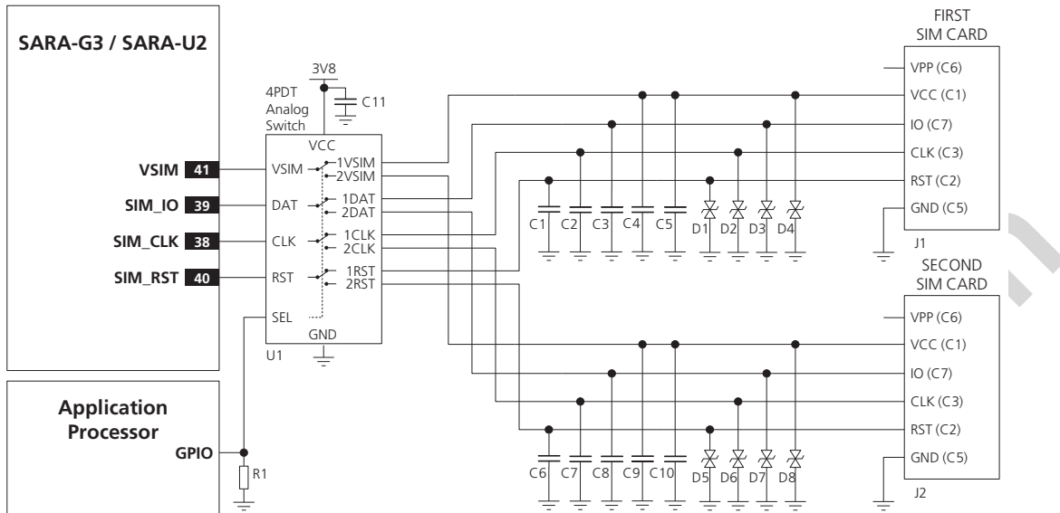
Figure 64: Application circuit for the connection to two removable SIM cards, with SIM detection not implemented
