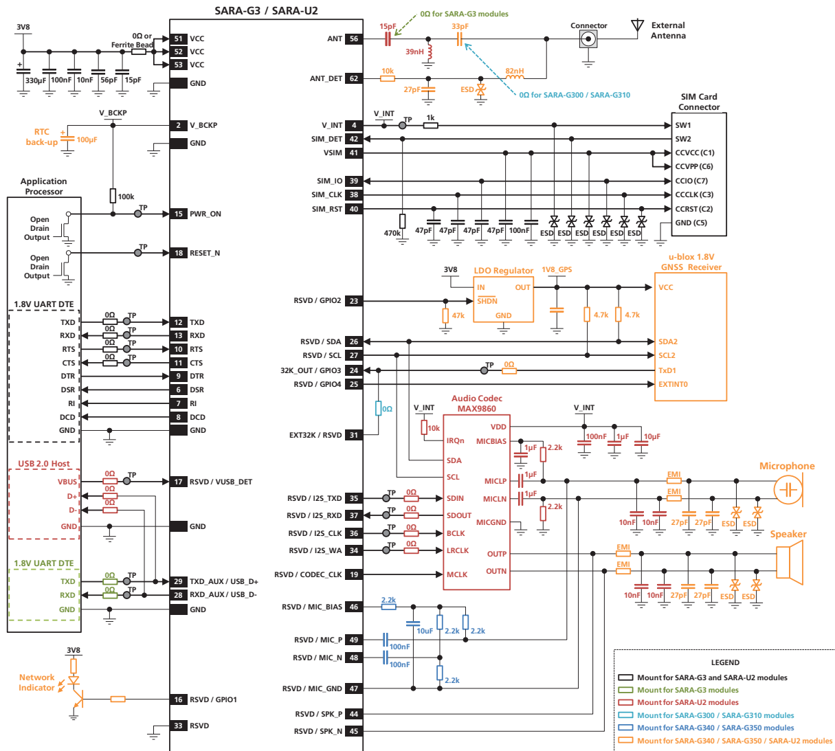
Figure 100: Example of complete schematic diagram to integrate SARA-G3 and SARA-U2 modules on the same application board
