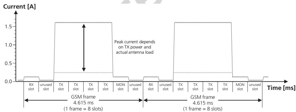
Figure 12: VCC current consumption profile versus time during a GPRS multi-slot class 12 connection (4 TX slots, 1 RX slot)
