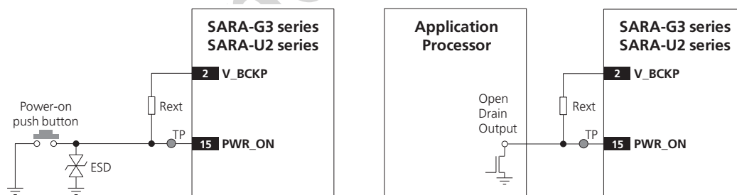
Figure 51: PWR_ON application circuits using a push button and an open drain output of an application processor
