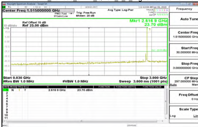
30MHz~3GHz_Band38_5MHz_QPSK_1_0_HighCH38225-2617.5
