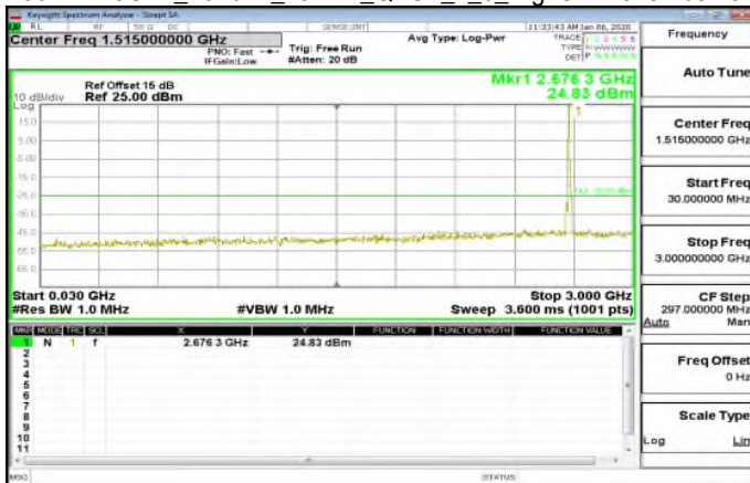
30MHz~3GHz_Band41_15MHz_QPSK_1_0_HighCH41515-2682.5
