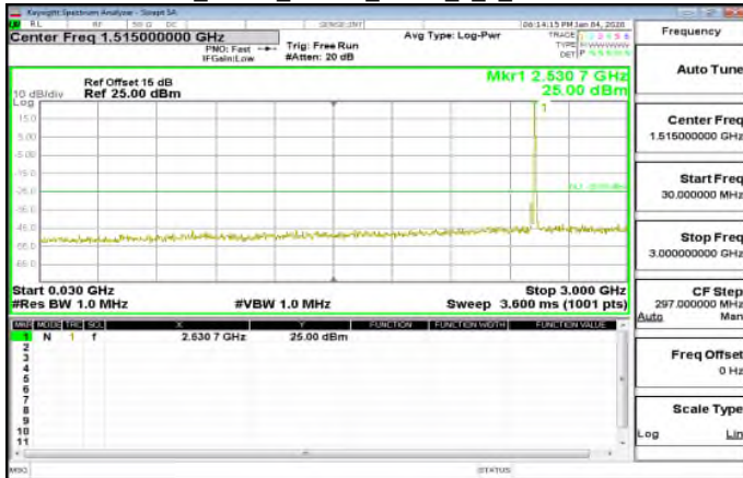
30MHz~3GHz_Band7_10MHz_QPSK_1_0_MidCH21100-2535
