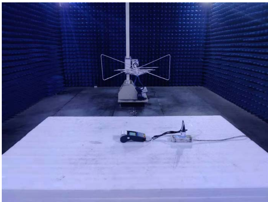
Photo of Radiated Emission Measurement (Below 1G) For adapter1
