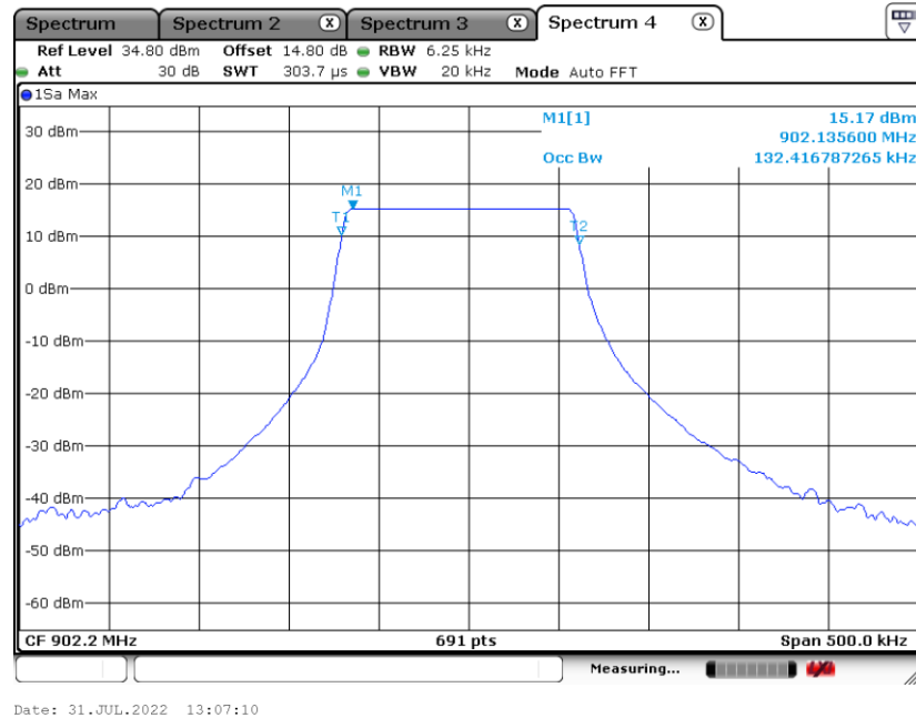
99% Occupied Bandwidth Plot on Channel 1
