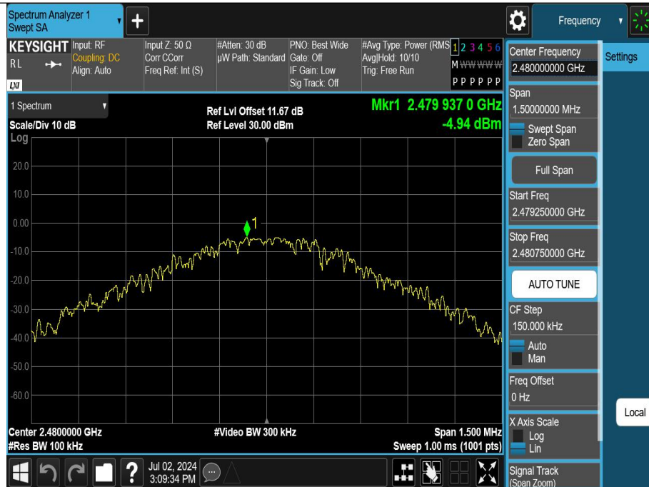
DH5-Ant1-2480-0~Reference-PASS
