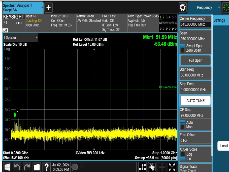
DH5-Ant1-2480-30~1000-PASS
