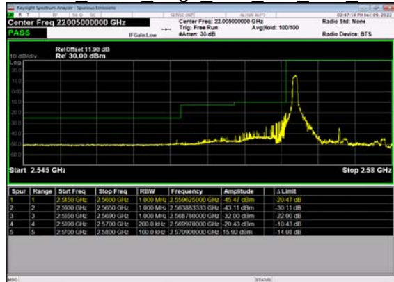
N38(10M)_DFT-s-OFDM BPSK Edge 1RB Left Low CH
