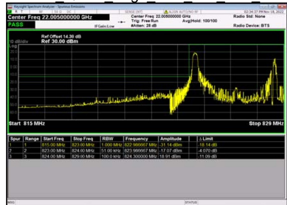
N5(5M)_DFT-s- OFDM QPSK Edge 1RB Left Low CH
