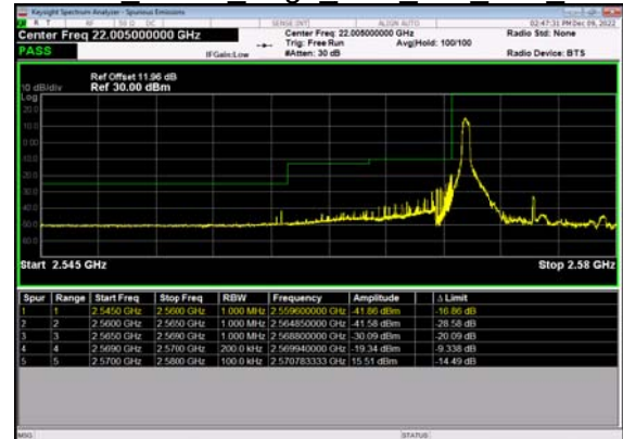
N38(10M)_DFT-s-OFDM QPSK Edge 1RB Left Low CH
