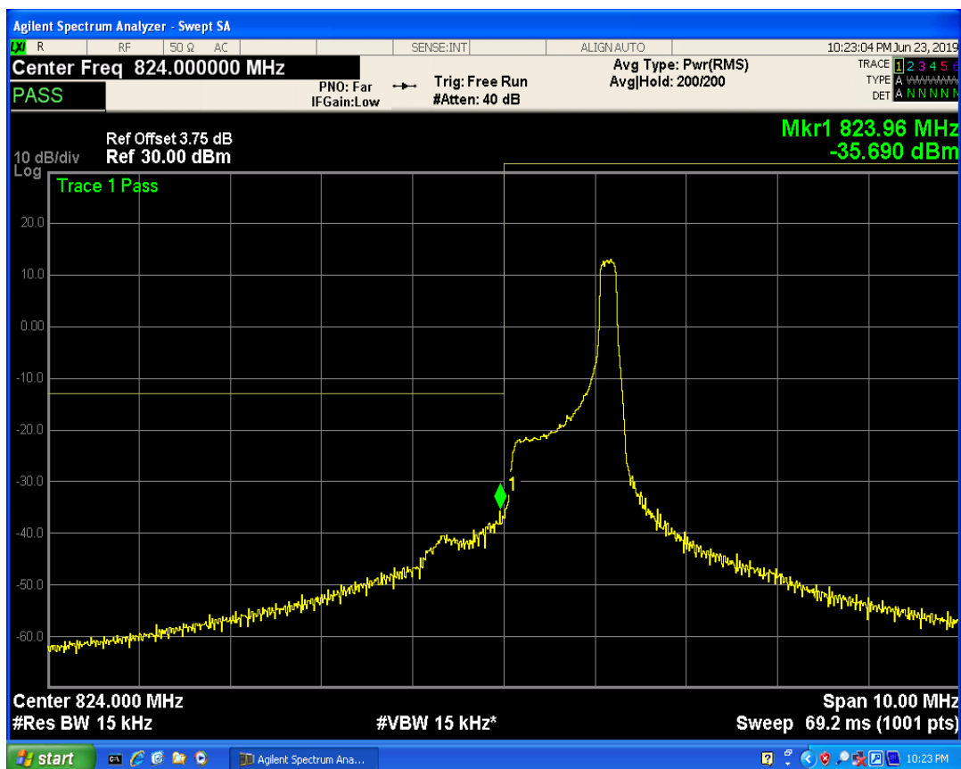
LTE Band5 QPSK BW=1.4MHz Channel=20407 RB Size=3 Position=#0
