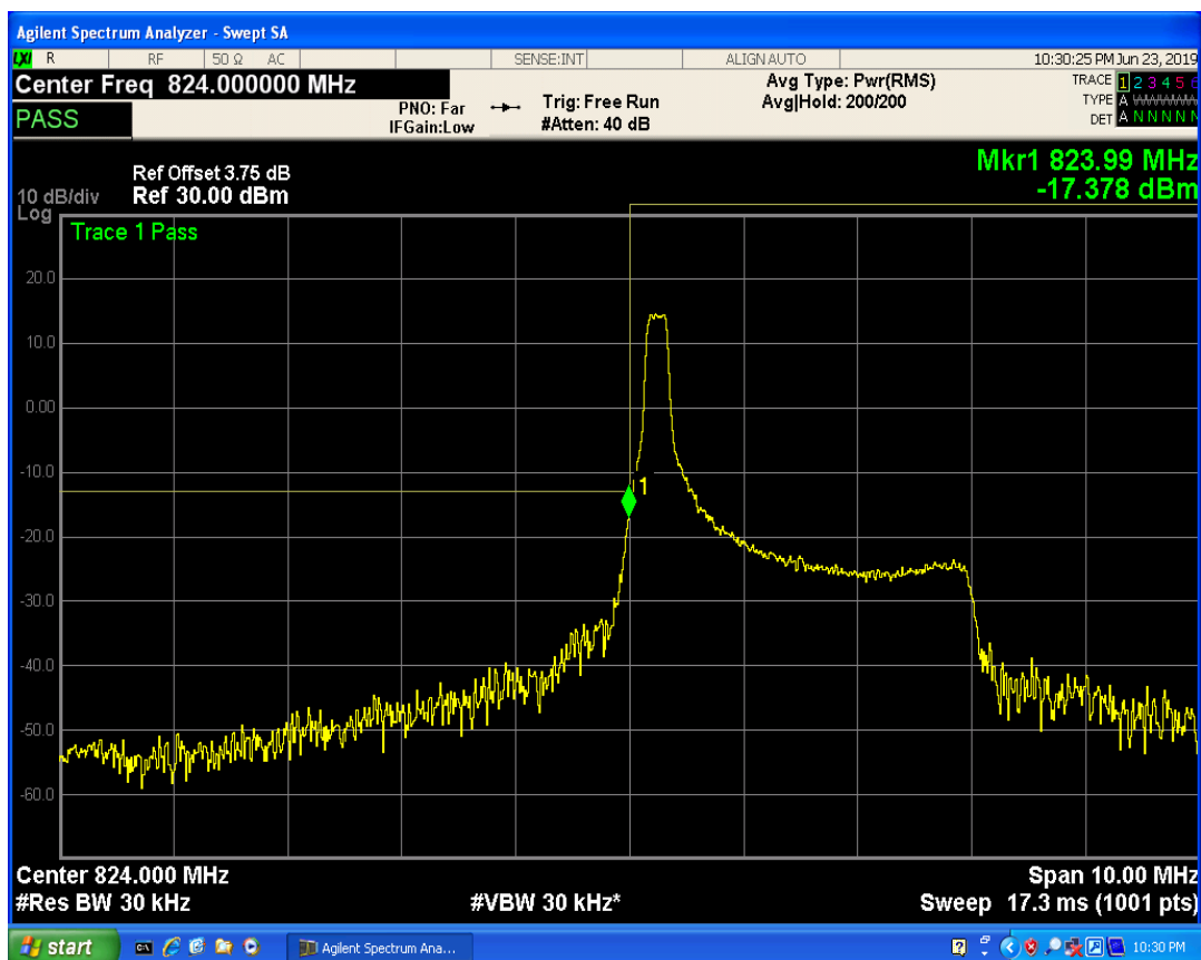
LTE Band5 QAM16 BW=3MHz Channel=20415 RB Size=1 Position=#Mid
