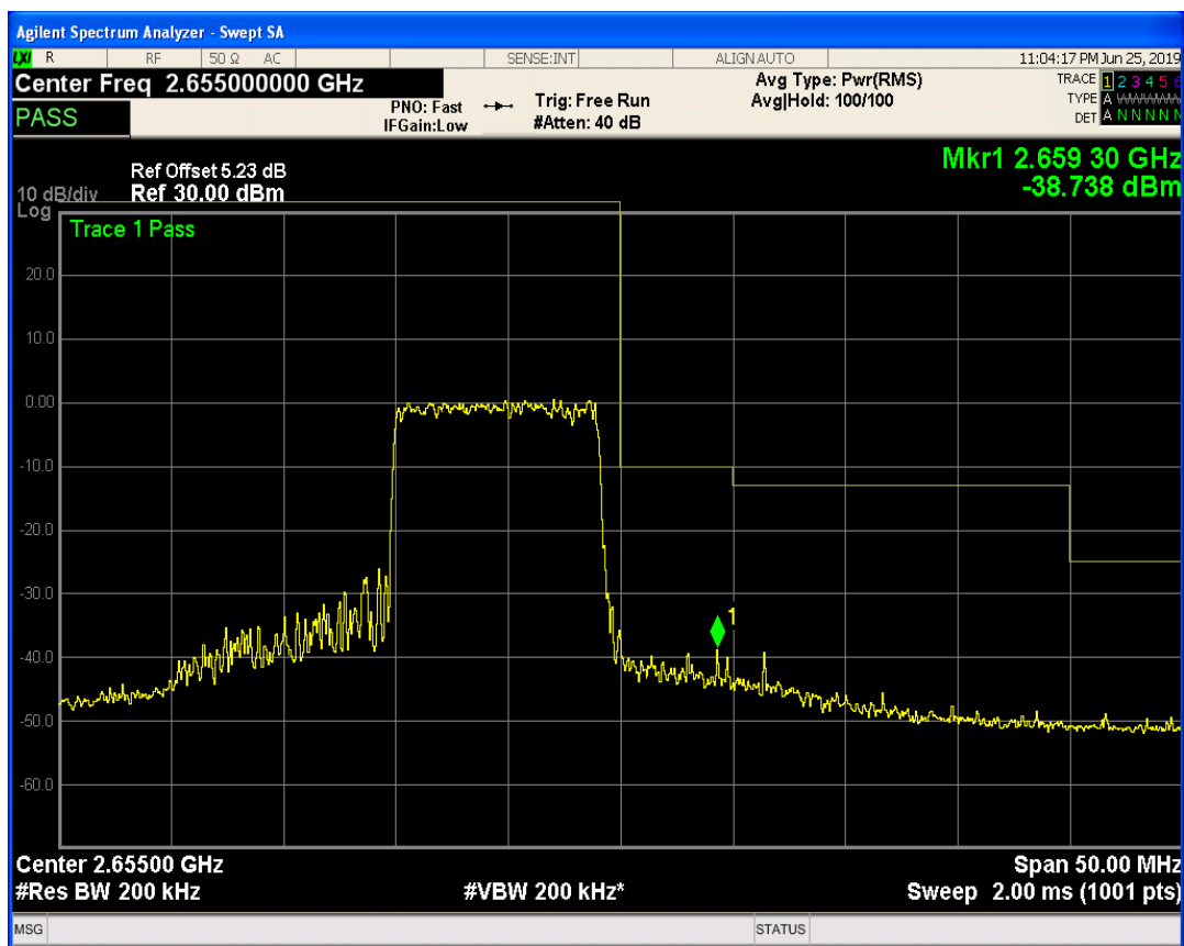
LTE Band41 QAM16 BW=20MHz Channel=41140 RB Size=1 Position=#Max
