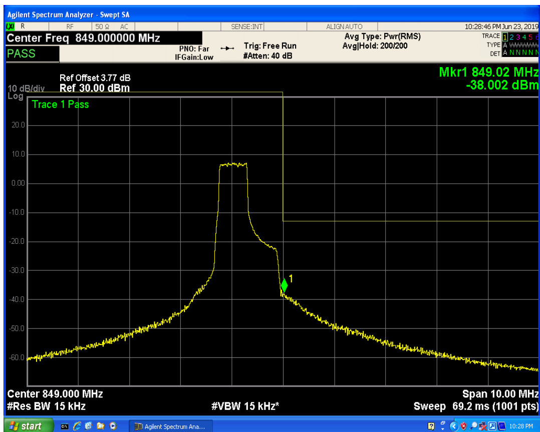
LTE Band5 QAM16 BW=1.4MHz Channel=20643 RB Size=3 Position=#Max
