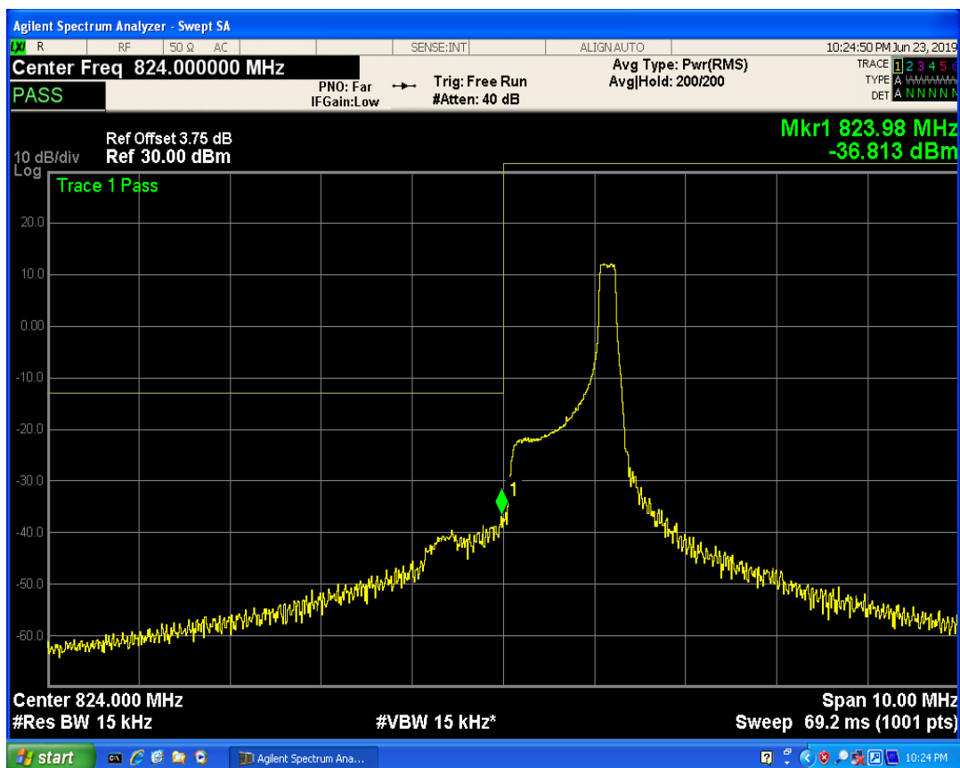
LTE Band5 QAM16 BW=1.4MHz Channel=20407 RB Size=3 Position=#Max
