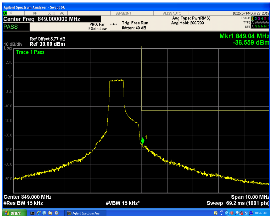
LTE Band5 QPSK BW=1.4MHz Channel=20643 RB Size=3 Position=#Max
