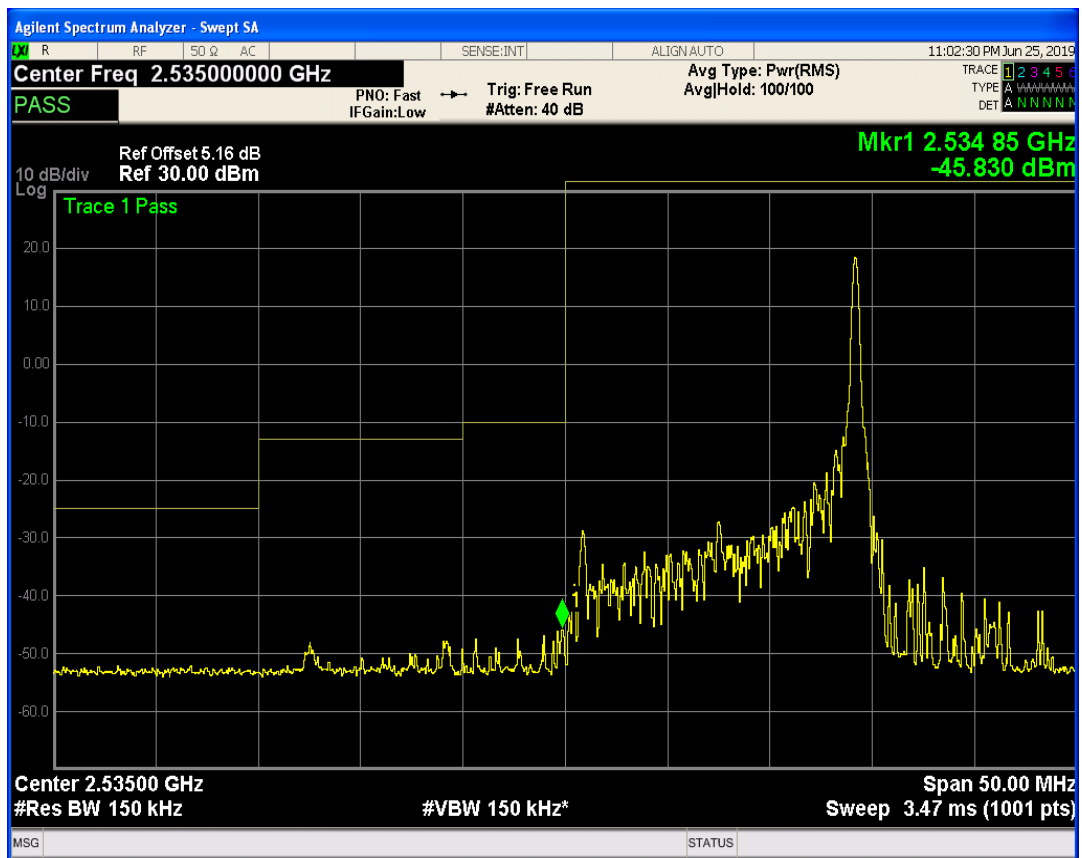
LTE Band41 QPSK BW=15MHz Channel=40115 RB Size=36 Position=#0
