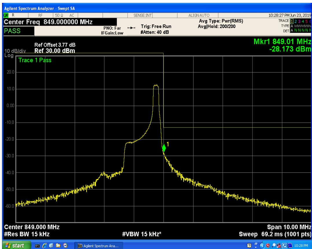
LTE Band5 QAM16 BW=1.4MHz Channel=20643 RB Size=3 Position=#0
