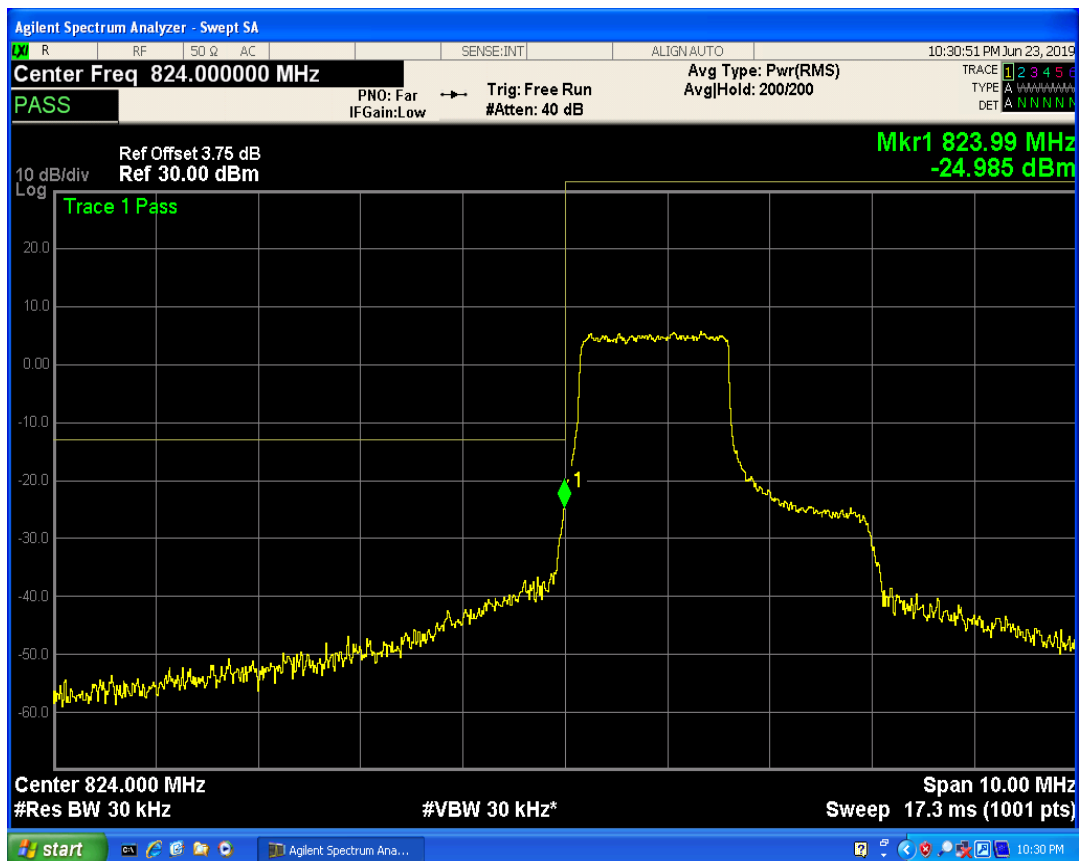
LTE Band5 QAM16 BW=3MHz Channel=20415 RB Size=8 Position=#Max
