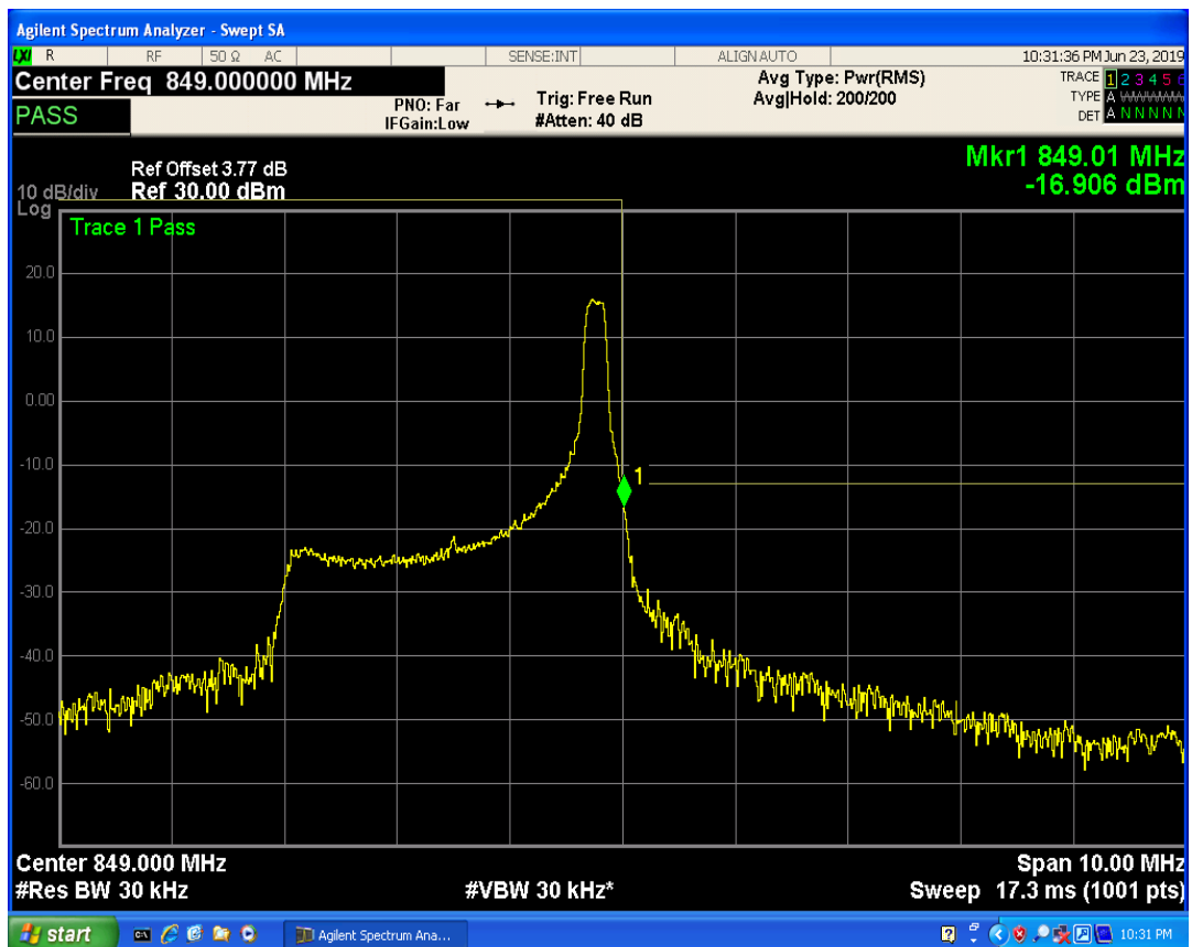
LTE Band5 QPSK BW=3MHz Channel=20635 RB Size=8 Position=#0
