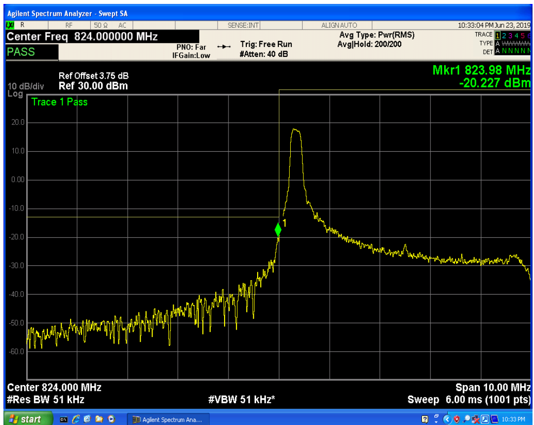
LTE Band5 QPSK BW=5MHz Channel=20425 RB Size=1 Position=#Mid
