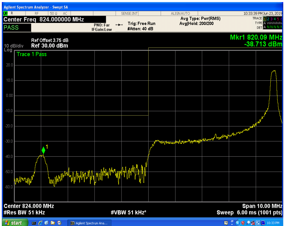
LTE Band5 QAM16 BW=5MHz Channel=20425 RB Size=12 Position=#0
