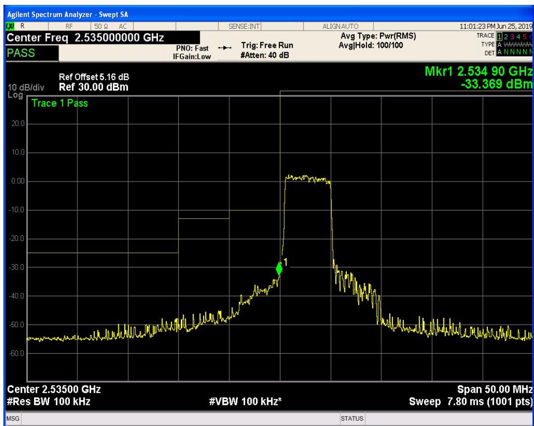
LTE Band41 QPSK BW=10MHz Channel=40090 RB Size=25 Position=#Max
