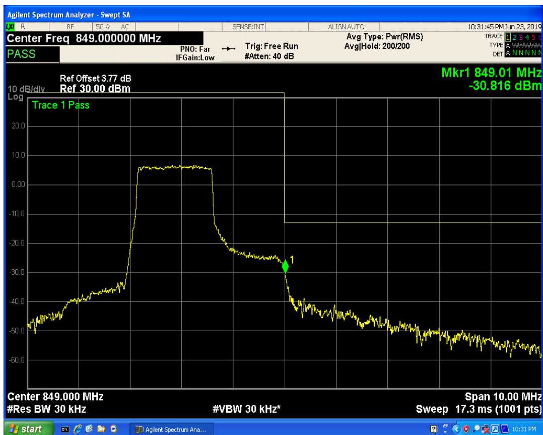
LTE Band5 QPSK BW=3MHz Channel=20635 RB Size=8 Position=#Max
