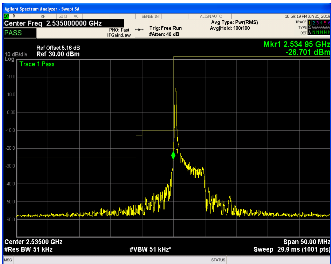
LTE Band41 QPSK BW=5MHz Channel=40065 RB Size=12 Position=#Max
