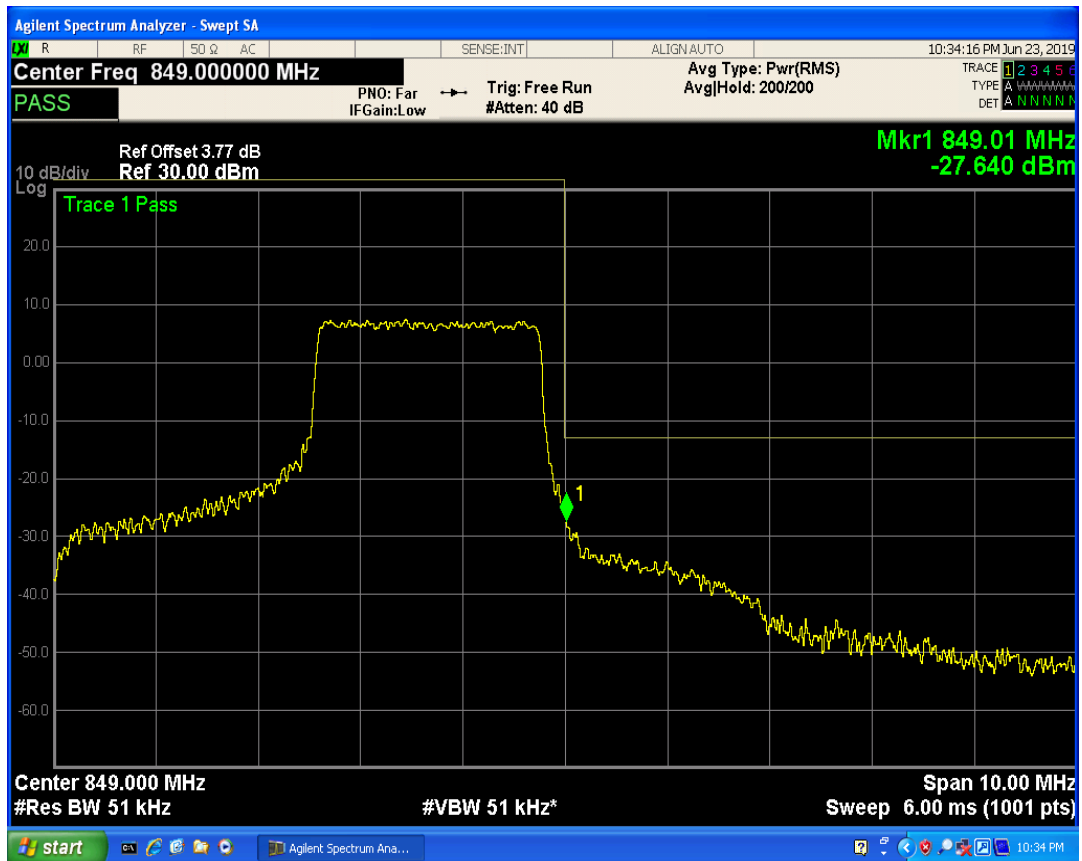
LTE Band5 QPSK BW=5MHz Channel=20625 RB Size=12 Position=#0
