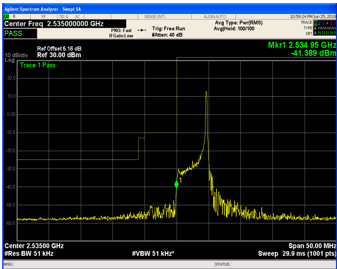
LTE Band41 QPSK BW=5MHz Channel=40065 RB Size=12 Position=#0
