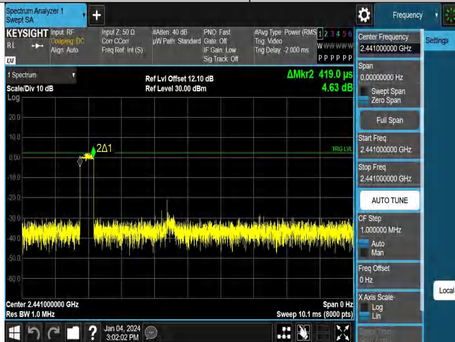
2DH1-Ant1-Hop-PASS
