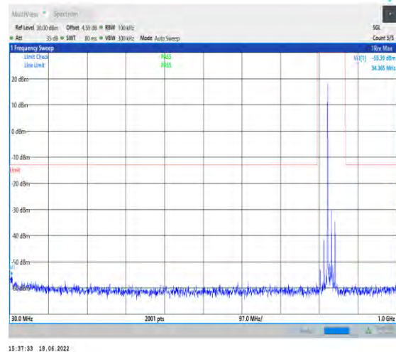
1-N5--15-20-M-1-DFT-PI2BPSK-Inner_1RB_Left-1@ 1-30-1000-Ant1--55.39--13-PASS
