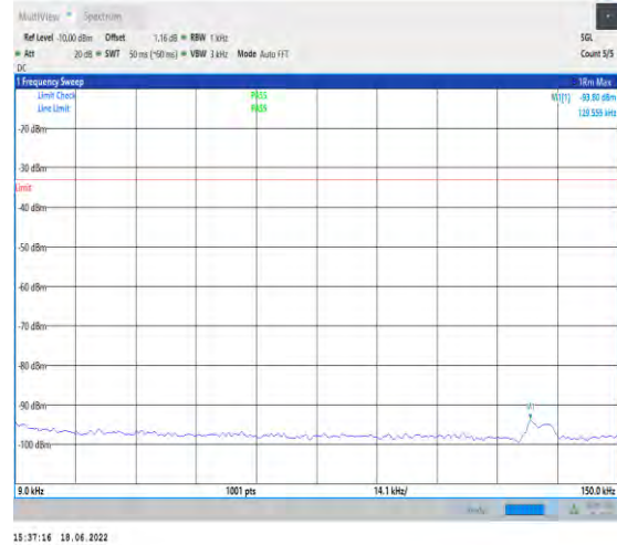
1-N5--15-20-M-1-DFT-PI2BPSK-Inner_1RB_Left-1@ 1-0.009-0.15-Ant1--93.80--33-PASS
