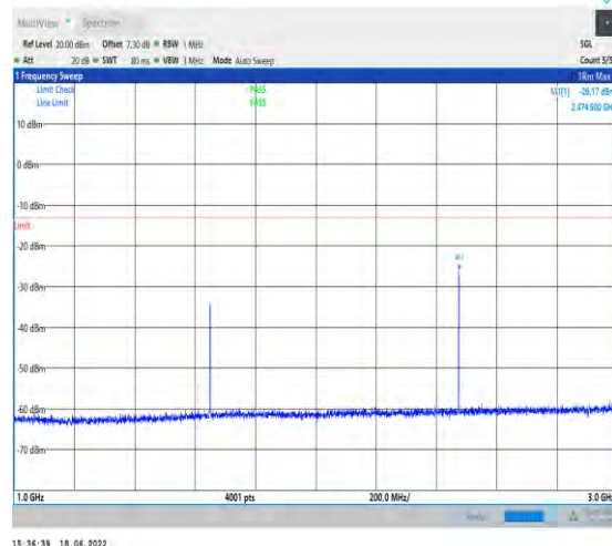
1-N5--15-20-L-1-DFT-PI2BPSK-Inner_1RB_Left-1@ 1-1000-3000-Ant1--26.17--13-PASS
