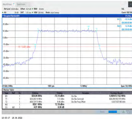
1-N5--15-5-L-3-DFT-16QAM-Outer_Full-25@0-Ant1- 4.47-4.910-≤5-PASS
