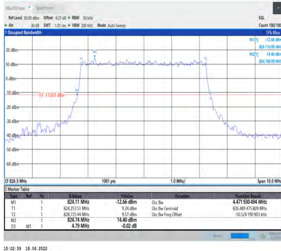
1-N5--15-5-L-1-DFT-QPSK-Outer_Full-25@0-Ant1-4 4.72-4.790-≤5-PASS
