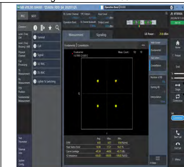
1-N5--15-20-M-6-CP-QPSK-Outer_Full-106@0-Ant 1-see graph-PASS
