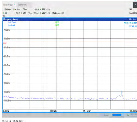
1-N5--15-20-L-1-DFT-PI2BPSK-Inner_1RB_Left-1@ 1-0.009-0.15-Ant1--93.65--33-PASS
