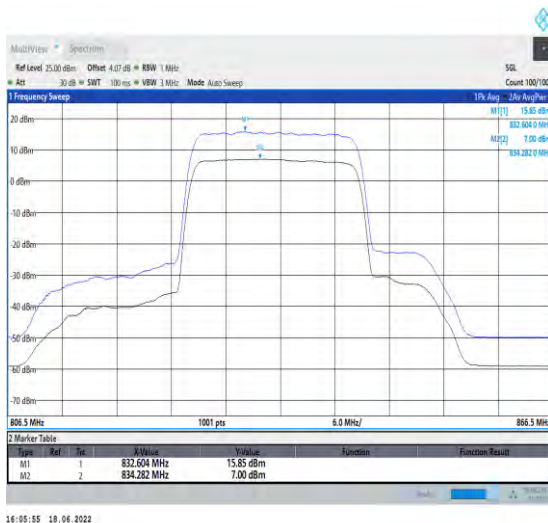
1-N5--15-20-M-1-DFT-256QAM-Outer_Full-100@0-A nt1-8.85-100%-0.00-8.85-PASS-≤13
