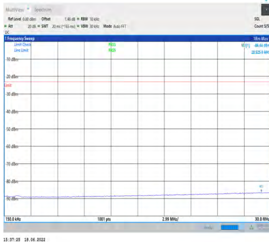
1-N5--15-20-M-1-DFT-PI2BPSK-Inner_1RB_Left-1@ 1-0.15-30-Ant1--86.44--23-PASS
