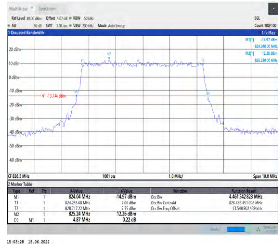
1-N5--15-5-L-4-DFT-64QAM-Outer_Full-25@0-Ant1- 4.462-4.870-≤5-PASS
