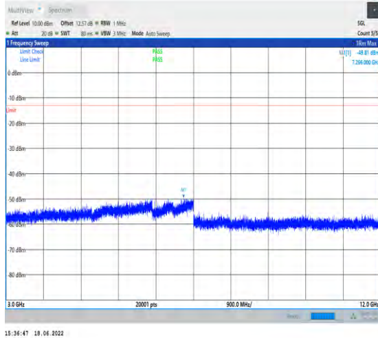
1-N5--15-20-L-1-DFT-PI2BPSK-Inner_1RB_Left-1@ 1-3000-12000-Ant1--49.81--13-PASS
