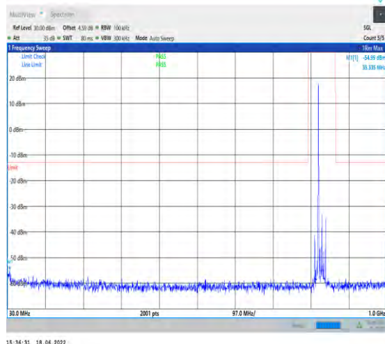
1-N5--15-20-L-1-DFT-PI2BPSK-Inner_1RB_Left-1@ 1-30-1000-Ant1--54.99--13-PASS
