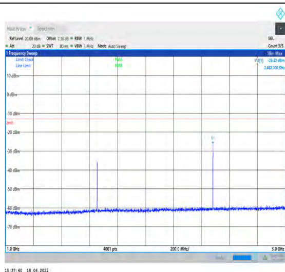
1-N5--15-20-M-1-DFT-PI2BPSK-Inner_1RB_Left-1@ 1-1000-3000-Ant1--26.42--13-PASS
