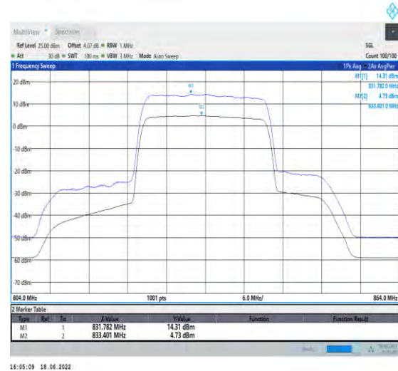
1-N5--15-20-L-2-CP-256QAM-Outer_Full-106@0-An t1-9.58-100%-0.00-9.58-PASS-≤13
