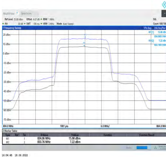
1-N5--15-20-L-1-DFT-256QAM-Outer_Full-100@0-A nt1-8.76-100%-0.00-8.76-PASS-≤13
