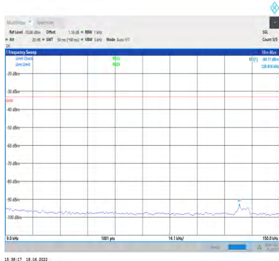
1-N5--15-20-H-1-DFT-PI2BPSK-Inner_1RB_Left-1@ 1-0.009-0.15-Ant1--94.11--33-PASS
