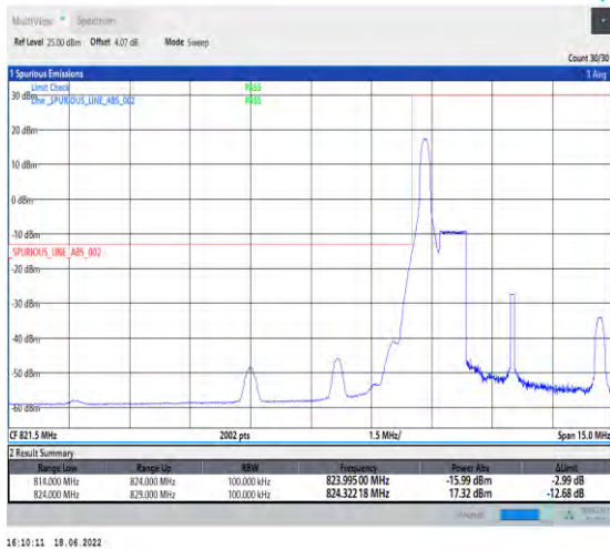
1-N5--15-5-L-4-CP-QPSK-Edge_1RB_Left-1@0-Ant1-s eegraph-PASS-see graph
