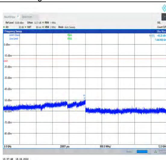
1-N5--15-20-M-1-DFT-PI2BPSK-Inner_1RB_Left-1@ 1-3000-12000-Ant1--49.25--13-PASS
