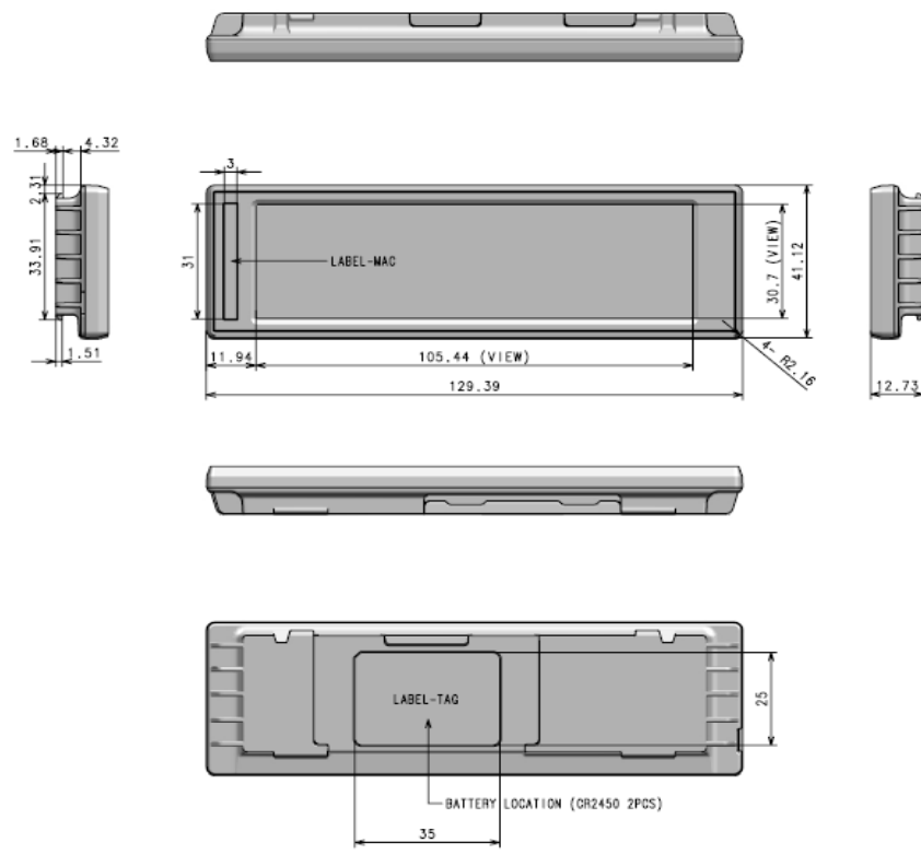
Figure 3 Mechanical Dimension
