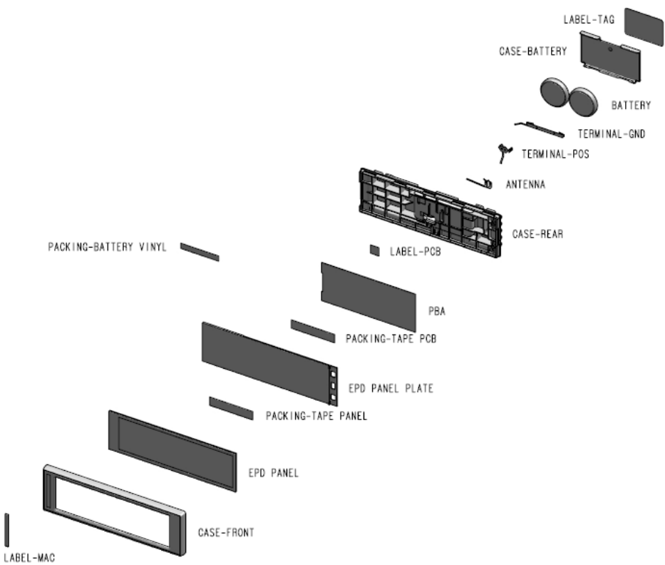
Figure 4 Exploded View
