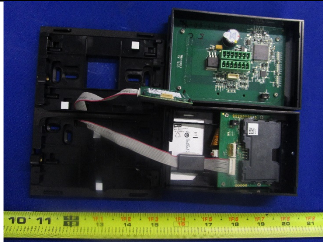
Cover off View 1 with PCBA2
