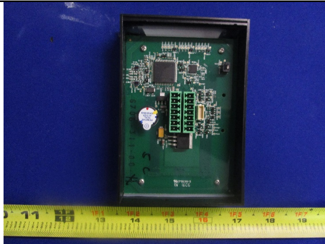
Cover off View 3 without PCBA2
