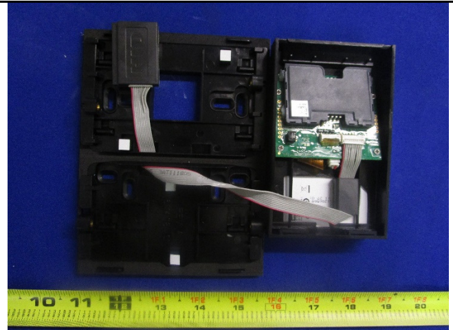
Cover off View 4 PCBA2
