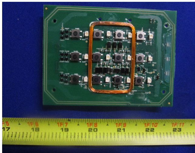
PCBA 1 Top View 1 without PCBA2
