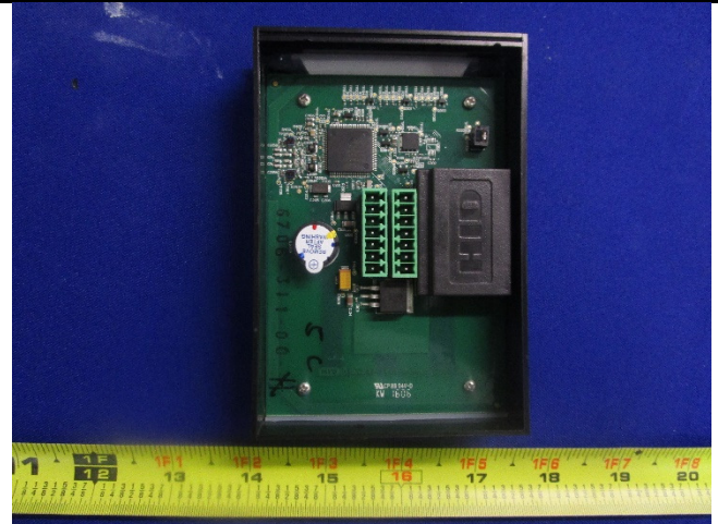
Cover off View 2 with PCBA2
