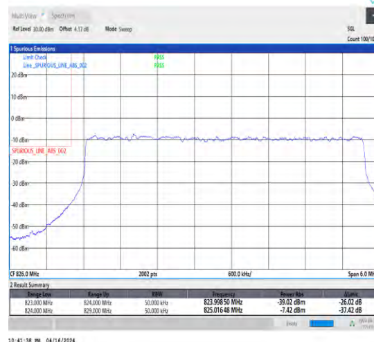
1-N5-15-5-L-3-DFT-PI2BPSK-Outer_Full-25@0-Ant1-1-seegraph-PASS-see graph
