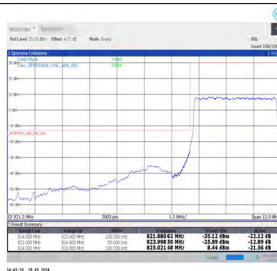
1-N5-15-5-L-3-DFT-PI2BPSK-Outer_Full-25@0-A nt1-1--PASS-see graph
