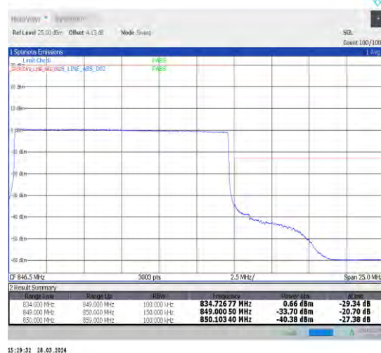
1-N5-15-15-H-6-CP-QPSK-Outer_Full-79@0-Ant1 -1--PASS-see graph
