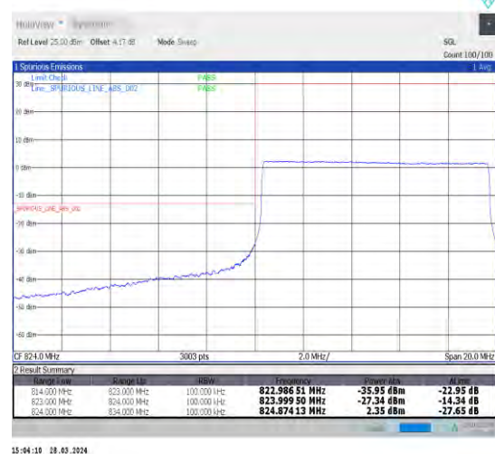
1-N5-15-10-L-6-CP-QPSK-Outer_Full-52@0-A nt1-1--PASS-see graph
