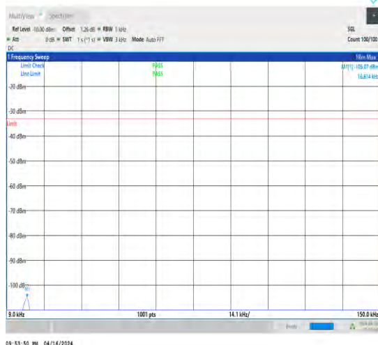
1-N5-15-20-L-1-DFT-QPSK-Edge_1RB_Left-1@0-0. 009-0.15-Ant1-0.02--105.07--33-PASS
