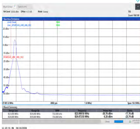
1-N5-15-15-L-4-CP-QPSK-Edge_1RB_Left-1@0-Ant1-1-seegraph-PASS-see graph
