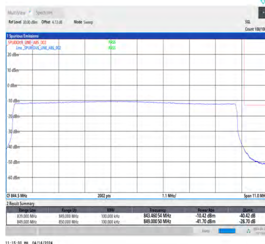
1-N5-15-10-H-6-CP-QPSK-Outer_Full-52@0-Ant1 -1-seegraph-PASS-see graph
