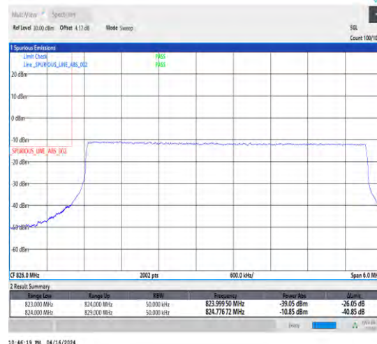
1-N5-15-5-L-6-CP-QPSK-Outer_Full-25@0-Ant1-1-seegraph-PASS-see graph
