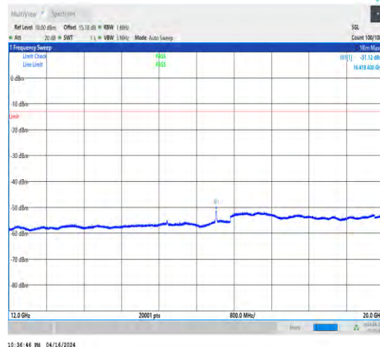
1-N5-15-20-H-1-DFT-QPSK-Edge_1RB_Left-1@0-12 000-20000-Ant1-16418.40--51.12--13-PASS
