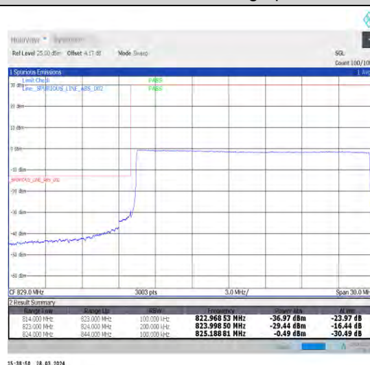
1-N5-15-20-L-6-CP-QPSK-Outer_Full-106@0-Ant 1-1--PASS-see graph
