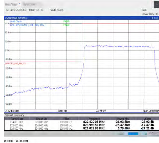
1-N5-15-10-L-3-DFT-PI2BPSK-Outer_Full-50@0-A Ant1-1--PASS-see graph
