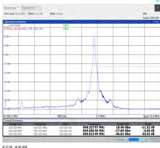
1-N5-15-15-H-5-CP-QPSK-Edge_1RB_Right-1@78-An t1-1--PASS-see graph
