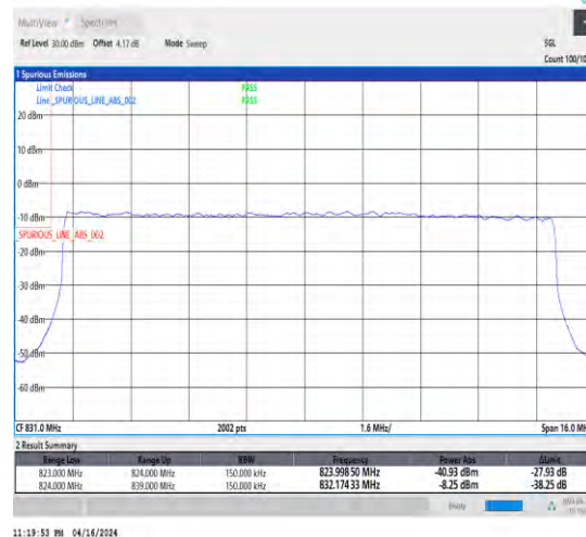
1-N5-15-15-L-3-DFT-PI2BPSK-Outer_Full-75@0-Ant1-1-seegraph-PASS-see graph
