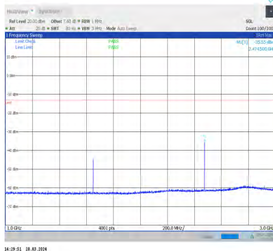
1-N5-15-20-L-1-DFT-PI2BPSK-Inner_1RB_Left-1@1 -1000-3000-Ant1-2474.50--35.55--13-PASS
