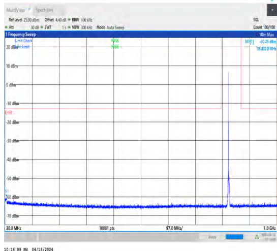
1-N5-15-20-M-1-DFT-QPSK-Edge_1RB_Left-1@0-3 0-1000-Ant1-35.43--60.25--13-PASS
