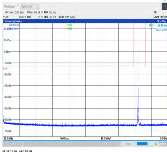
1-N5-15-20-L-1-DFT-QPSK-Edge_1RB_Left-1@0-3 0-1000-Ant1-32.23--60.58--13-PASS
