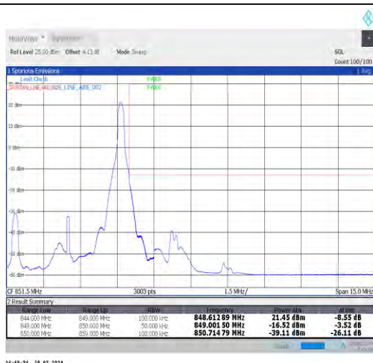
1-N5-15-5-H-2-DFT-PI2BPSK-Edge_1RB_Right-1@24-Ant1-1--PASS-see graph
