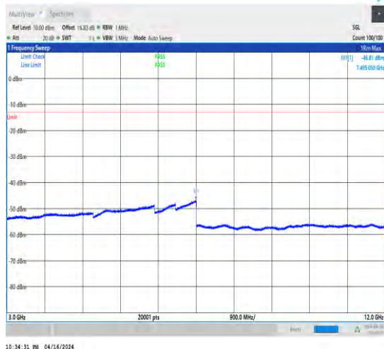
1-N5-15-20-H-1-DFT-QPSK-Edge_1RB_Left-1@0-3 000-12000-Ant1-7495.05--46.81--13-PASS
