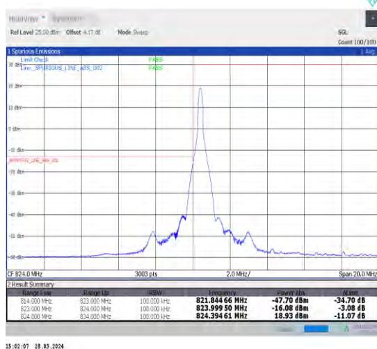
1-N5-15-10-L-4-CP-QPSK-Edge_1RB_Left-1@0-A nt1-1--PASS-see graph
