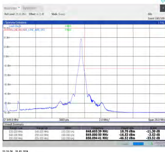
1-N5-15-10-H-5-CP-QPSK-Edge_1RB_Right-1@51-An t1-1--PASS-see graph
