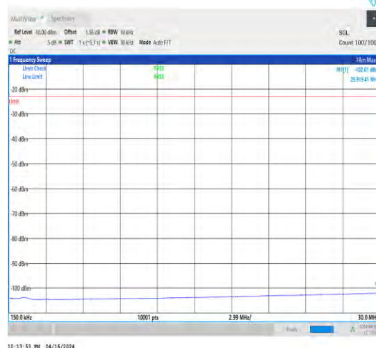
1-N5-15-20-M-1-DFT-QPSK-Edge_1RB_Left-1@0-0. 15-30-Ant1-29.92--102.01--23-PASS
