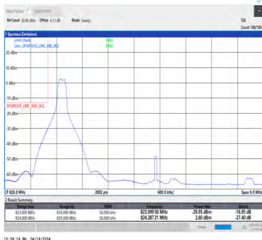
1-N5-15-5-L-1-DFT-PI2BPSK-Edge_1RB_Left-1@0-Ant1-1-seegraph-PASS-see graph
