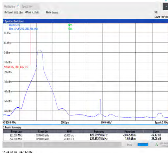
1-N5-15-5-L-4-CP-QPSK-Edge_1RB_Left-1@0-Ant1-1-seegraph-PASS-see graph
