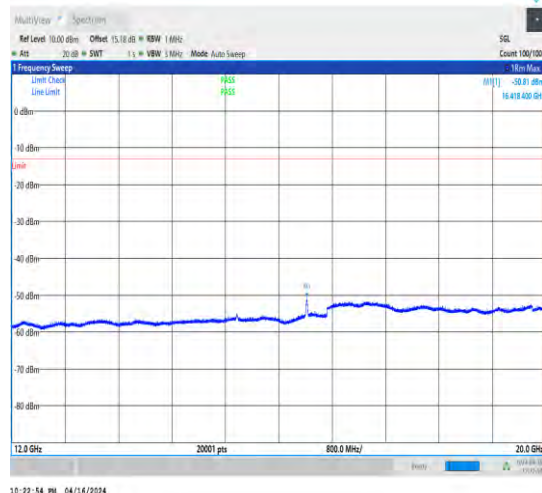
1-N5-15-20-M-1-DFT-QPSK-Edge_1RB_Left-1@0-12 000-20000-Ant1-16418.40--50.81--13-PASS
