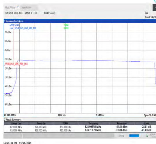
1-N5-15-15-L-6-CP-QPSK-Outer_Full-79@0-Ant1-1-seegraph-PASS-see graph
