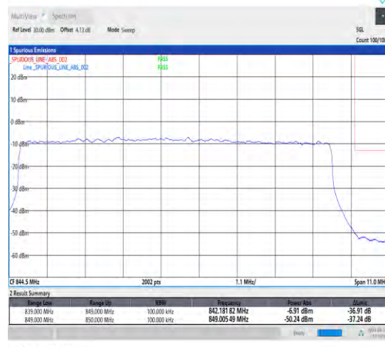
1-N5-15-10-H-3-DFT-PI2BPSK-Outer_Full-50@0- Ant1-1-seegraph-PASS-see graph
