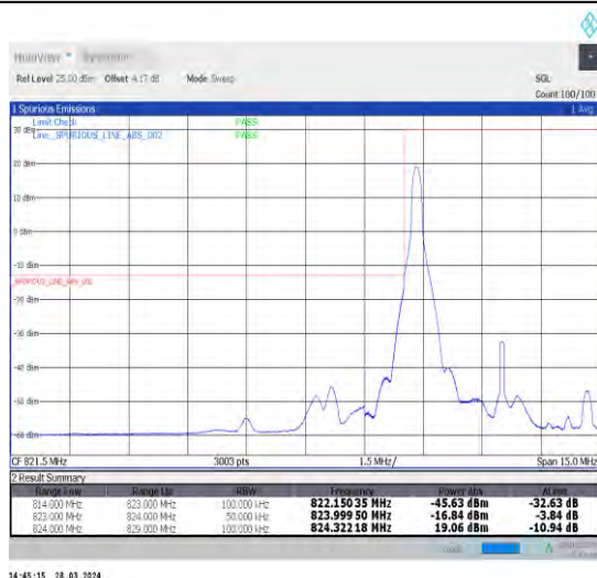
1-N5-15-5-L-4-CP-QPSK-Edge_1RB_Left-1@0-Ant1-1- -PASS-see graph
