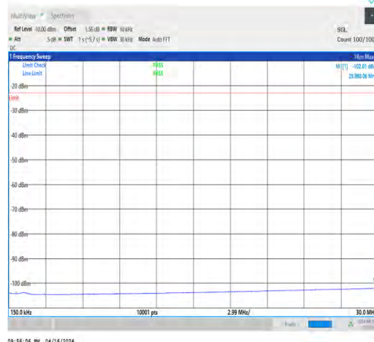
1-N5-15-20-L-1-DFT-QPSK-Edge_1RB_Left-1@0-0.1 5-30-Ant1-29.99--102.01--23-PASS
