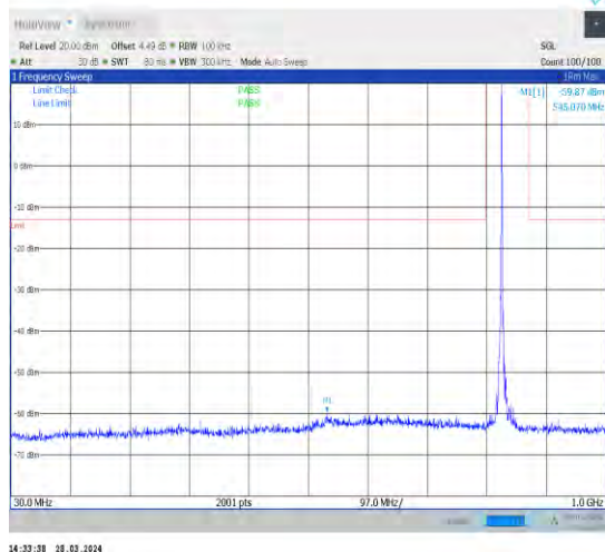
1-N5-15-20-H-1-DFT-PI2BPSK-Inner_1RB_Left-1@1 -30-1000-Ant1-545.07--59.87--13-PASS
