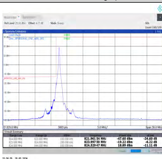
1-N5-15-20-L-4-CP-QPSK-Edge_1RB_Left-1@0-Ant1-1--PASS-see graph
