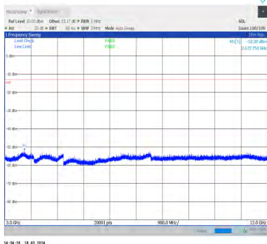
1-N5-15-20-H-1-DFT-PI2BPSK-Inner_1RB_Left-1@1 -3000-12000-Ant1-3672.75--52.30--13-PASS
