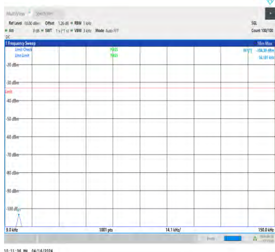
1-N5-15-20-M-1-DFT-QPSK-Edge_1RB_Left-1@0-0 .009-0.15-Ant1-0.02--104.39--33-PASS
