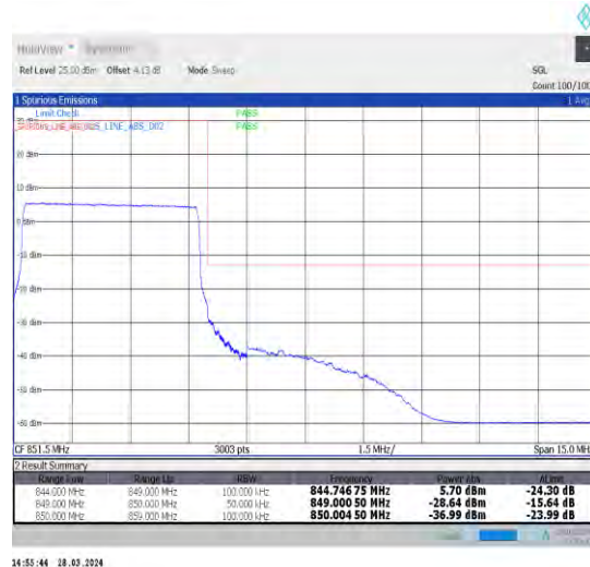
1-N5-15-5-H-6-CP-QPSK-Outer_Full-25@0-Ant1-1--PASS-see graph
