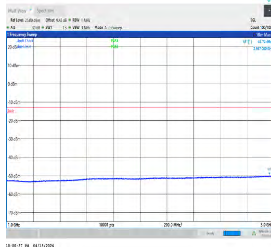
1-N5-15-20-L-1-DFT-QPSK-Edge_1RB_Left-1@0-10 00-3000-Ant1-2967.00--49.72--13-PASS
