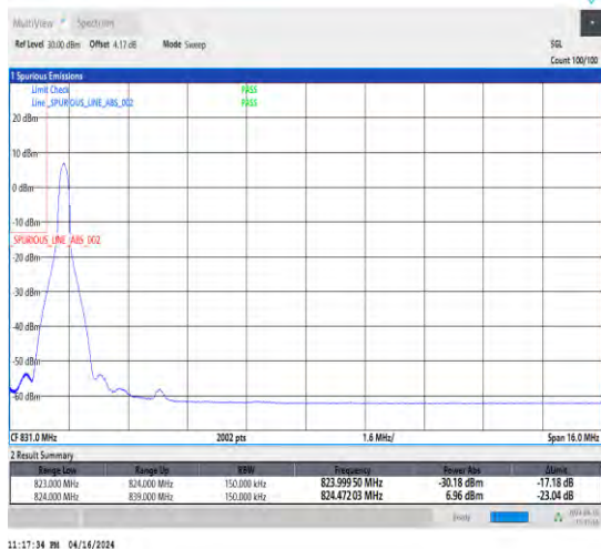
1-N5-15-15-L-1-DFT-PI2BPSK-Edge_1RB_Left-1@0-Ant1-1-seegraph-PASS-see graph
