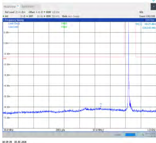
1-N5-15-20-L-1-DFT-PI2BPSK-Inner_1RB_Left-1@1 -30-1000-Ant1-649.35--60.29--13-PASS
