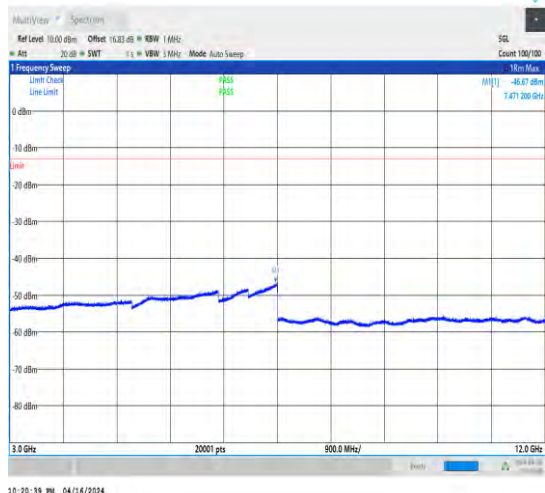
1-N5-15-20-M-1-DFT-QPSK-Edge_1RB_Left-1@0-3 000-12000-Ant1-7471.20--46.67--13-PASS
