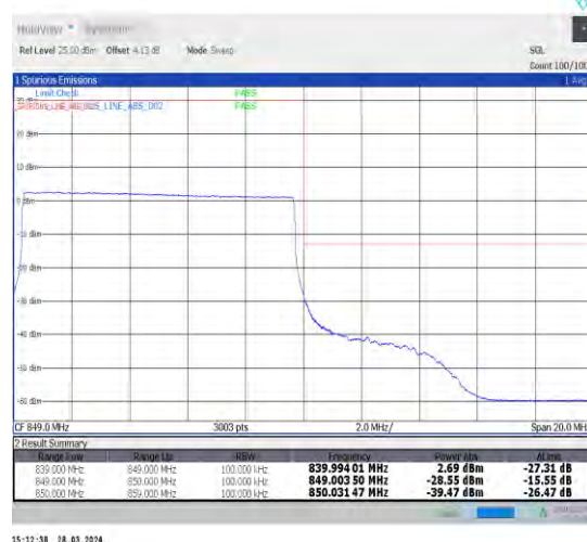
1-N5-15-10-H-6-CP-QPSK-Outer_Full-52@0-Ant1 -1--PASS-see graph
