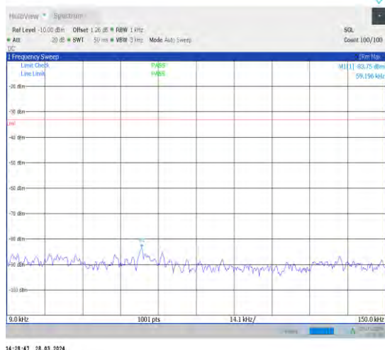
1-N5-15-20-L-1-DFT-PI2BPSK-Inner_1RB_Left-1@1 -0.009-0.15-Ant1-0.06--83.75--33-PASS
