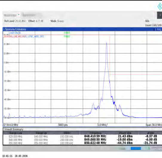
1-N5-15-20-H-2-DFT-PI2BPSK-Edge_1RB_Right-1@105-Ant1-1--PASS-see graph
