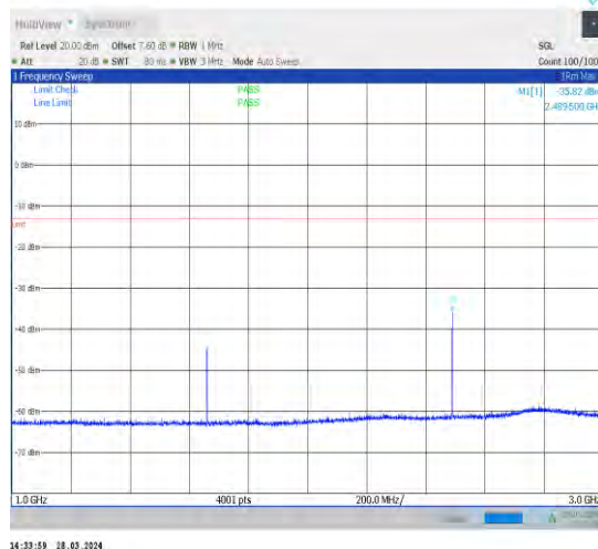
1-N5-15-20-H-1-DFT-PI2BPSK-Inner_1RB_Left-1@1 -1000-3000-Ant1-2489.50--35.82--13-PASS
