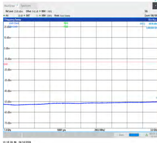
1-N5-15-20-M-1-DFT-QPSK-Edge_1RB_Left-1@0-10 00-3000-Ant1-3000.00--49.94--13-PASS
