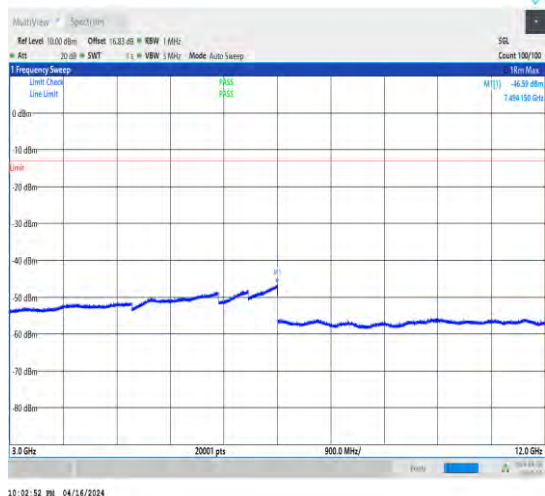
1-N5-15-20-L-1-DFT-QPSK-Edge_1RB_Left-1@0-3 000-12000-Ant1-7494.15--46.59--13-PASS
