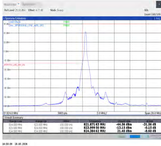
1-N5-15-10-L-1-DFT-PI2BPSK-Edge_1RB_Left-1@0-A nt1-1--PASS-see graph
