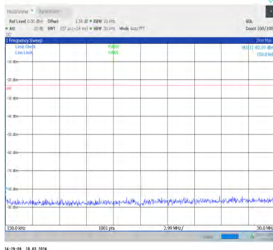
1-N5-15-20-L-1-DFT-PI2BPSK-Inner_1RB_Left-1@1 -0.15-30-Ant1-0.15--82.97--23-PASS
