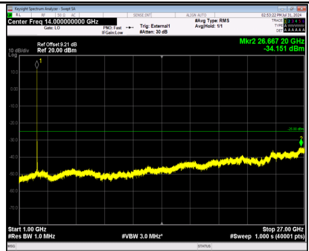
41-41-5MHz-20MHz-64QAM-64QAM-41023-41140-1RB# 0-1RB#99-1000~27000MHz-PASS
