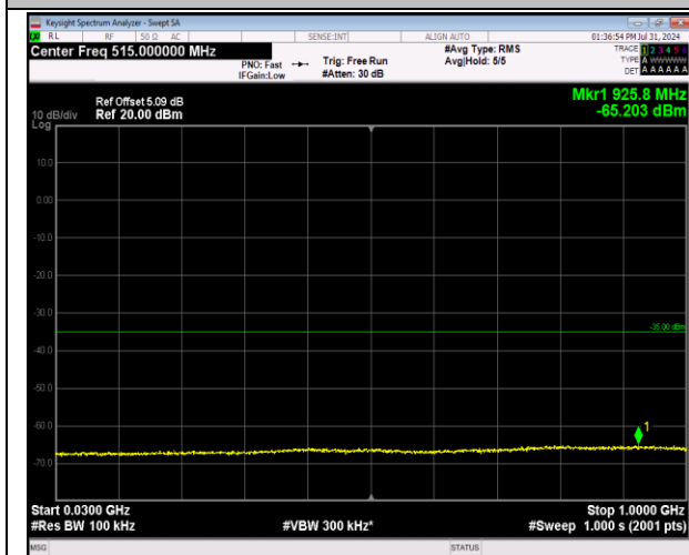
7-7-20MHz-20MHz-64QAM-64QAM-21152-21350-1RB# 99-0RB#0-30~1000MHz-PASS
