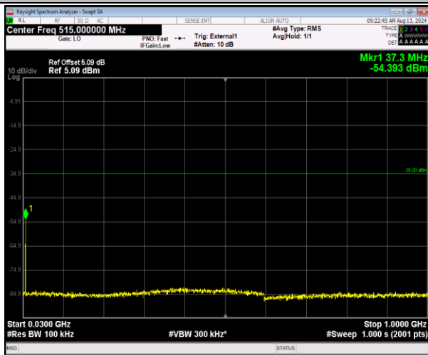
41-41-5MHz-20MHz-QPSK-QPSK-40648-40765-1RB#2-4-ORB#0-30~1000MHz-PASS
