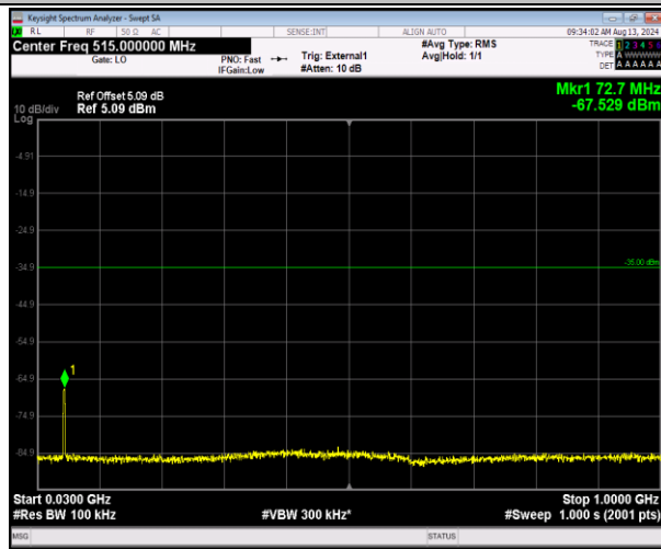
41-41-5MHz-20MHz-16QAM-16QAM-41023-41140-25R B#0-100RB#0-30~1000MHz-PASS
