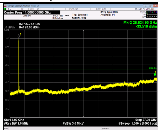
41-41-5MHz-20MHz-64QAM-64QAM-40273-40390-1RB# 0-1RB#99-1000~27000MHz-PASS
