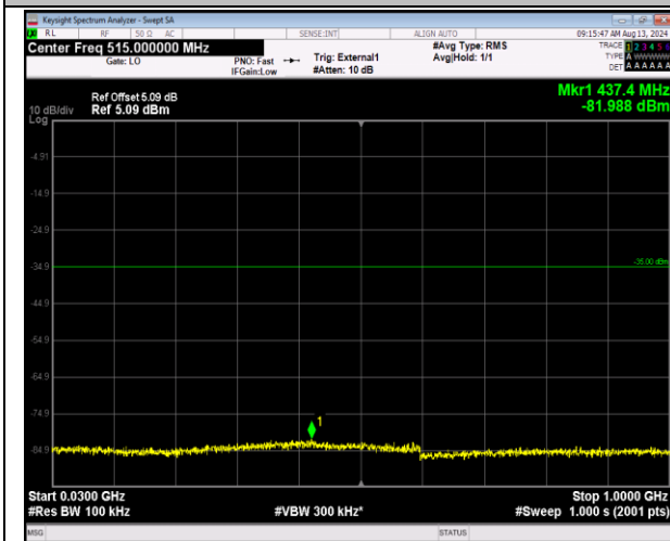
41-41-5MHz-20MHz-QPSK-QPSK-40273-40390-1RB#2-4-ORB#0-30~1000MHz-PASS
