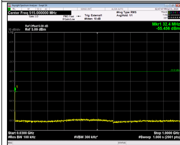
41-41-5MHz-20MHz-64QAM-64QAM-40648-40765-1RB #0-ORB#0-30~1000MHz-PASS
