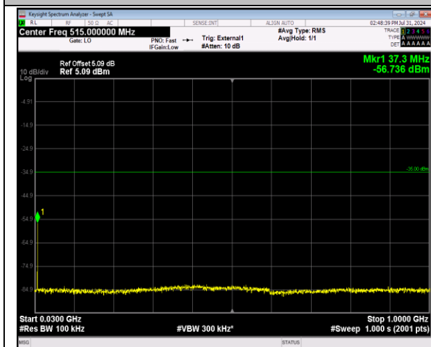
41-41-5MHz-20MHz-64QAM-64QAM-40648-40765-1RB #24-0RB#0-30~1000MHz-PASS
