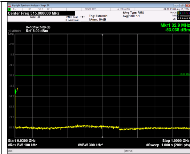
41-41-5MHz-20MHz-QPSK-QPSK-40648-40765-1RB#0-ORB#0-30~1000MHz-PASS
