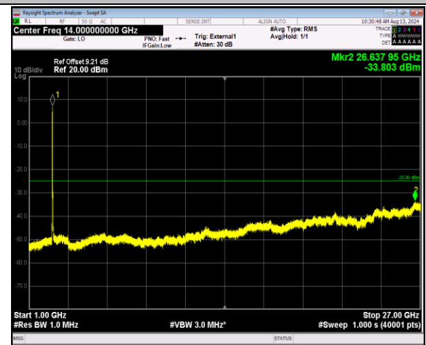
41-41-20MHz-5MHz-16QAM-16QAM-40340-40457-100R B#0-25RB#0-1000~27000MHz-PASS
