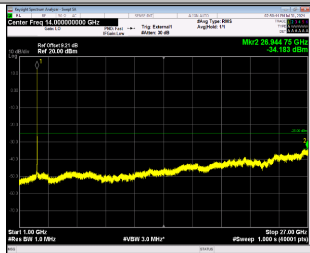
41-41-5MHz-20MHz-64QAM-64QAM-40648-40765-25R B#0-100RB#0-1000~27000MHz-PASS
