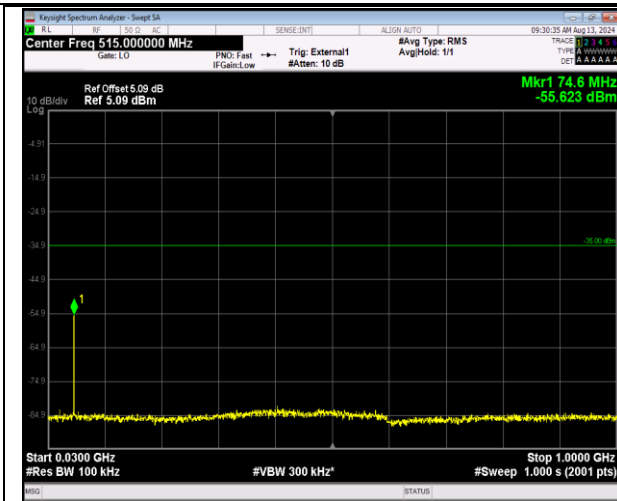
41-41-5MHz-20MHz-16QAM-16QAM-41023-41140-1RB #24-ORB#0-30~1000MHz-PASS
