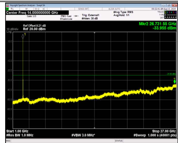
41-41-5MHz-20MHz-16QAM-16QAM-41023-41140-1RB# 0-1RB#99-1000~27000MHz-PASS
