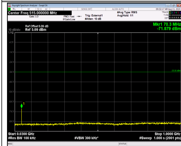
41-41-5MHz-20MHz-16QAM-16QAM-41023-41140-1RB #0-1RB#99-30~1000MHz-PASS
