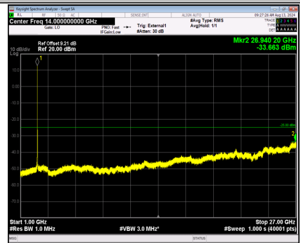
41-41-5MHz-20MHz-16QAM-16QAM-40648-40765-25RB #0-100RB#0-1000~27000MHz-PASS
