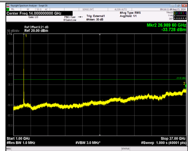
41-41-5MHz-20MHz-QPSK-QPSK-40273-40390-1RB#24-ORB#0-1000~27000MHz-PASS
