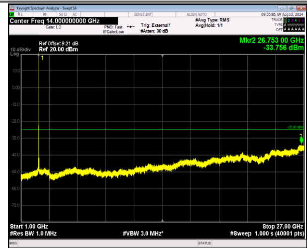
41-41-5MHz-20MHz-QPSK-QPSK-41023-41140-1RB#24- ORB#0-1000~27000MHz-PASS
