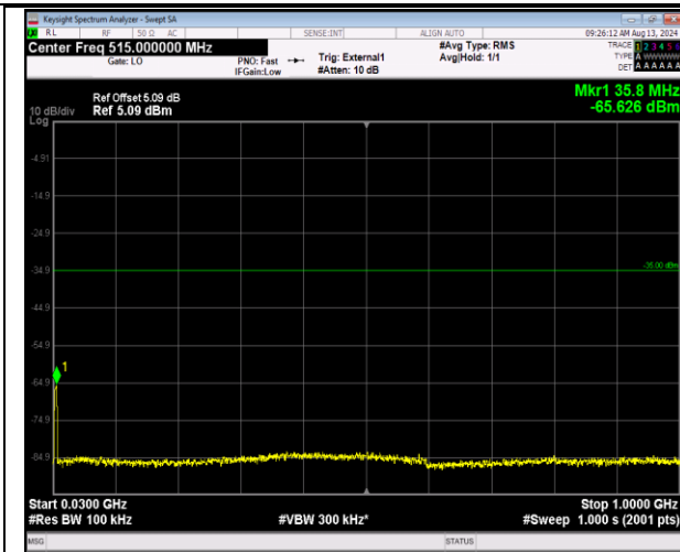
41-41-5MHz-20MHz-QPSK-QPSK-40648-40765-25RB# 0-100RB#0-30~1000MHz-PASS
