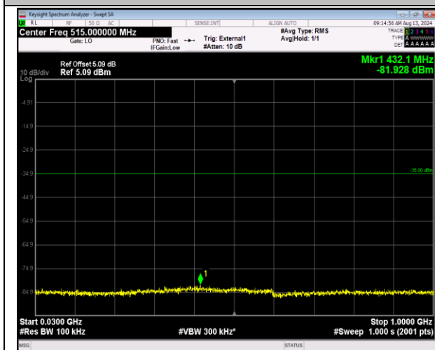
41-41-5MHz-20MHz-16QAM-16QAM-40273-40390-1RB #0-0RB#0-30~1000MHz-PASS
