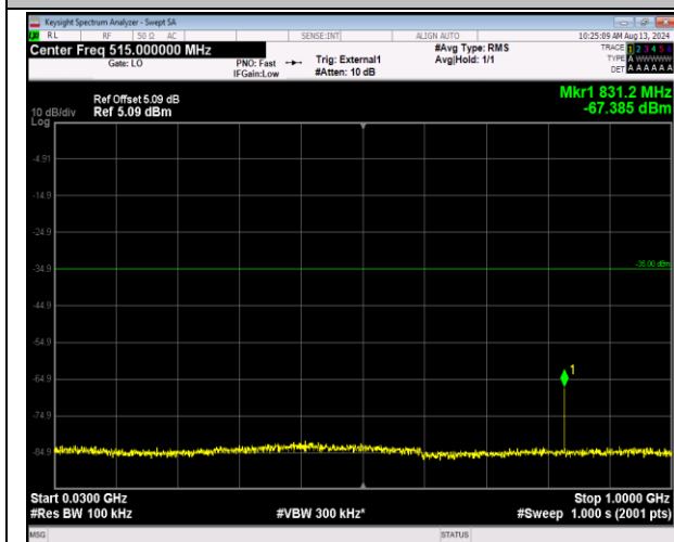
41-41-20MHz-5MHz-16QAM-16QAM-40340-40457-1RB #0-0RB#0-30~1000MHz-PASS
