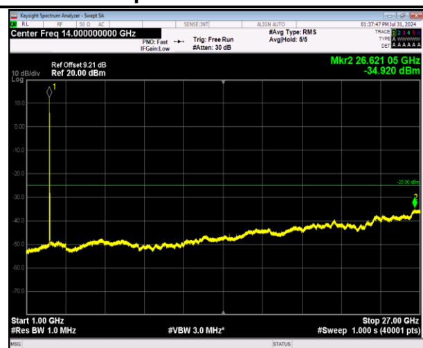
7-7-20MHz-20MHz-64QAM-64QAM-21152-21350-1RB#0- 1RB#99-1000~27000MHz-PASS
