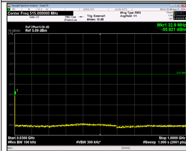
41-41-5MHz-20MHz-16QAM-16QAM-40648-40765-1RB #0-0RB#0-30~1000MHz-PASS
