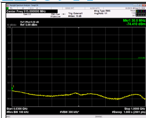
41-41-20MHz-5MHz-QPSK-QPSK-40340-40457-100RB #0-25RB#0-30~1000MHz-PASS
