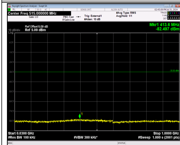
41-41-5MHz-20MHz-64QAM-64QAM-40273-40390-1RB #24-0RB#0-30~1000MHz-PASS
