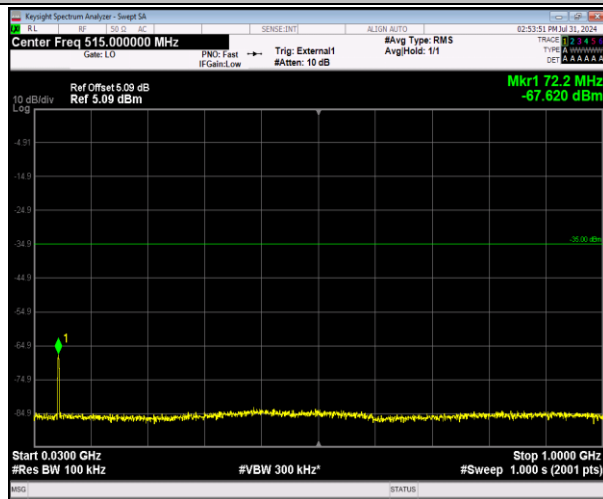
41-41-5MHz-20MHz-64QAM-64QAM-41023-41140-25R B#0-100RB#0-30~1000MHz-PASS
