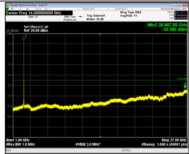
41-41-5MHz-20MHz-16QAM-16QAM-41023-41140-25RB #0-100RB#0-1000~27000MHz-PASS
