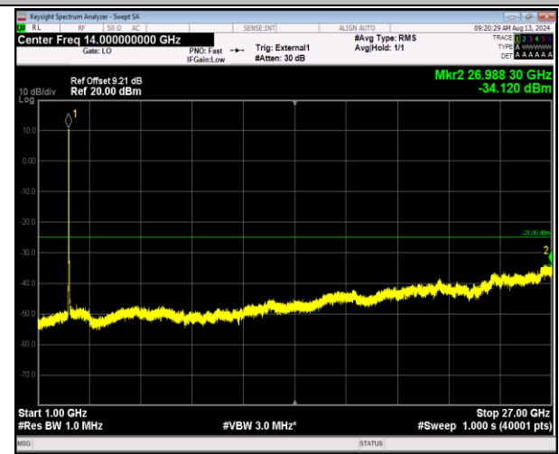
41-41-5MHz-20MHz-16QAM-16QAM-40273-40390-25RB #0-100RB#0-1000~27000MHz-PASS
