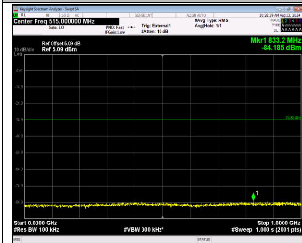
41-41-20MHz-5MHz-16QAM-16QAM-40340-40457-1RB #0-1RB#24-30~1000MHz-PASS
