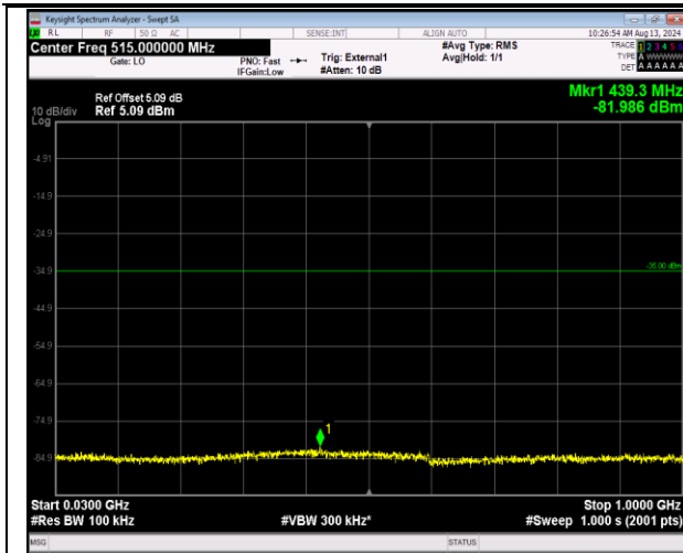
41-41-20MHz-5MHz-16QAM-16QAM-40340-40457-1RB #99-ORB#0-30~1000MHz-PASS
