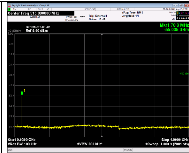
41-41-5MHz-20MHz-QPSK-QPSK-41023-41140-1RB#0- ORB#0-30~1000MHz-PASS
