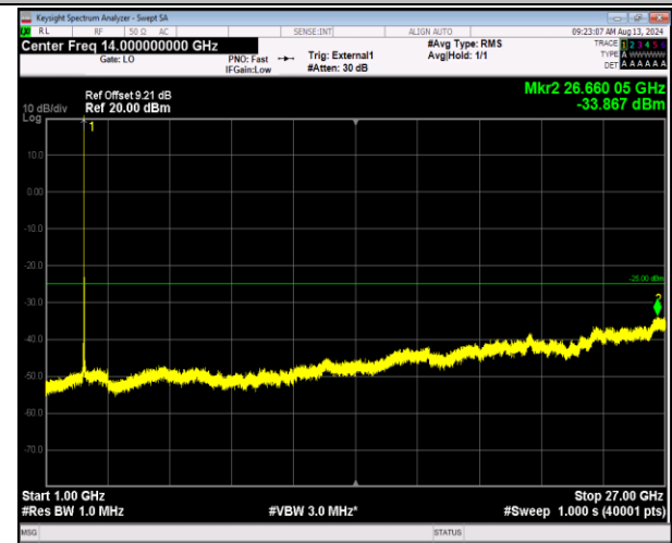
41-41-5MHz-20MHz-QPSK-QPSK-40648-40765-1RB#24-ORB#0-1000~27000MHz-PASS
