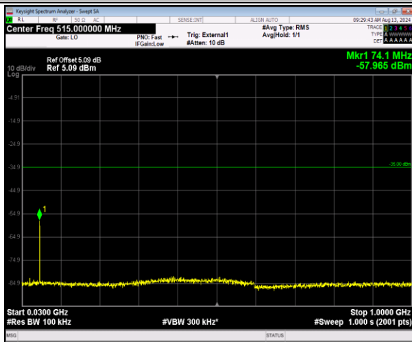
41-41-5MHz-20MHz-QPSK-QPSK-41023-41140-1RB#24 -ORB#0-30~1000MHz-PASS
