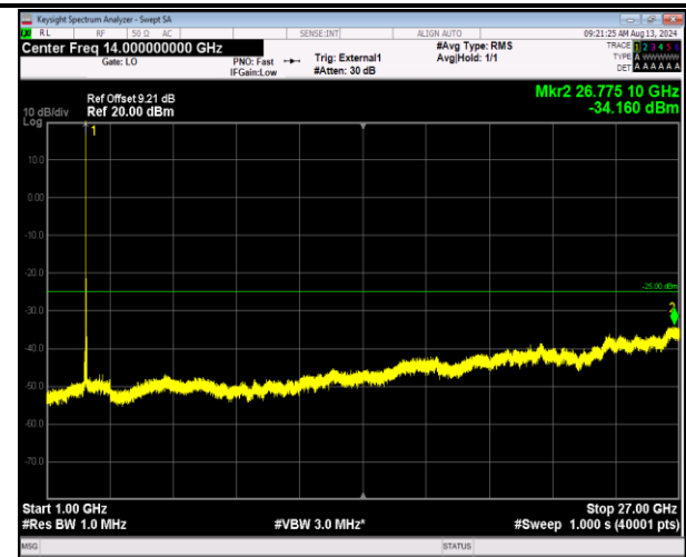
41-41-5MHz-20MHz-QPSK-QPSK-40648-40765-1RB#0-ORB#0-1000~27000MHz-PASS
