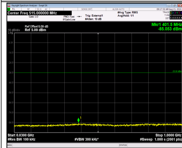
41-41-5MHz-20MHz-QPSK-QPSK-40273-40390-1RB#0-1RB#99-30~1000MHz-PASS
