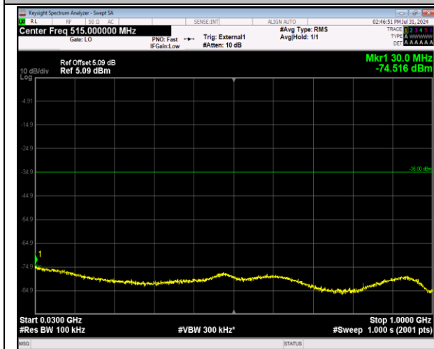
41-41-5MHz-20MHz-64QAM-64QAM-40273-40390-25R B#0-100RB#0-30~1000MHz-PASS
