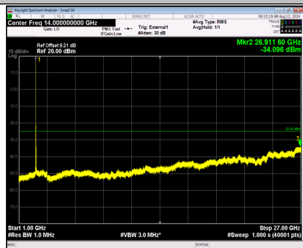
41-41-5MHz-20MHz-16QAM-16QAM-40273-40390-1RB# 0-0RB#0-1000~27000MHz-PASS
