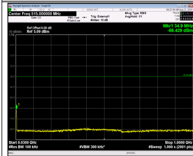
41-41-5MHz-20MHz-16QAM-16QAM-40648-40765-25R B#0-100RB#0-30~1000MHz-PASS
