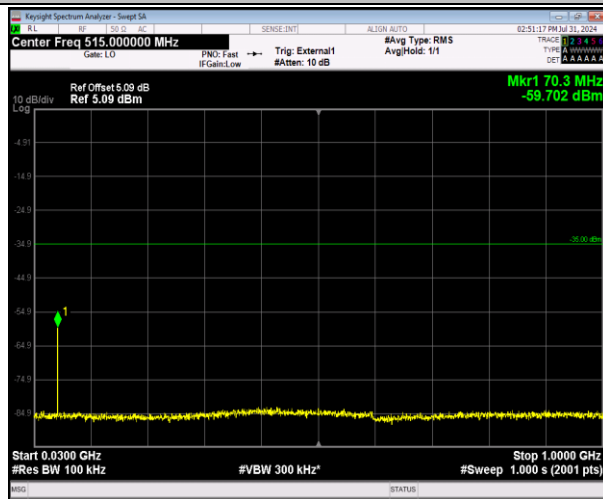
41-41-5MHz-20MHz-64QAM-64QAM-41023-41140-1RB #0-ORB#0-30~1000MHz-PASS
