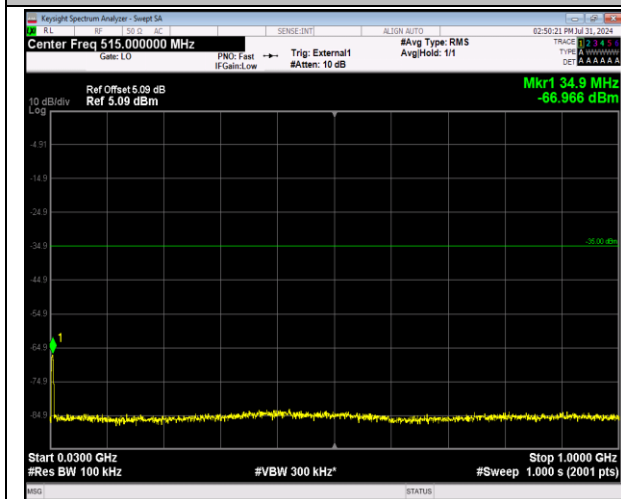
41-41-5MHz-20MHz-64QAM-64QAM-40648-40765-25R B#0-100RB#0-30~1000MHz-PASS
