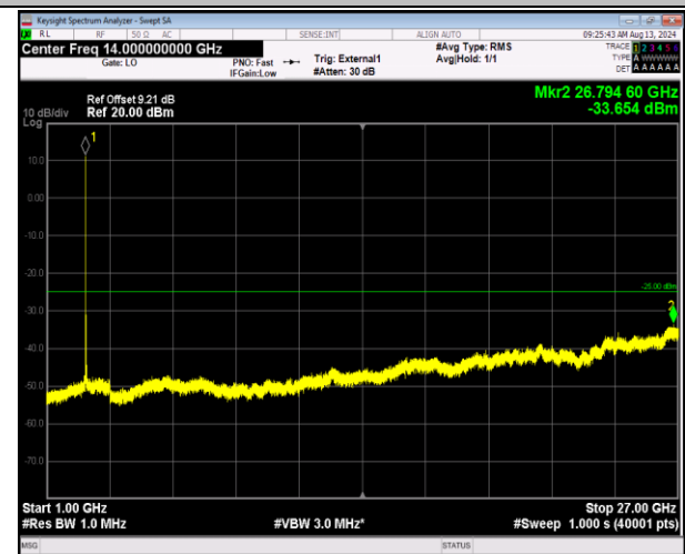
41-41-5MHz-20MHz-16QAM-16QAM-40648-40765-1RB# 0-1RB#99-1000~27000MHz-PASS
