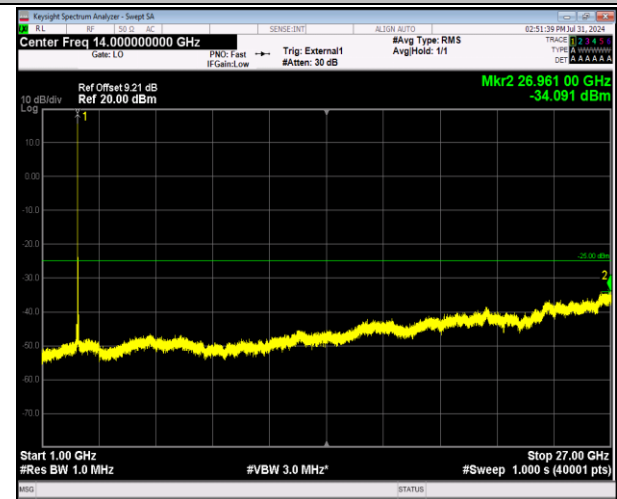
41-41-5MHz-20MHz-64QAM-64QAM-41023-41140-1RB# 0-ORB#0-1000~27000MHz-PASS
