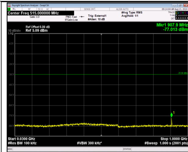
41-41-5MHz-20MHz-QPSK-QPSK-40273-40390-1RB#0-ORB#0-30~1000MHz-PASS
