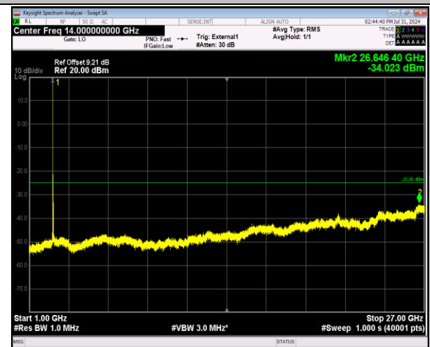
41-41-5MHz-20MHz-64QAM-64QAM-40273-40390-1RB# 0-ORB#0-1000~27000MHz-PASS
