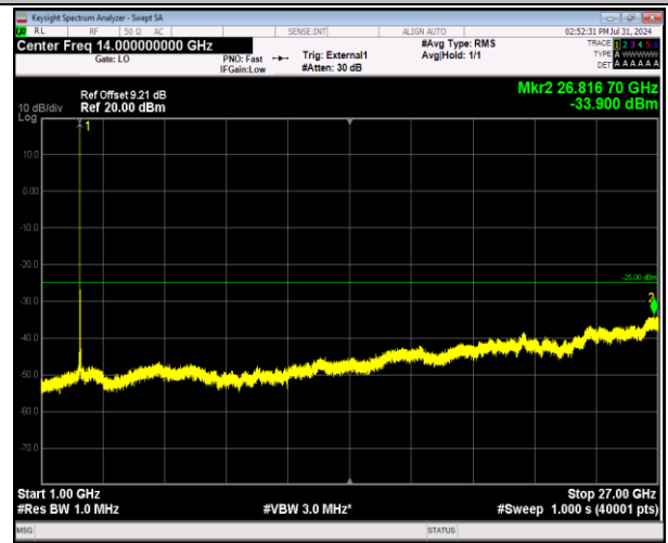
41-41-5MHz-20MHz-64QAM-64QAM-41023-41140-1RB# 24-0RB#0-1000~27000MHz-PASS
