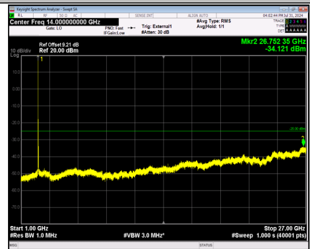
41-41-20MHz-5MHz-64QAM-64QAM-40340-40457-1RB# 0-0RB#0-1000~27000MHz-PASS
