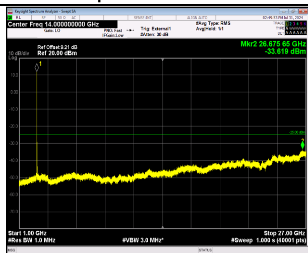
41-41-5MHz-20MHz-64QAM-64QAM-40648-40765-1RB# 0-1RB#99-1000~27000MHz-PASS
