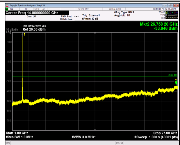
41-41-5MHz-20MHz-64QAM-64QAM-40648-40765-1RB# 0-ORB#0-1000~27000MHz-PASS
