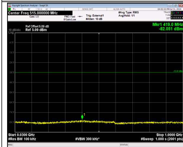
41-41-20MHz-5MHz-64QAM-64QAM-40340-40457-1RB #0-0RB#0-30~1000MHz-PASS
