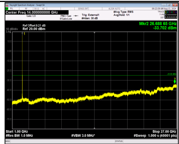
41-41-5MHz-20MHz-16QAM-16QAM-40648-40765-1RB# 24-ORB#0-1000~27000MHz-PASS
