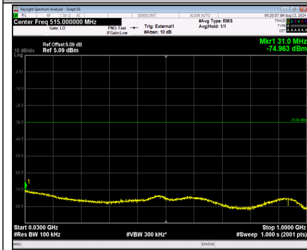
41-41-5MHz-20MHz-16QAM-16QAM-40273-40390-25R B#0-100RB#0-30~1000MHz-PASS
