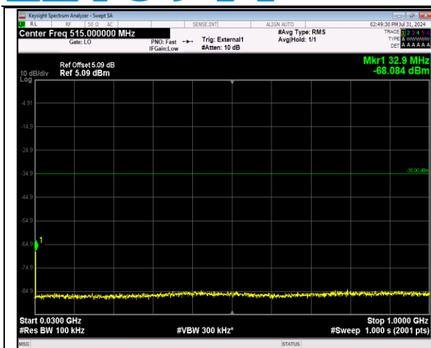
41-41-5MHz-20MHz-64QAM-64QAM-40648-40765-1RB #0-1RB#99-30~1000MHz-PASS
