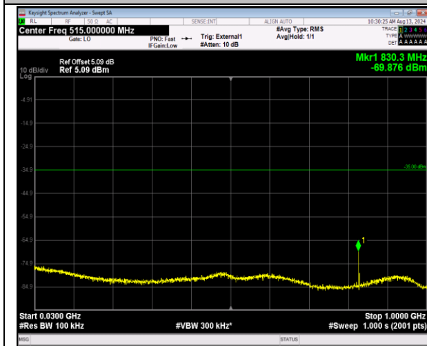
41-41-20MHz-5MHz-16QAM-16QAM-40340-40457-100 RB#0-25RB#0-30~1000MHz-PASS
