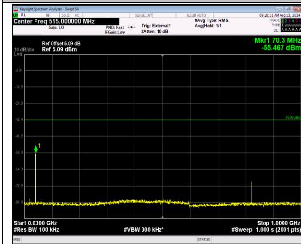
41-41-5MHz-20MHz-16QAM-16QAM-41023-41140-1RB #0-0RB#0-30~1000MHz-PASS
