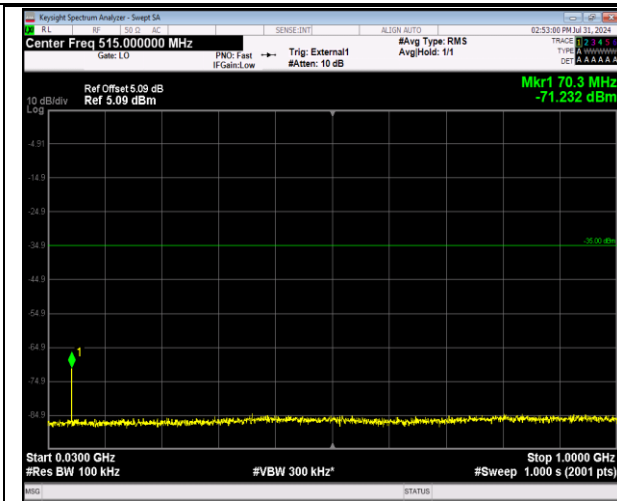
41-41-5MHz-20MHz-64QAM-64QAM-41023-41140-1RB #0-1RB#99-30~1000MHz-PASS
