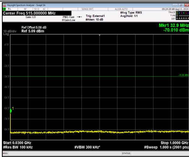
41-41-5MHz-20MHz-QPSK-QPSK-40648-40765-1RB#0-1RB#99-30~1000MHz-PASS
