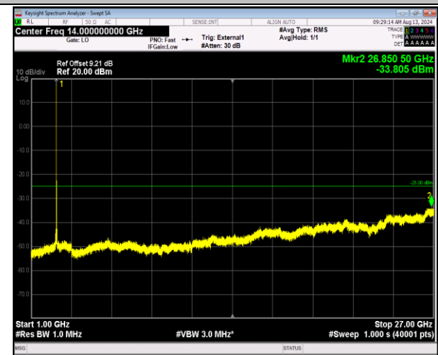
41-41-5MHz-20MHz-16QAM-16QAM-41023-41140-1RB# 0-0RB#0-1000~27000MHz-PASS
