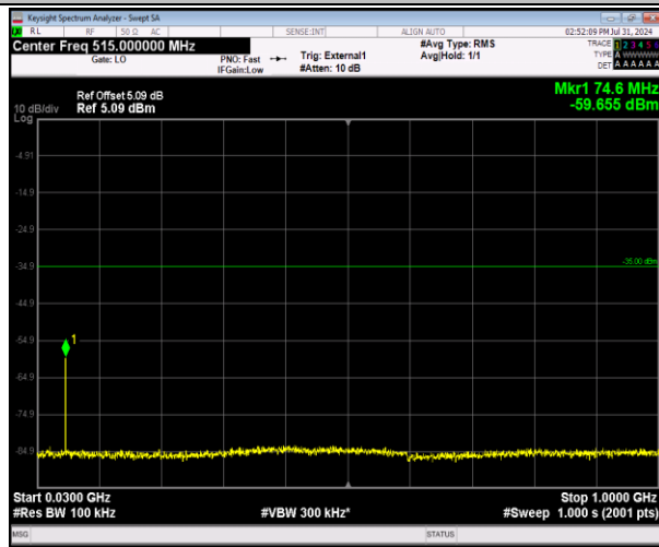
41-41-5MHz-20MHz-64QAM-64QAM-41023-41140-1RB #24-0RB#0-30~1000MHz-PASS
