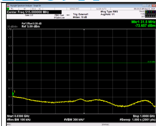
41-41-5MHz-20MHz-QPSK-QPSK-40273-40390-25RB# 0-100RB#0-30~1000MHz-PASS
