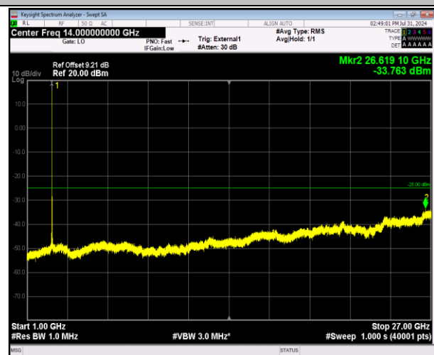
41-41-5MHz-20MHz-64QAM-64QAM-40648-40765-1RB# 24-0RB#0-1000~27000MHz-PASS
