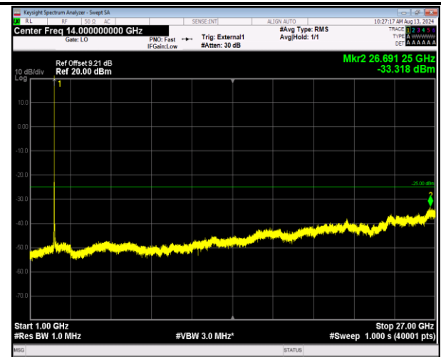
41-41-20MHz-5MHz-16QAM-16QAM-40340-40457-1RB# 99-ORB#0-1000~27000MHz-PASS
