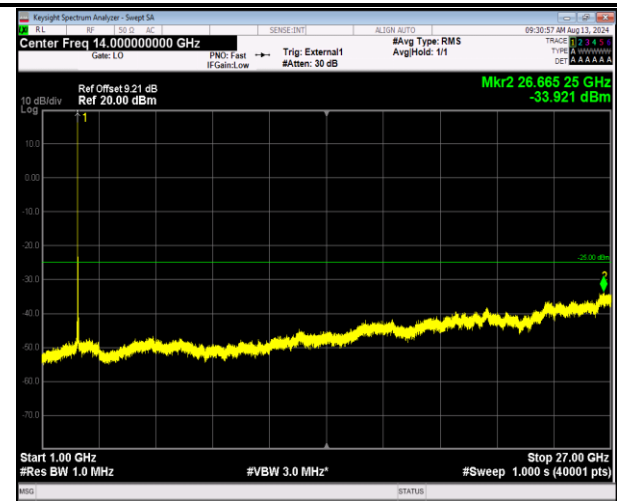
41-41-5MHz-20MHz-16QAM-16QAM-41023-41140-1RB# 24-ORB#0-1000~27000MHz-PASS
