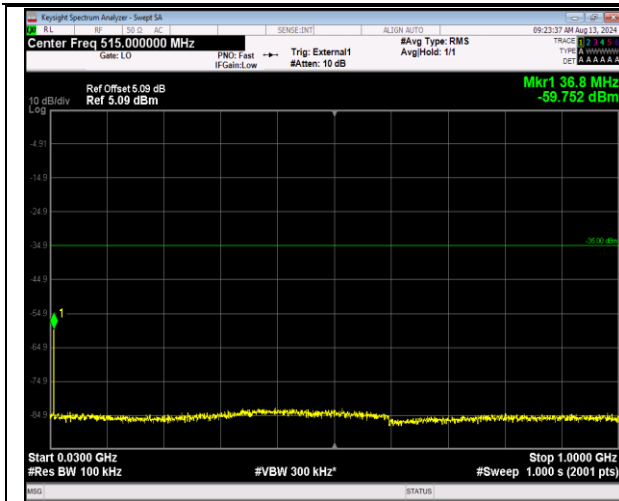
41-41-5MHz-20MHz-16QAM-16QAM-40648-40765-1RB #24-ORB#0-30~1000MHz-PASS
