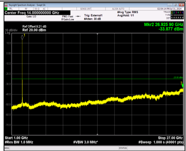
41-41-5MHz-20MHz-64QAM-64QAM-41023-41140-25RB #0-100RB#0-1000~27000MHz-PASS
