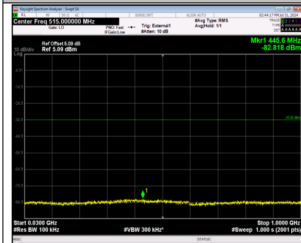
41-41-5MHz-20MHz-64QAM-64QAM-40273-40390-1RB #0-ORB#0-30~1000MHz-PASS
