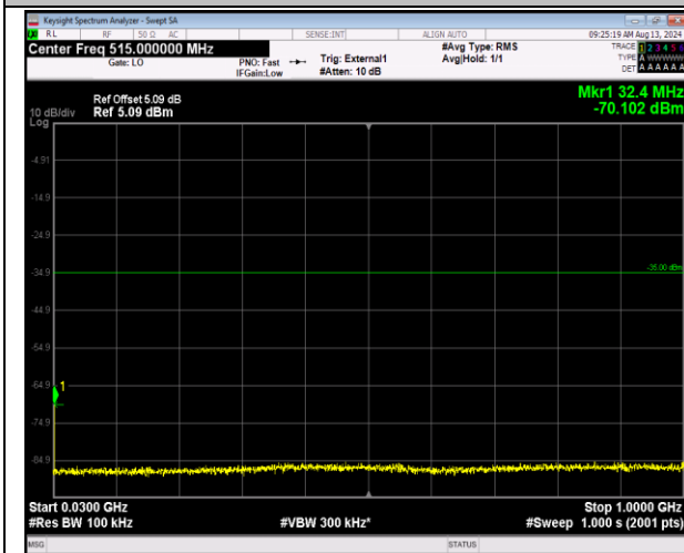
41-41-5MHz-20MHz-16QAM-16QAM-40648-40765-1RB #0-1RB#99-30~1000MHz-PASS
