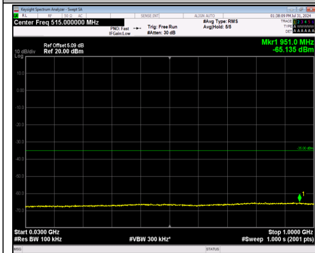
7-7-20MHz-20MHz-64QAM-64QAM-21152-21350-100R B#0-100RB#0-30~1000MHz-PASS
