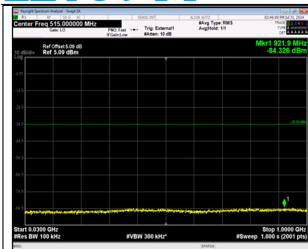
41-41-5MHz-20MHz-64QAM-64QAM-40273-40390-1RB #0-1RB#99-30~1000MHz-PASS
