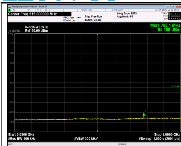
7-7-20MHz-20MHz-64QAM-64QAM-21152-21350-1RB# 0-1RB#99-30~1000MHz-PASS
