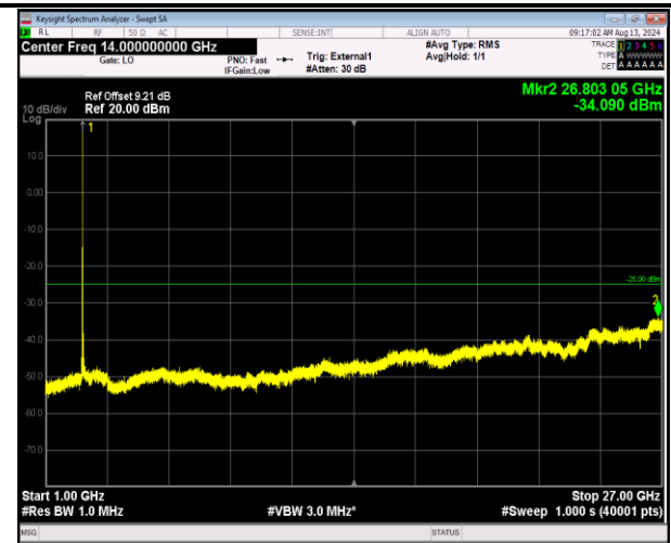
41-41-5MHz-20MHz-16QAM-16QAM-40273-40390-1RB# 24-ORB#0-1000~27000MHz-PASS
