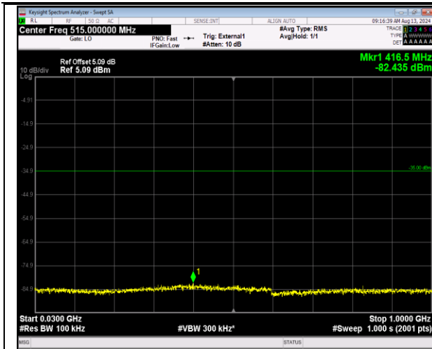
41-41-5MHz-20MHz-16QAM-16QAM-40273-40390-1RB #24-ORB#0-30~1000MHz-PASS
