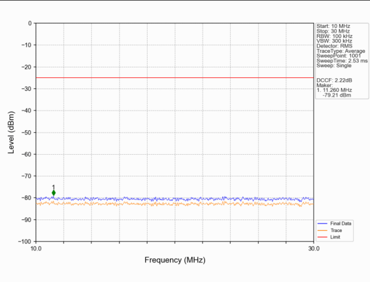
Band41_5MHz_16QAM_HCH_2652.5MHz_RB_1_0_NTNV
