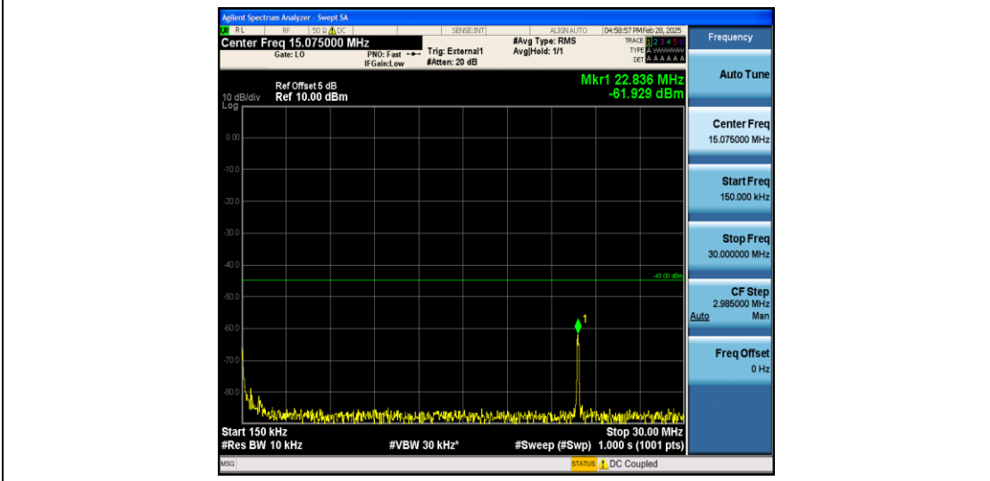
Band41_20MHz_16QAM_40620_1RB#0_0.15~30_0.15~30
