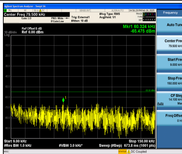
Band41_20MHz_16QAM_39750_1RB#0_0.009~0.15_0.009~0.15
