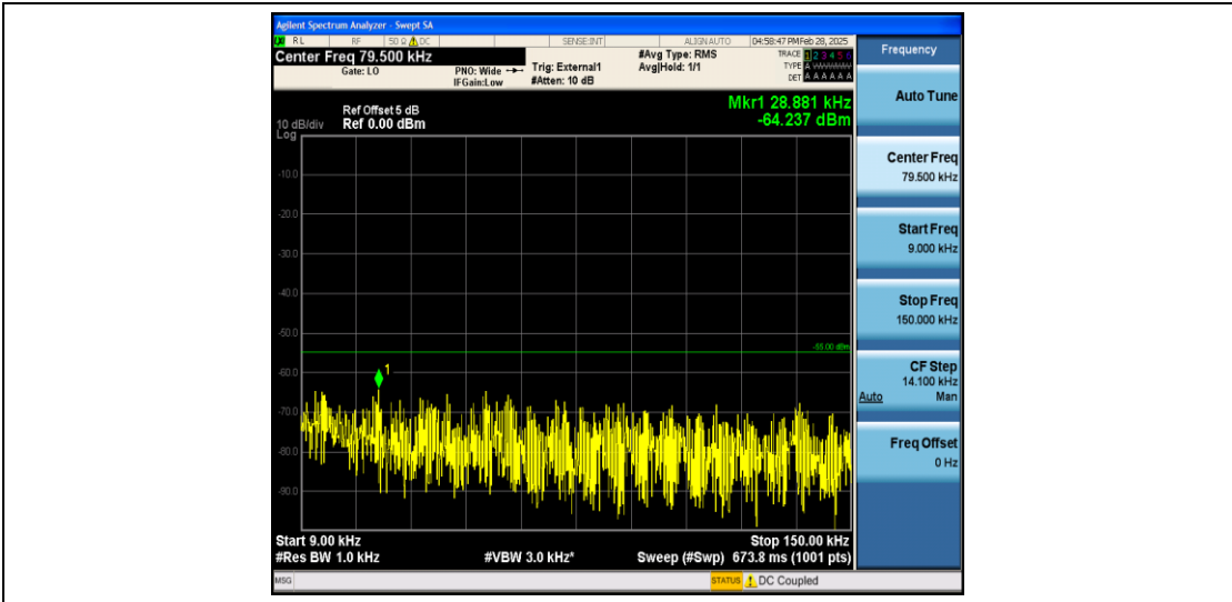
Band41_20MHz_16QAM_40620_1RB#0_0.009~0.15_0.009~0.15
