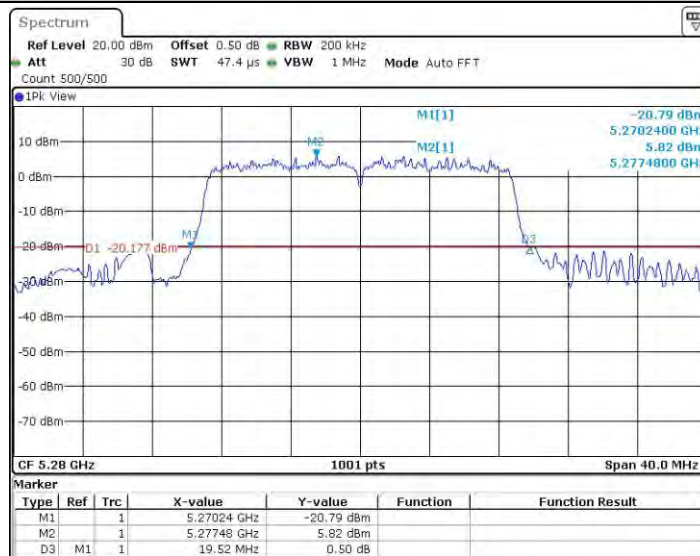
11AC20SISO_Ant0_5280
