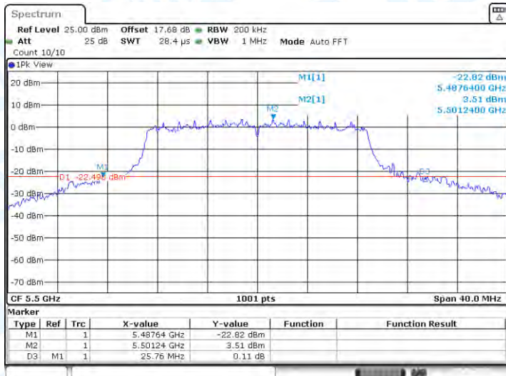
11AC20-CDD-Ant1-5500
