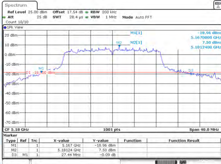
11N20-CDD-Ant1-5180
