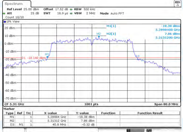
11N40-CDD-Ant2-5310
