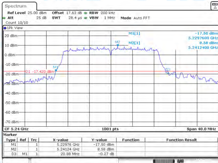
11AC20-CDD-Ant1-5240
