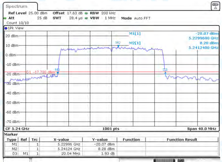
11AX20-CDD-Ant1-5240
