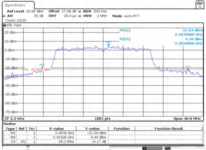
11AX20-CDD-Ant1-5500
