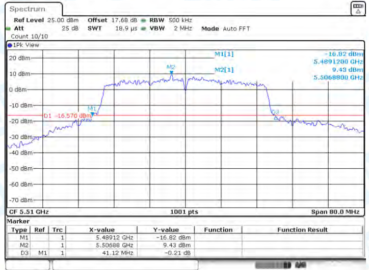
11AC40-CDD-Ant1-5510
