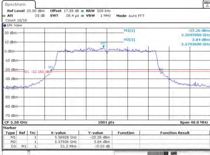
11AX20-CDD-Ant1-5580
