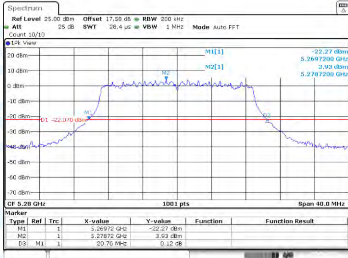
11AC20-CDD-Ant1-5280
