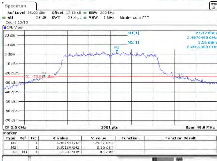
11N20-CDD-Ant1-5500
