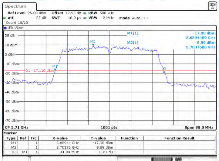
11N40-CDD-Ant1-5710
