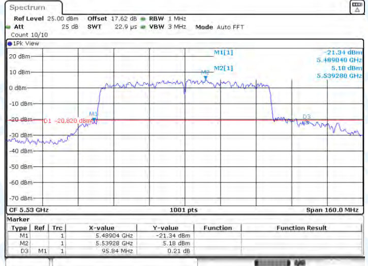
11AC80-CDD-Ant2-5530
