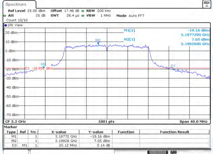
11A-CDD-Ant2-5200
