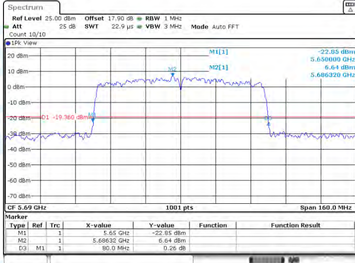
11AC80-CDD-Ant1-5690
