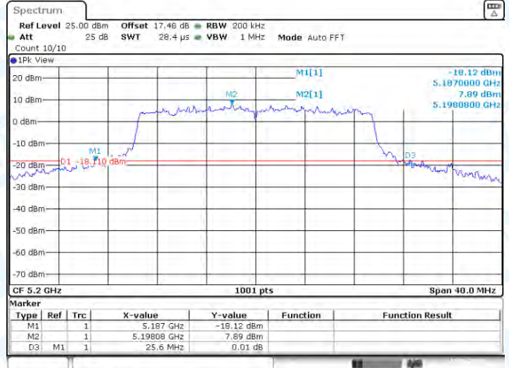
11AX20-CDD-Ant2-5200
