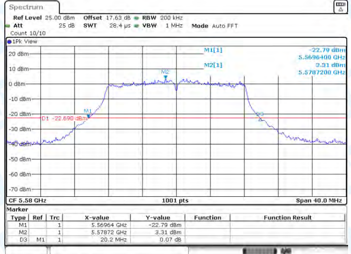
11A-CDD-Ant2-5580
