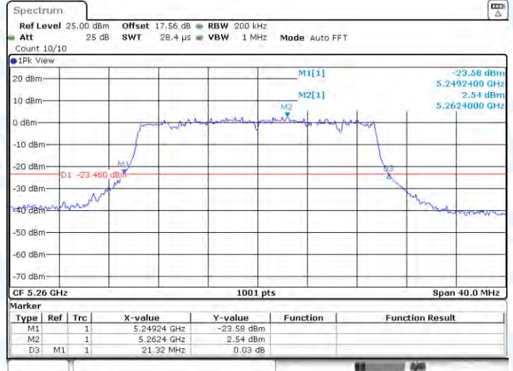
11AX20-CDD-Ant2-5260
