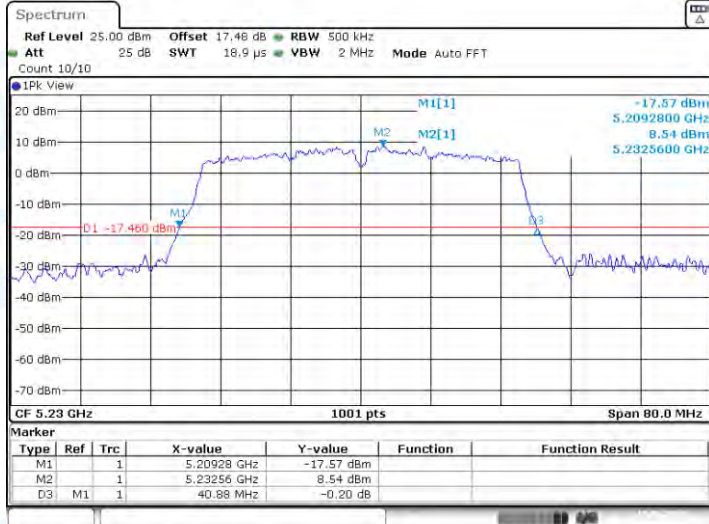
11AC40-CDD-Ant1-5230
