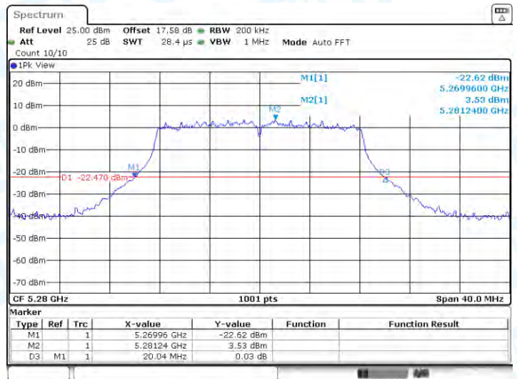
11A-CDD-Ant1-5280
