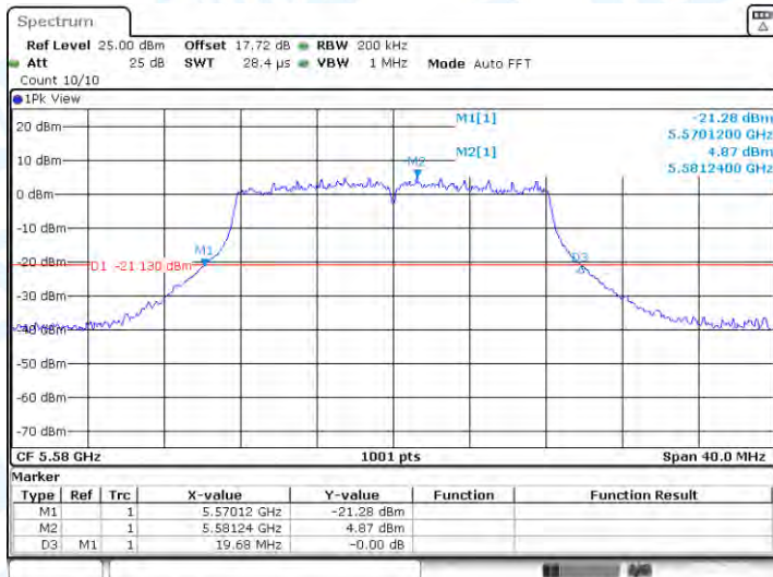
11A-CDD-Ant1-5580
