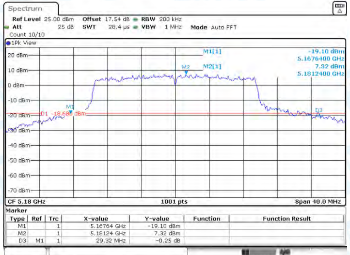
11AX20-CDD-Ant1-5180
