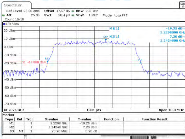
11N20-CDD-Ant2-5240
