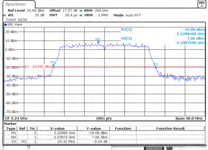
11AC20-CDD-Ant2-5240
