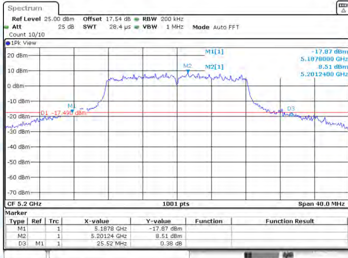
11A-CDD-Ant1-5200
