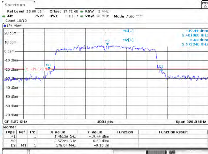
11AC160-CDD-Ant1-5570
