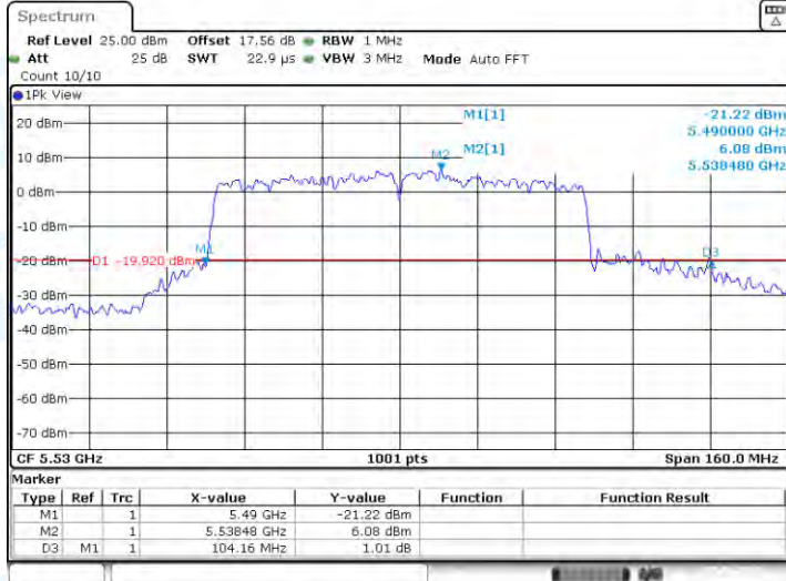
11AC80-CDD-Ant1-5530
