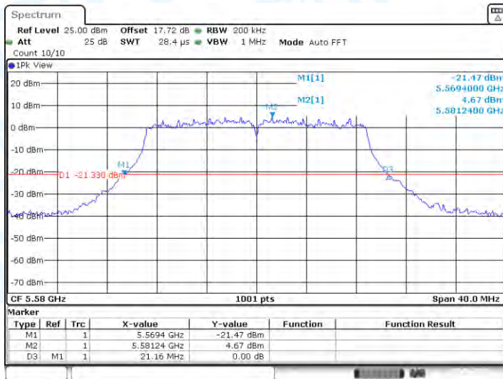
11N20-CDD-Ant1-5580
