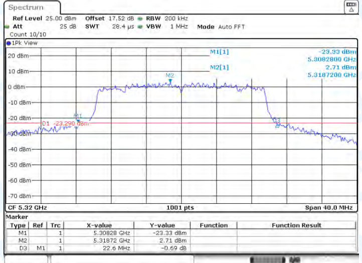
11AX20-CDD-Ant2-5320
