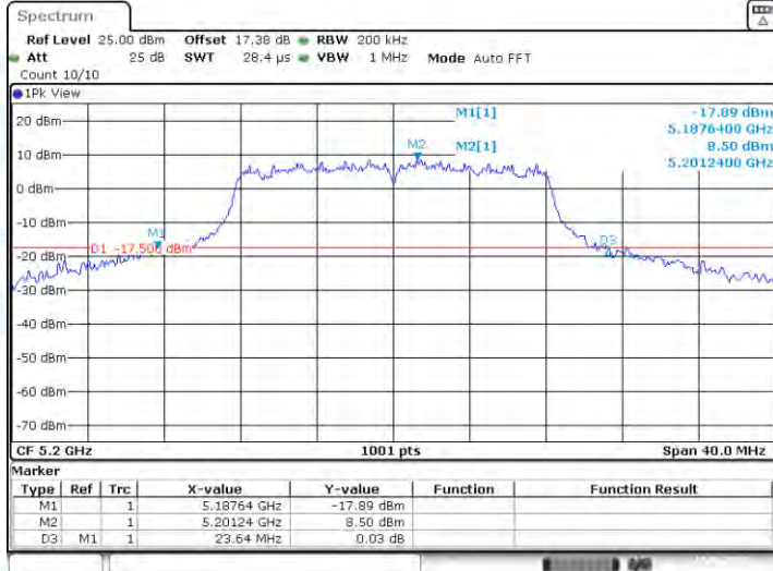
11A-CDD-Ant1-5200
