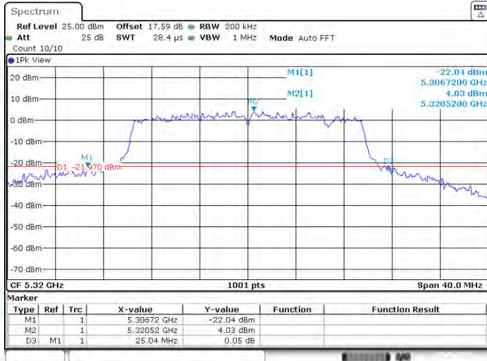
11AX20-CDD-Ant1-5320
