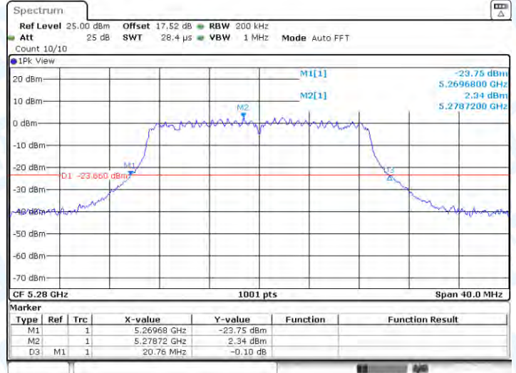
11AC20-CDD-Ant2-5280
