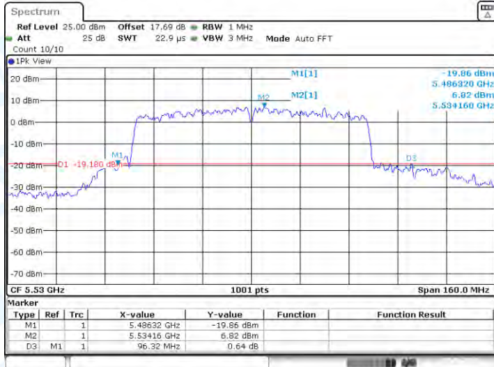
11AC80-CDD-Ant1-5530
