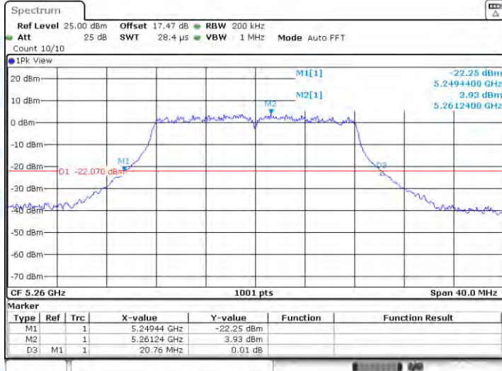
11A-CDD-Ant1-5260
