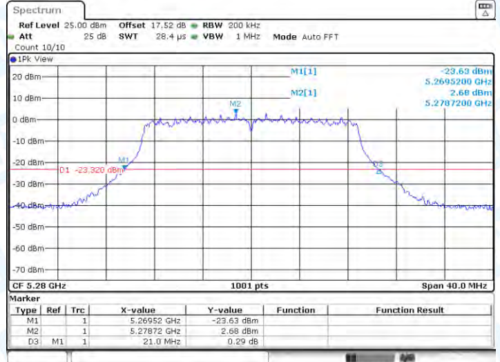
11N20-CDD-Ant2-5280
