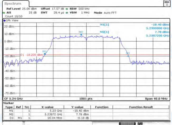
11A-Ant2-5240
