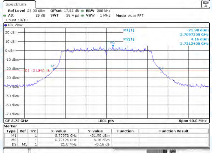
11N20-CDD-Ant2-5720
