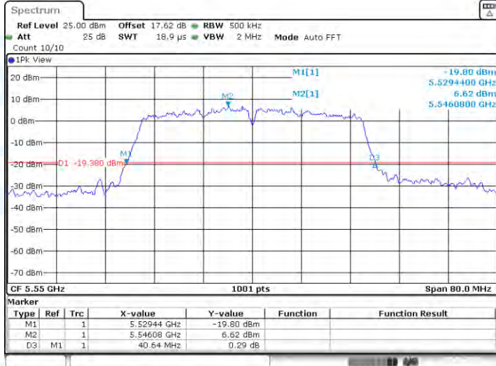
11AC40-CDD-Ant1-5550
