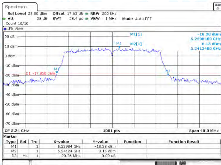
11N20-CDD-Ant1-5240
