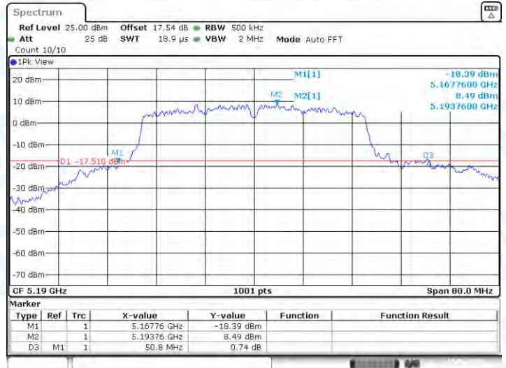
11AC40-CDD-Ant1-5190
