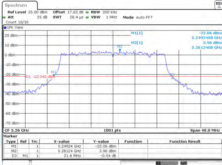
11AX20-CDD-Ant1-5260
