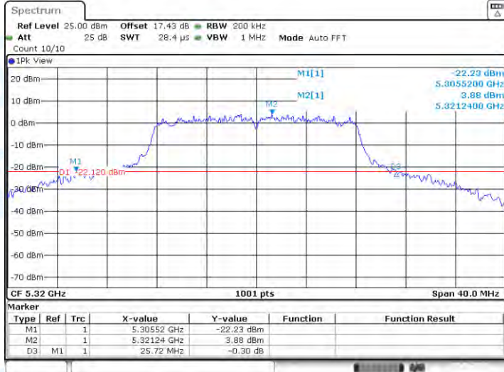
11A-CDD-Ant1-5320
