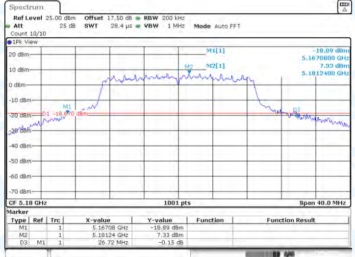
11N20-CDD-Ant2-5180
