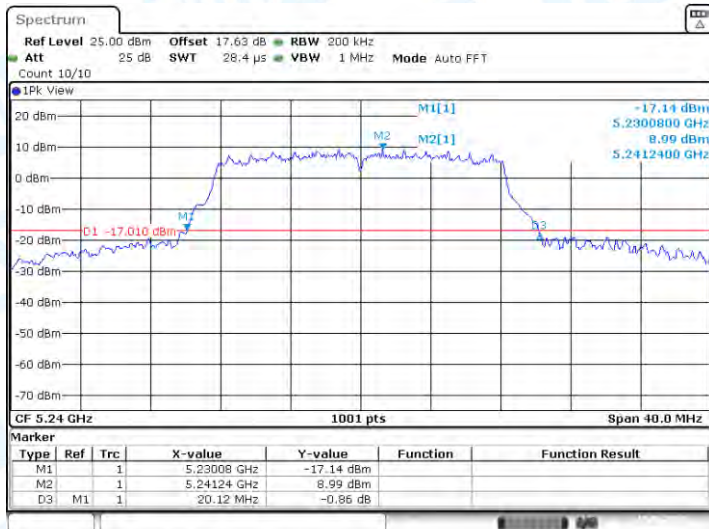
11A-Ant1-5240
