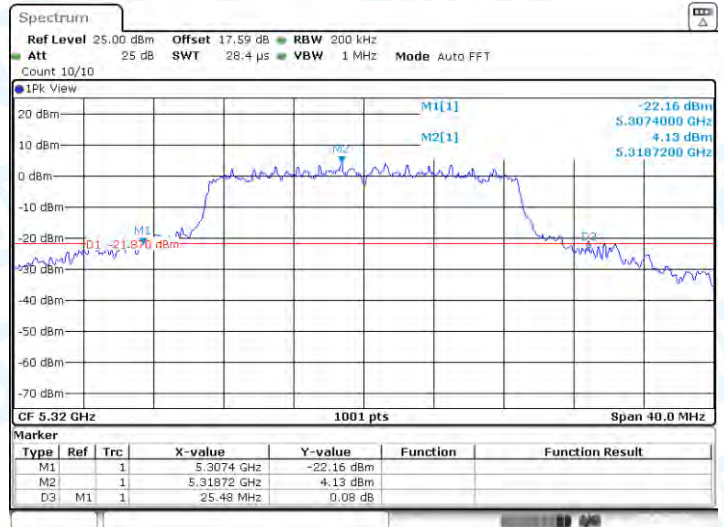
11AC20-CDD-Ant1-5320
