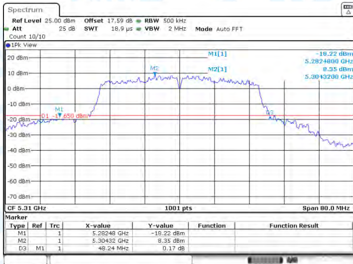
11AC40-CDD-Ant1-5310
