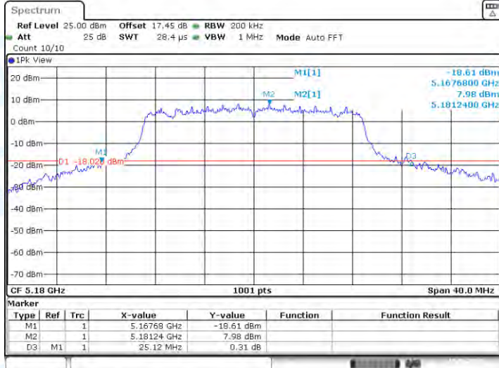
11AC20-CDD-Ant1-5180
