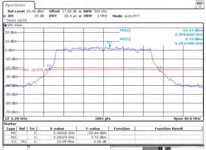
11AX20-CDD-Ant1-5280
