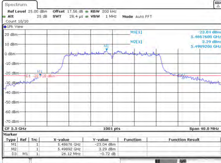
11AC20-CDD-Ant1-5500
