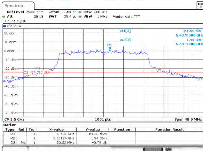
11N20-CDD-Ant2-5500
