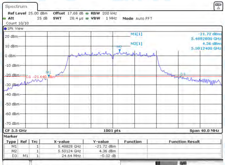
11A-CDD-Ant1-5500
