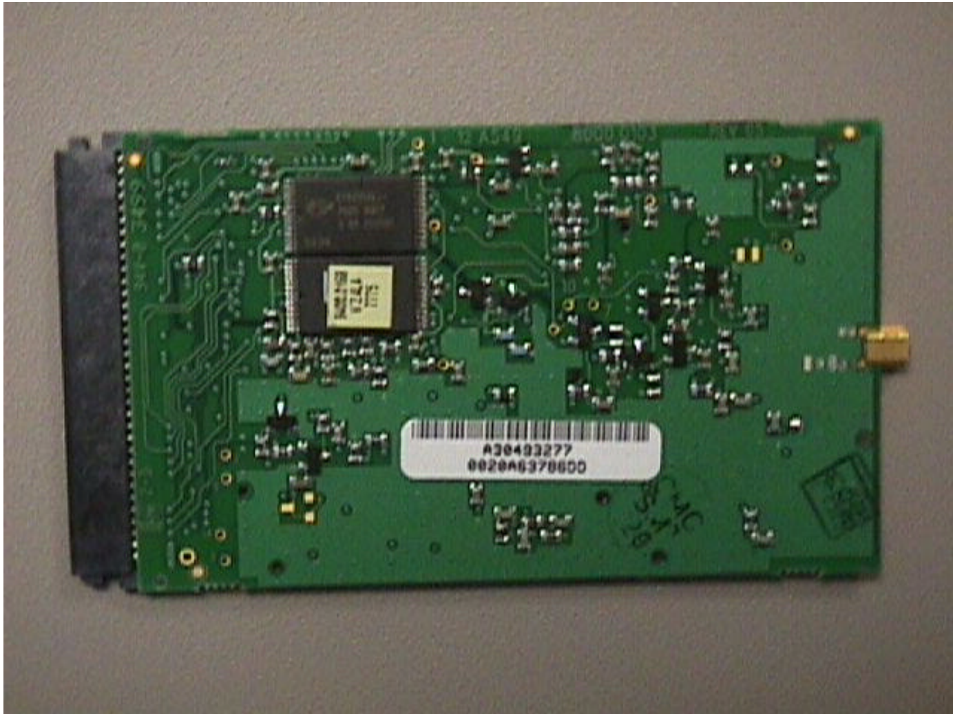
Radio board (bottom view)
