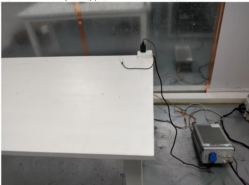
Test Setup Photo(s) of Conducted Emissions Measurement
