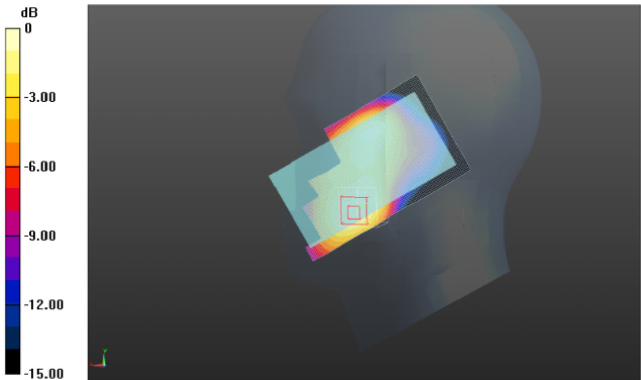
Left Head Cheek (LTE Band IV Middle Channel)
