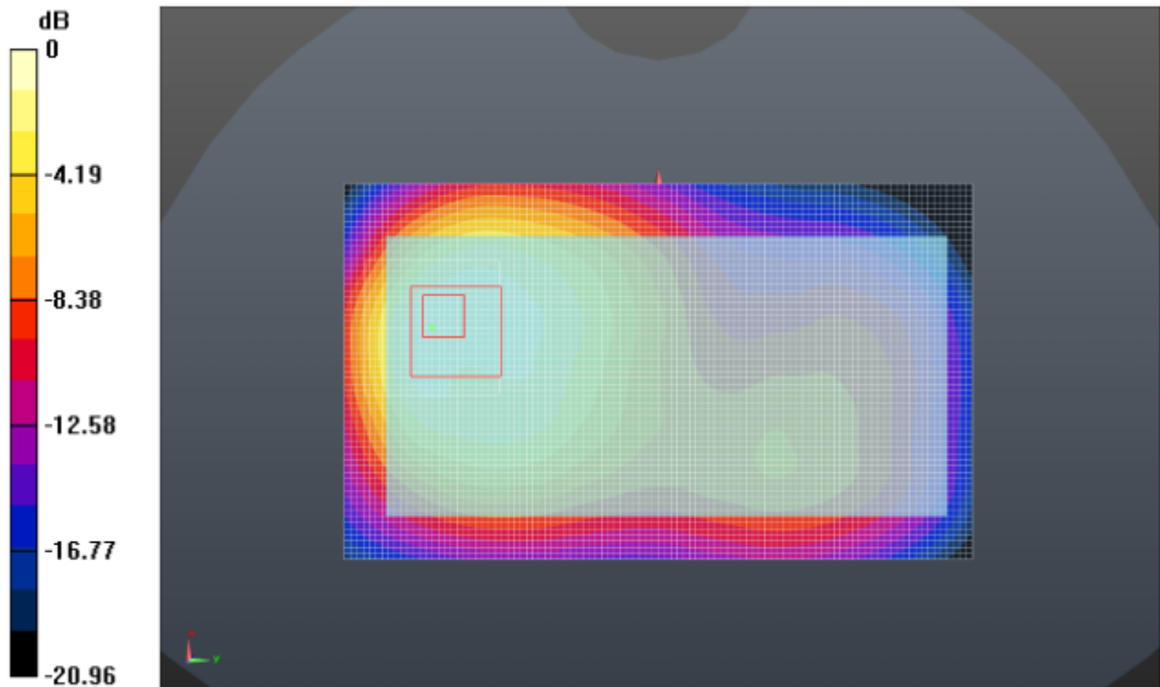
Body- worn Rear Side (LTE Band IV Middle Channel)
