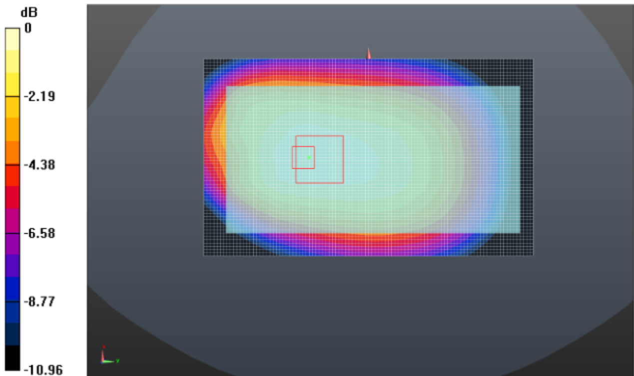
Body- worn Rear Side (LTE Band V Middle Channel)
