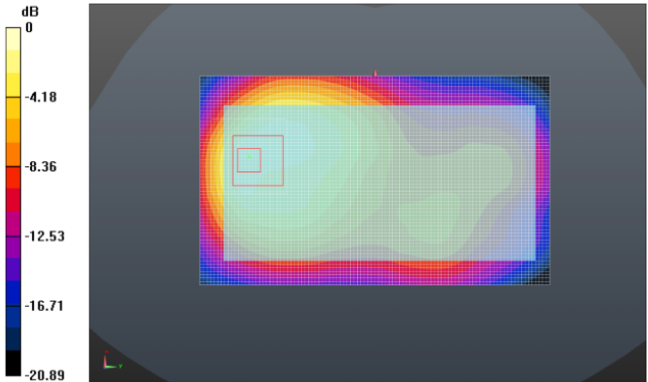
Body- worn Rear Side (WCDMA Band II Middle Channel)
