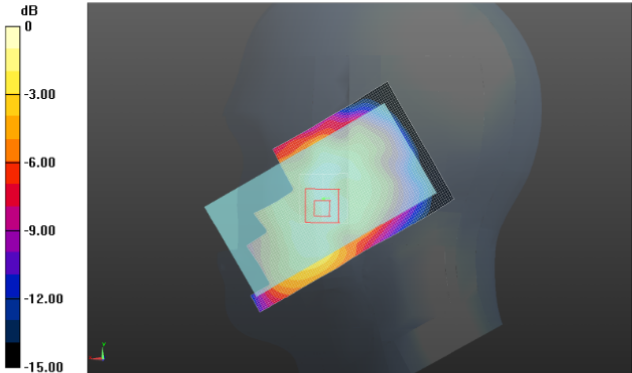
Left Head Cheek (LTE Band V Middle Channel)
