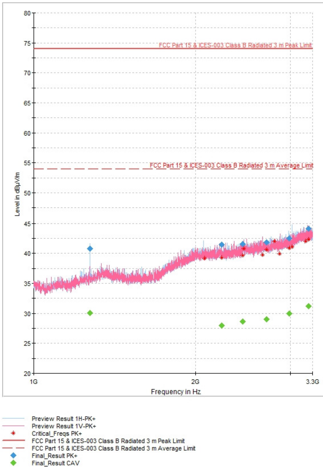
Figure 2.2.9-2 – Radiated Emissions Plot 1 – 3.3 GHz
