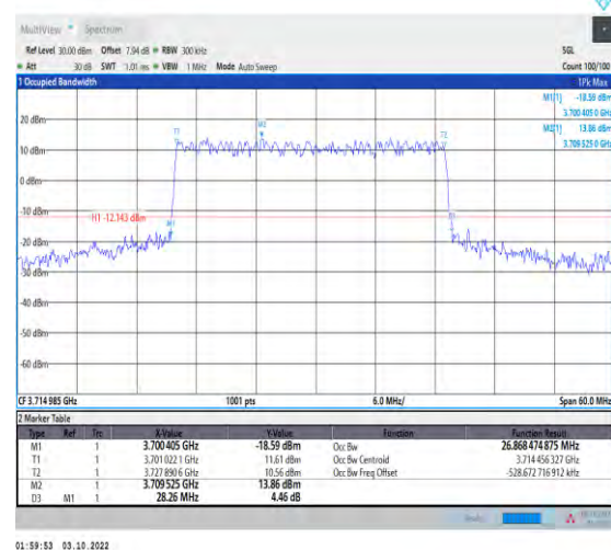
1-N78-3700-3800-PASS-30-30-L-1-DFT-QPSK-Outer _Full-75@0-Ant1-26.868-28.260-≤30-PASS
