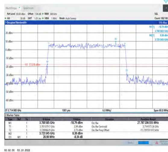
1-N78-3700-3800-PASS-30-30-L-9-CP-256QAM-Outer_Full-78@0-Ant1-27.787-28.980-≤30-PASS
