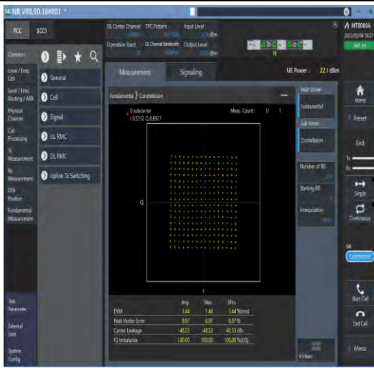
1-N78-3700-3800--30-100-M-5-DFT-256QAM-Outer_Fu Full-270@0-Ant1-see graph-PASS
