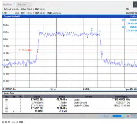
1-N78-3700-3800-PASS-30-20-L-5-DFT-256QAM-Outer_Full-50@0-Ant1-17.844-18.800-≤20-PASS
