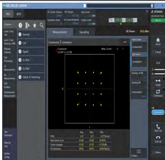
1-N78-3700-3800--30-100-M-3-DFT-16QAM-Outter_Full-270@0-Ant1-see graph-PASS
