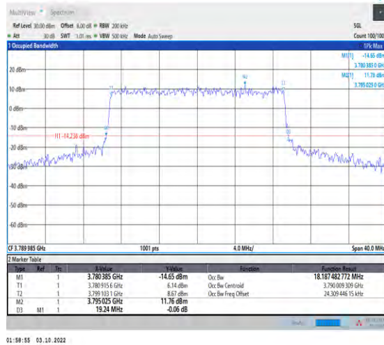
1-N78-3700-3800-PASS-30-20-H-7-CP-16QAM-Out er_Full-51@0-Ant1-18.187-19.240-≤20-PASS
