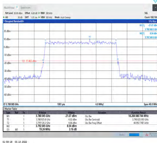
1-N78-3700-3800-PASS-30-20-H-9-CP-256QAM-Out ter_Full-51@0-Ant1-18.2-19.240-≤20-PASS
