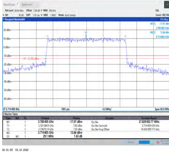
1-N78-3700-3800-PASS-30-30-L-6-CP-QPSK-Outer_Full-78@0-Ant1-27.829-29.100-≤30-PASS
