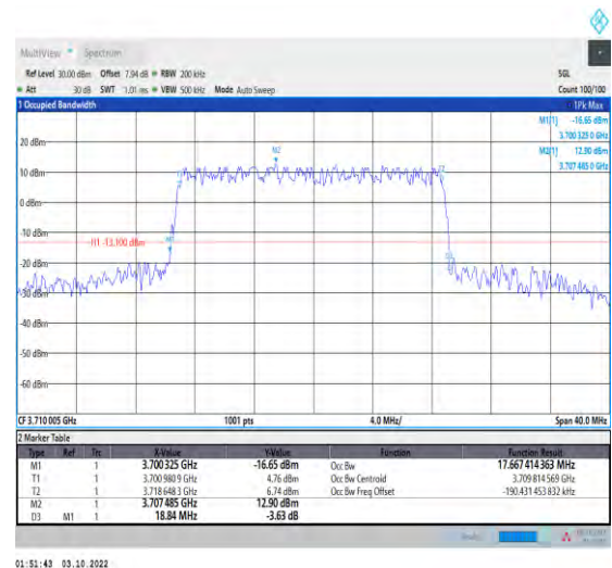
1-N78-3700-3800-PASS-30-20-L-4-DFT-64QAM-Outer_Full-50@0-Ant1-17.667-18.840-≤20-PASS
