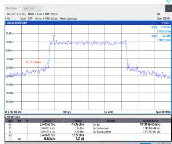
1-N78-3700-3800-PASS-30-20-M-7-CP-16QAM-Outer_Full-51@0-Ant1-18.192-18.880-≤20-PASS
