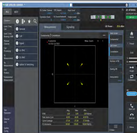
1-N78-3700-3800--30-100-M-2-DFT-QPSK-Outter_Full-270@0-Ant1-see graph-PASS
