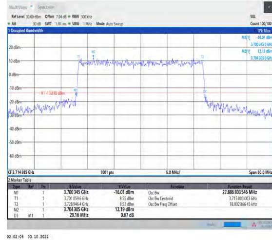
1-N78-3700-3800-PASS-30-30-L-7-CP-16QAM-Outer_Full-78@0-Ant1-27.887-29.160-≤30-PASS
