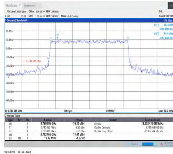
1-N78-3700-3800-PASS-30-20-H-8-CP-64QAM-Out r_Full-51@0-Ant1-18.252-19.320-≤20-PASS
