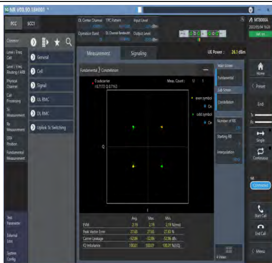
1-N78-3700-3800--30-100-M-1-DFT-PI2BPSK-Outter_Full-270@0-Ant1-see graph-PASS
