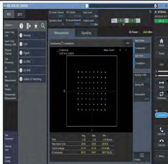
1-N78-3700-3800--30-100-M-4-DFT-64QAM-Outter_Full-270@0-Ant1-see graph-PASS
