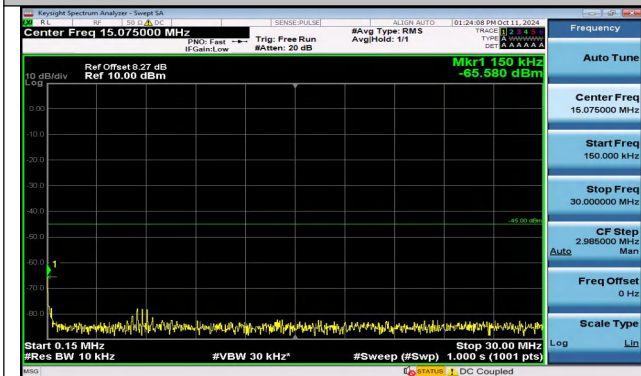
Band41_20MHz_16QAM_41140_1RB#99_0.15~30_0.15~ 30
