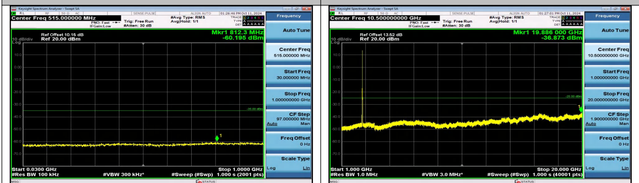
Band41_20MHz_QPSK_41140_100RB#0_30~1000_30~1000
