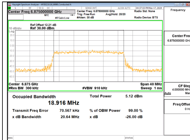
H STRADDLE Antenna 1
