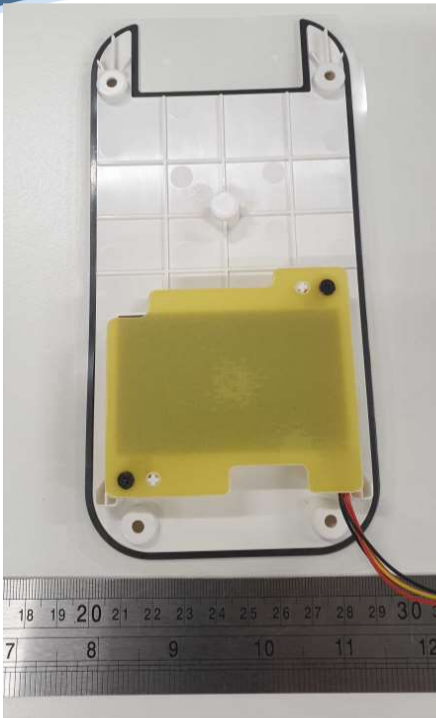
Receiver Back Plate and Antenna
