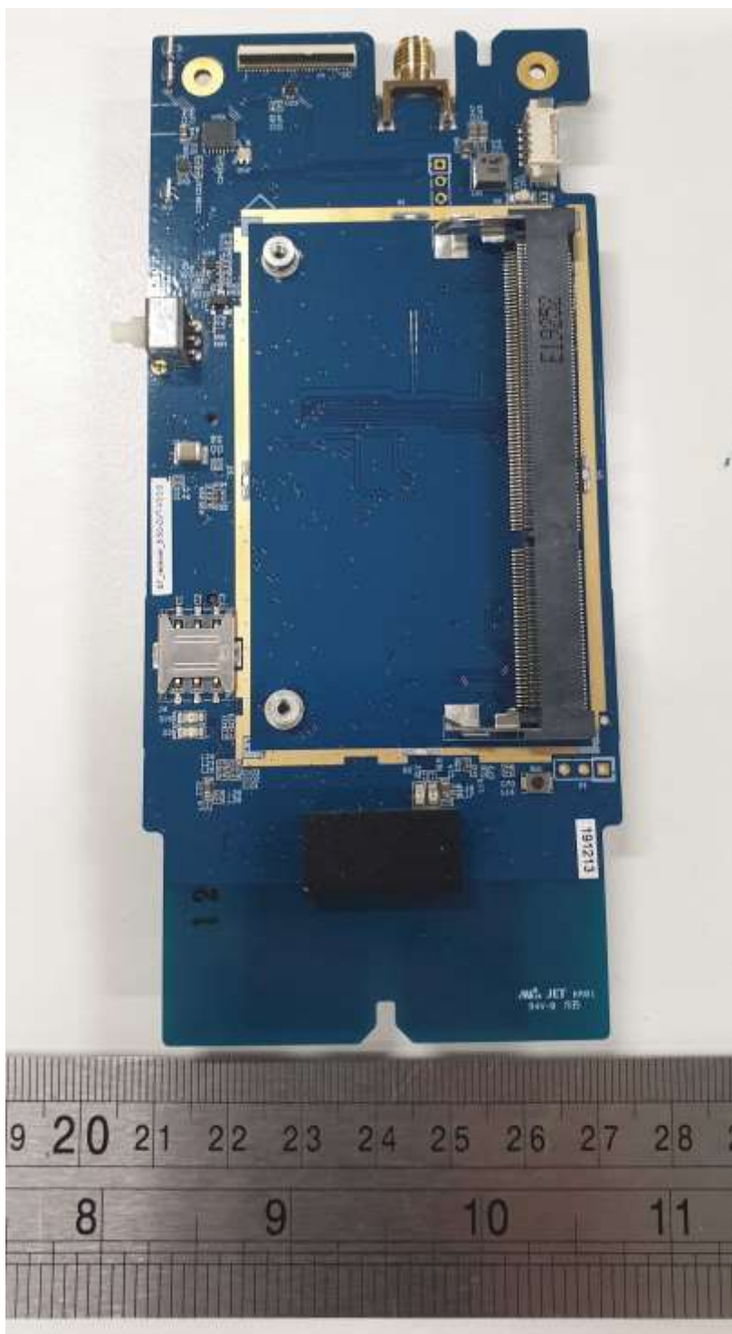
Main Board Back, Module Removed
