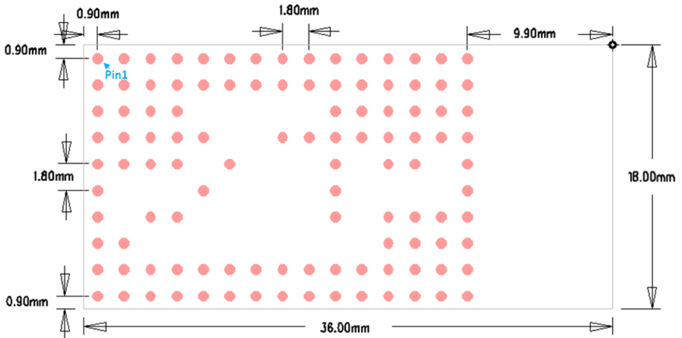
TOP VIEW (Bottom Pads)
