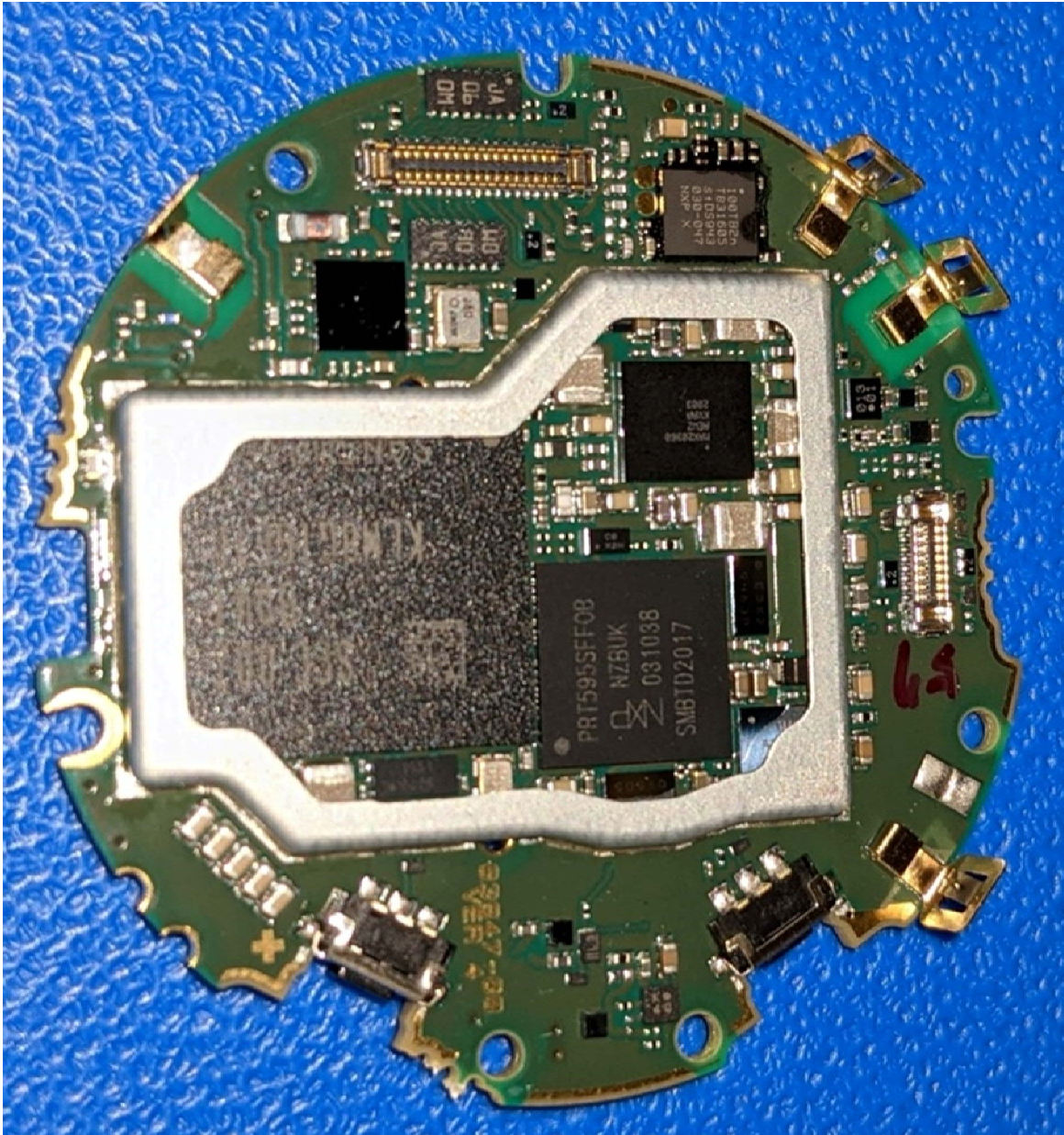
Figure E19.3 – Internal Photo – PCB Top, Shield Removed
