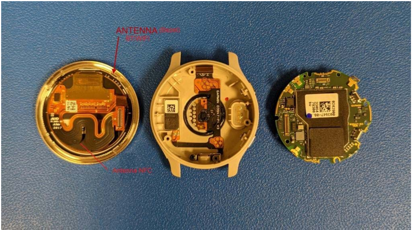
Figure E19.4 – Internal Photo – Antennas
