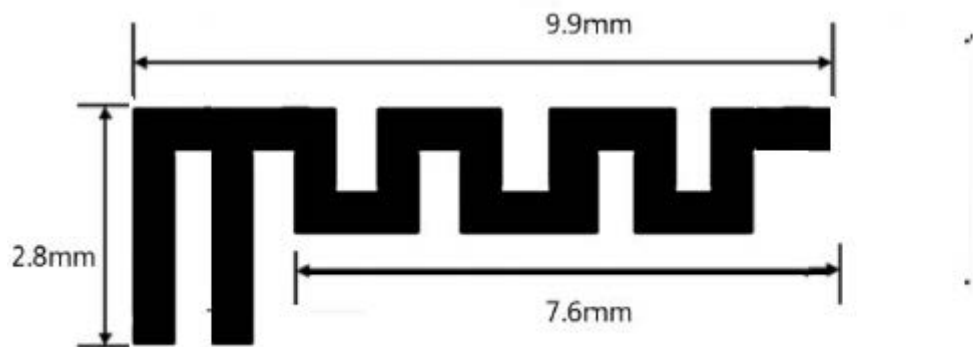
Antenna Dimensions
