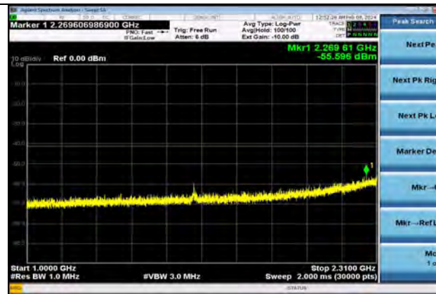
802.11b | Channel 6 | 1 Mbps | 1000-2310 MHz
