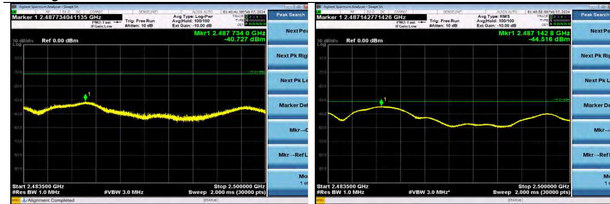
802.11b | Channel 11 | 1 Mbps | Peak
