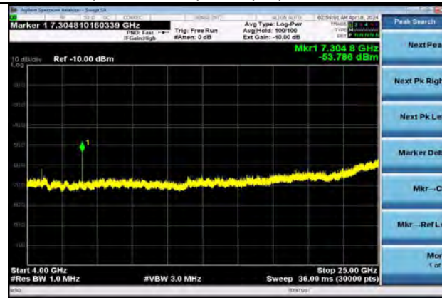
802.11ax20 | Channel 6 | MCS0 | RU26 | 4000-25000 MHz
