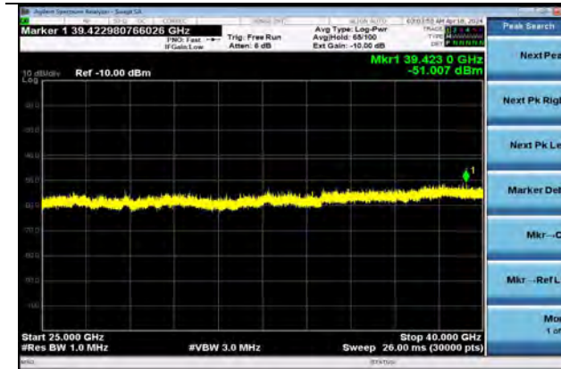
802.11ax20 | Channel 6 | MCS0 | RU26 | 25000-40000 MHz
