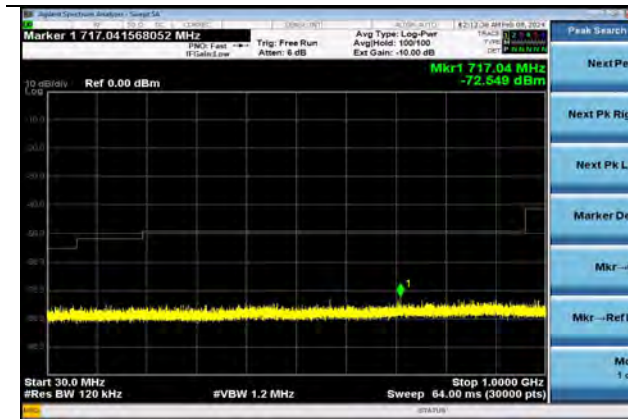
802.11b | Channel 6 | 1 Mbps | 30-1000 MHz
