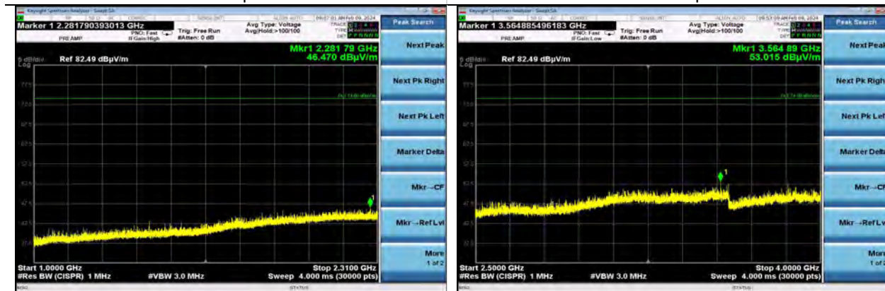
802.11ax40 | Channel 3 | MCS11 | RU38 1000-2310 MHz | Vertical
