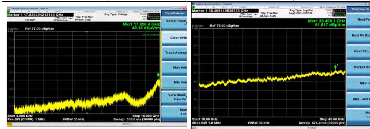
802.11ax20 | Channel 6 | MCS0 4000-18000 MHz | Vertical
