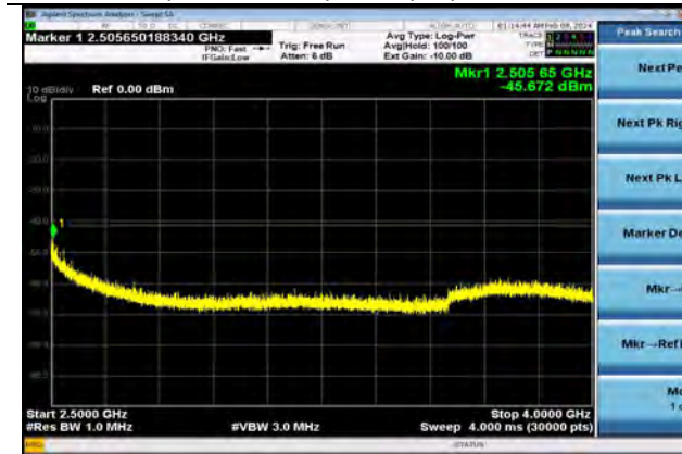
802.11n40 | Channel 6 | MCS0 | 2500-4000 MHz
