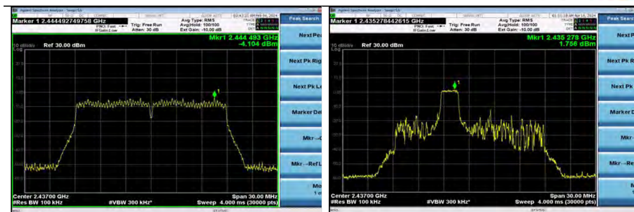
802.11n20 | Channel 6 | MCS7
