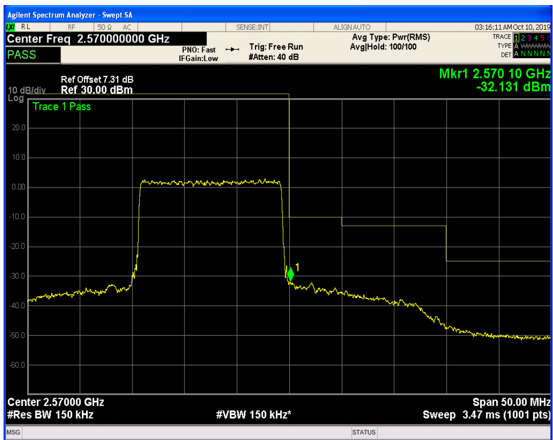
LTE Band7 QAM16 BW=15MHz Channel=21375 RB Size=1 Position=#Max
