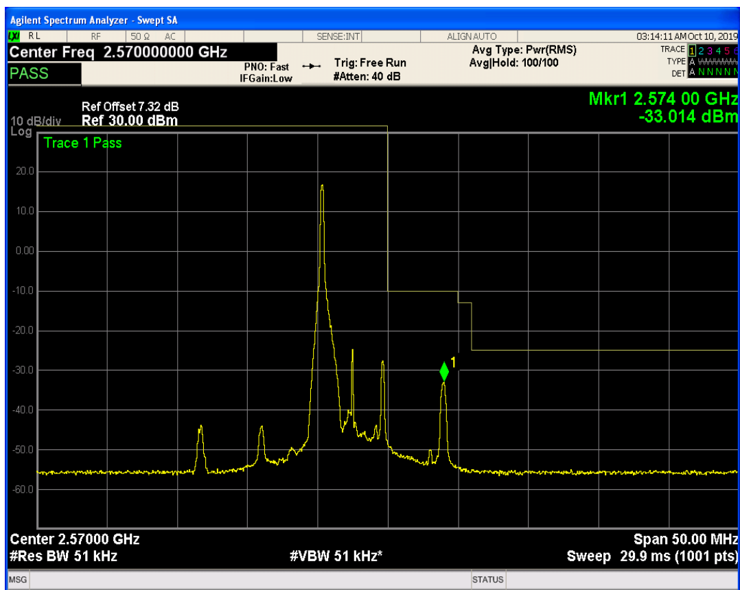
LTE Band7 QAM16 BW=5MHz Channel=21425 RB Size=1 Position=#Max
