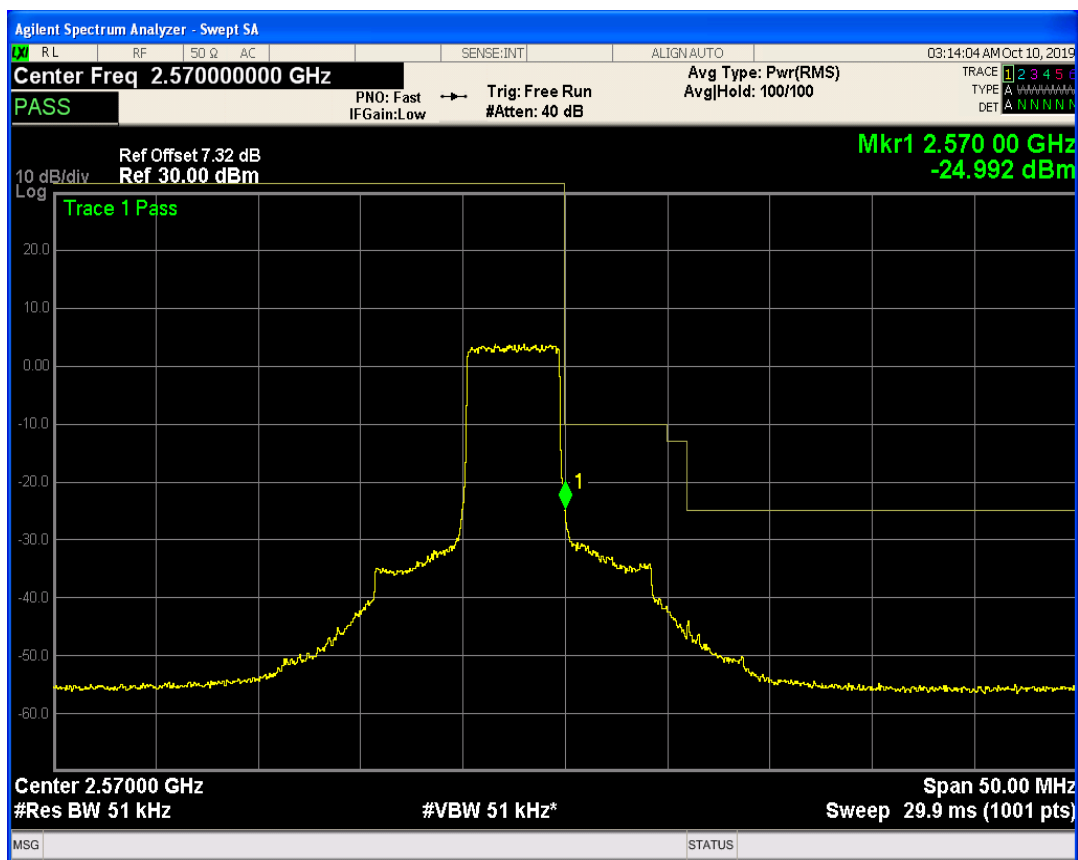
LTE Band7 QPSK BW=5MHz Channel=21425 RB Size=1 Position=#Max
