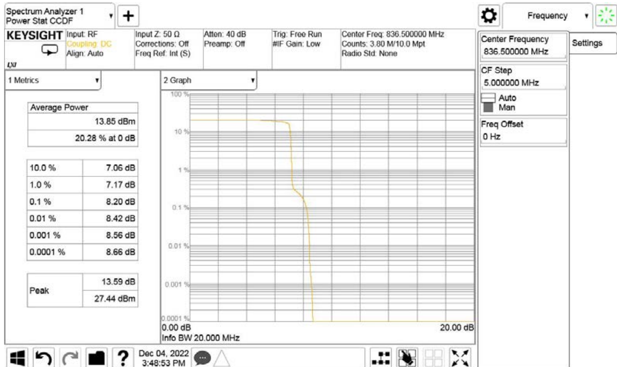
Band26-CH26915-836.5MHz-QPSK
